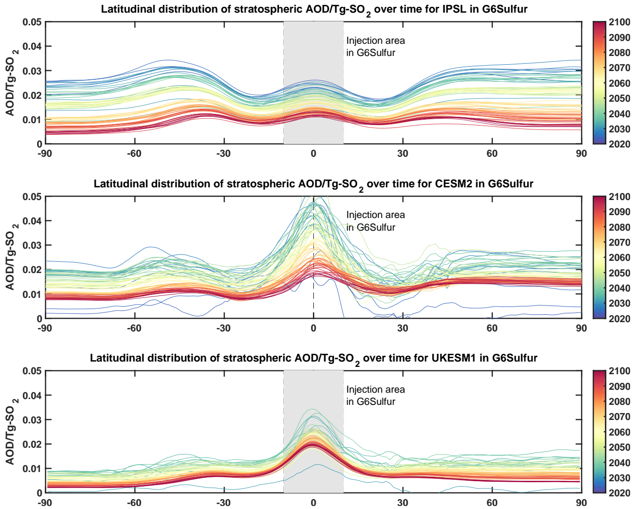
Fig. S1 Latitudinal distribution of yearly-averaged AOD normalized by amount of SO 2 injected in that year. The color scale indicate the year of analyses.
