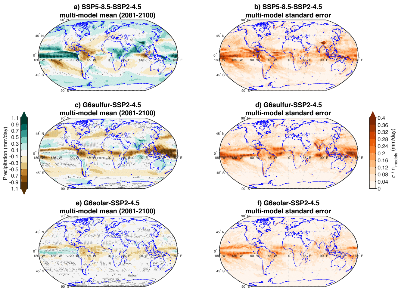
Figure 9. Left column: multi-model averages for precipitation changes averaged over 2081-2100 in different cases (a) SSP5-8.5; c) G6sulfur; e) G6solar) minus the same period for SSP2-4.5. Etched areas (in grey) indicate where less than 66% of models (here, 4 out of 6) agree on the sign of the difference in that grid-point. Right column: Standard error in the multi-model mean for the same reference case on the left. All models results have been re-gridded using a common grid equivalent to that from the model with the lowest horizontal resolution.
