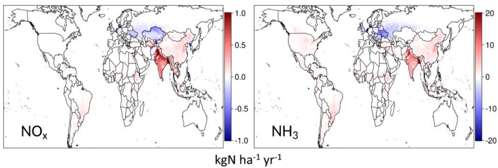
860 Figure 4. Changes in agricultural NH 3 and NO x emissions (2014 – 1992) as implemented by the Community Emissions Data System (CEDs).
