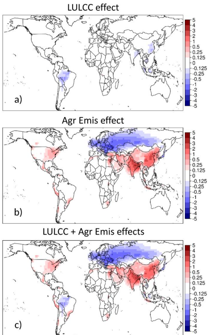
Figure 5. Simulated changes in annual mean surface PM 2.5 due to (a) LULCC, (b) agricultural emission (“Agr Emis”) changes, and (c) the combined effects of agricultural emissions and LULCC.
