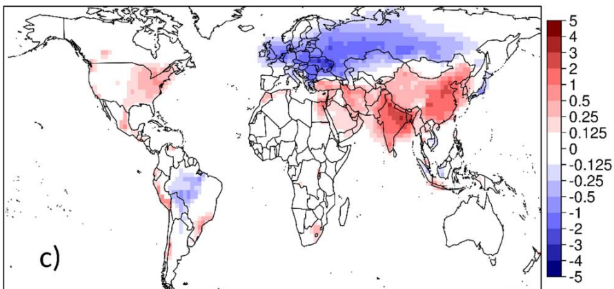
Figure 5. Simulated changes in annual mean surface PM 2.5 due to (a) LULCC, (b) agricultural emission changes, and (c) the combined effects of agricultural emissions and LULCC.
