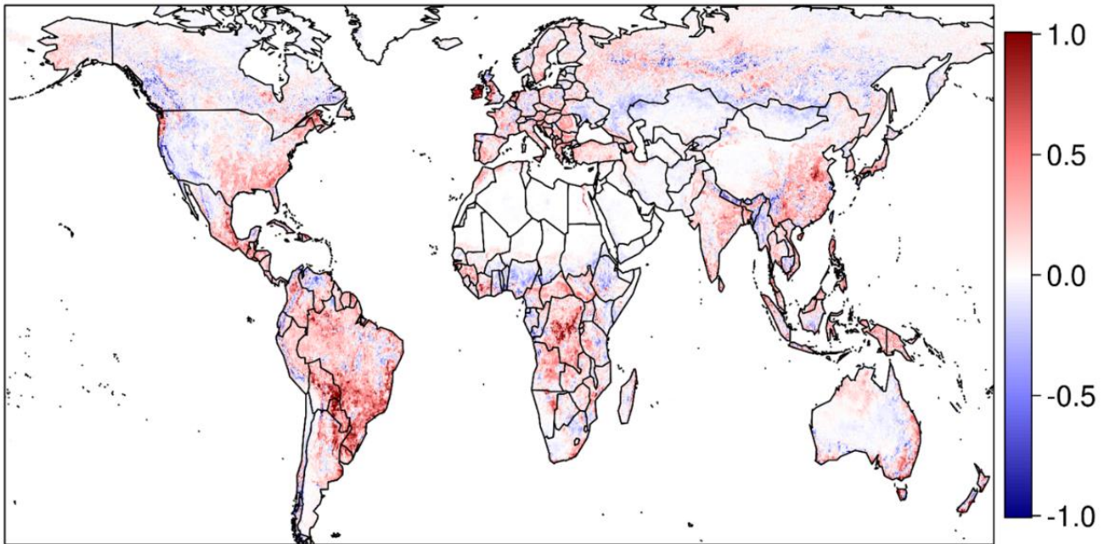
Figure 2. GLASS-derived changes in 3-year mean annual LAI (2012 to 2014 average minus 1991 to 1993 average).
