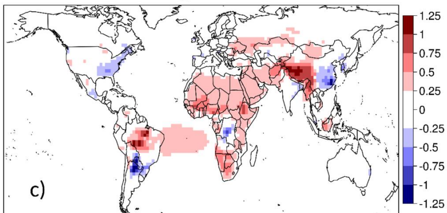
Figure 6. Simulated changes in annual mean surface O_3 due to (a) LULCC, (b) agricultural emission changes, and (c) the combined effects of agricultural emissions and LULCC.
