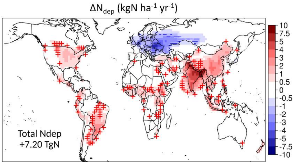
830 Figure 7. Changes in total nitrogen deposition ( \Delta N_{\text{dep}} ) due to changes (1992-2014) in agricultural emissions and land cover. Red plus signs (+) mark new gridcells where total nitrogen deposition exceeds 5 \text{ kg N ha}^{-1} \text{yr}^{-1} , while blue minus signs (-) denote the gridcells where total nitrogen deposition decreases to below 5 \text{ kg N ha}^{-1} \text{yr}^{-1} .
