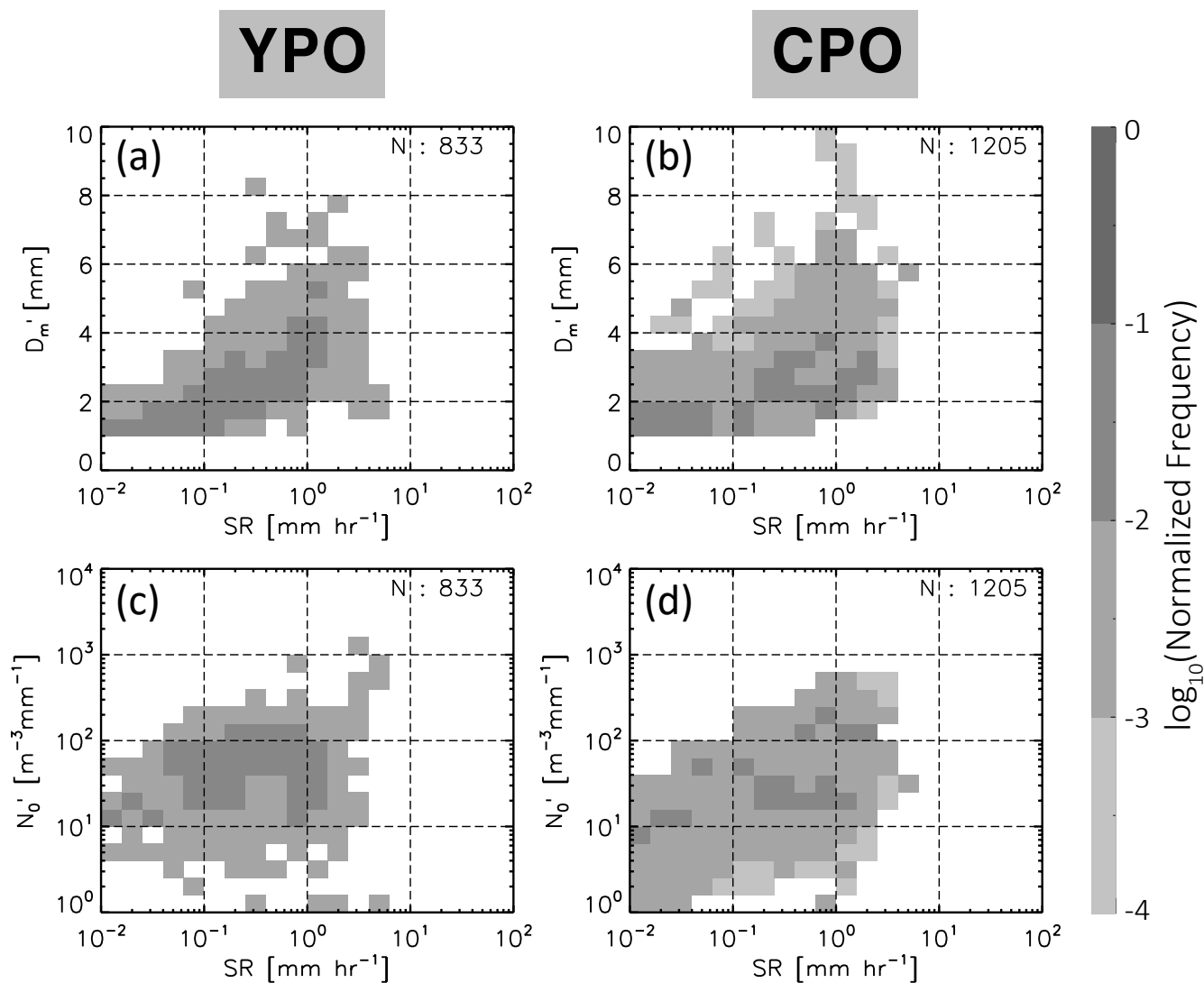
Figure 9. Normalized frequency of D'_m - SR (first row) and N'_0 - SR (second row) at YPO and CPO sites for the cold low events.
