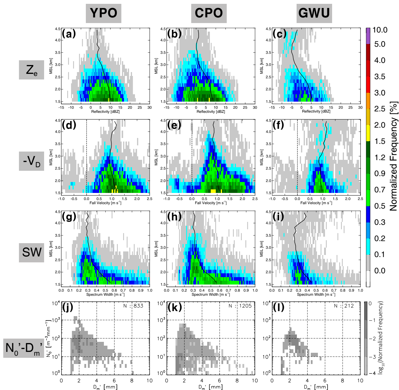
Figure 8. Same as in Fig. 6, except for the cold low events.
