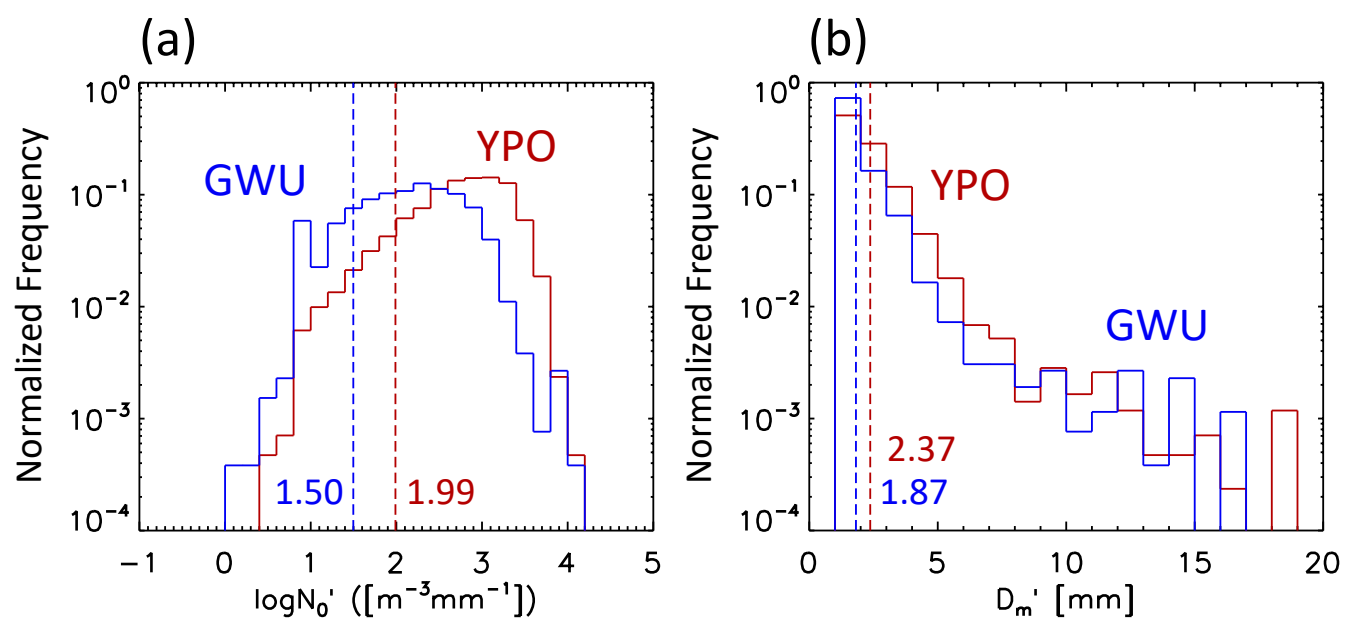
Figure 4. Normalized frequency of (a) \log N'_0 and (b) D'_m for YPO (in red) and GWU (in blue) sites. Dashed lines denote the mean value of each site.
