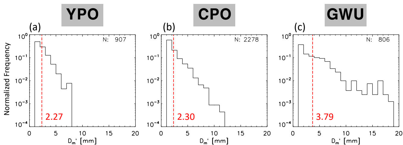
Figure 7. Normalized frequency of D'_m at (a) YPO, (b) CPO, and (c) GWU sites for air-sea interaction events during 2-yr winters. Red dashed line indicates the average value for each diagram.
