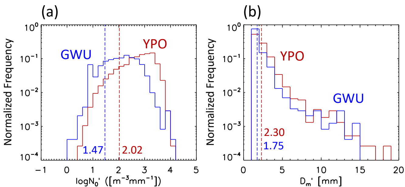
Figure 11. Same as in Fig. 4, except for the warm low events.
