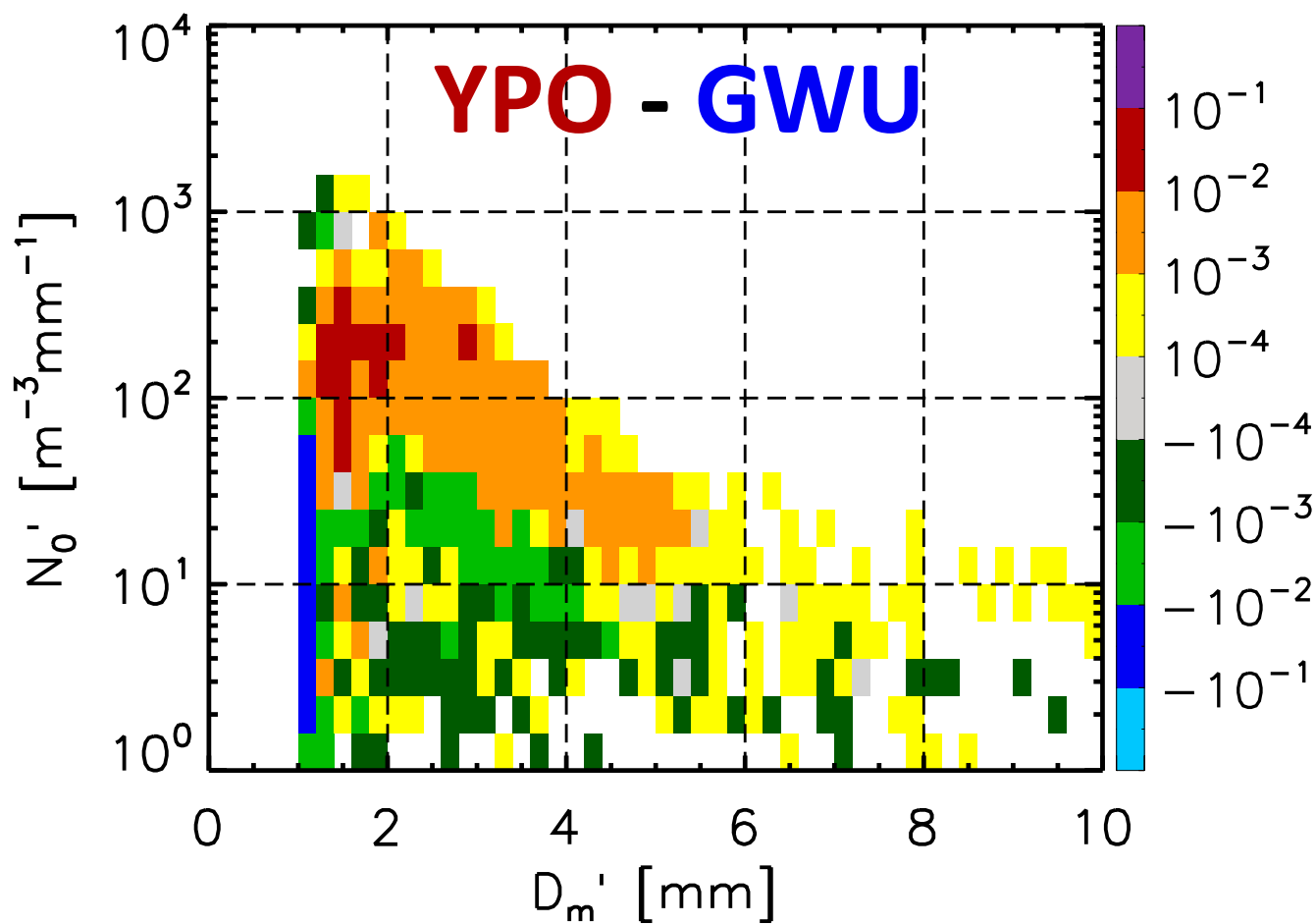
Figure 5. Difference of normalized frequency of N'_0 - D'_m between YPO and GWU sites. Warm (cold) color indicates YPO (GWU) has more frequency.
