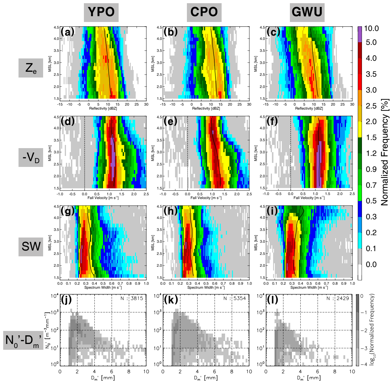
Figure 10. Same as in Fig. 6, except for the warm low events.
