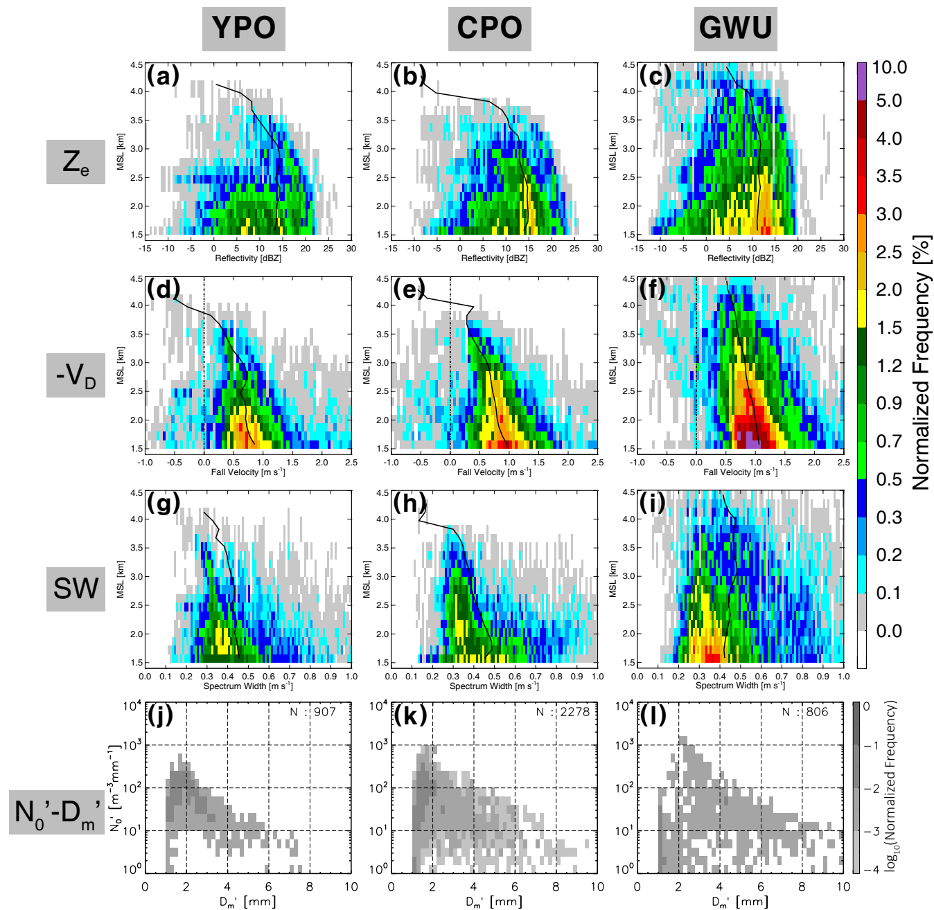
Figure 6. CFADs of radar reflectivity (dBZ, first row), negative of Doppler radial velocity (m s -1 , second row), and spectral width (m s -1 , third row) from MRR (first three rows) and normalized frequency of N'_0-D'_m (fourth row) at YPO, CPO, and GWU sites for the air–sea interaction events during 2-yr winters. The number of snow-observed minutes at the ground by PARSIVEL is shown in the upper right corner of the diagram in the fourth row.
