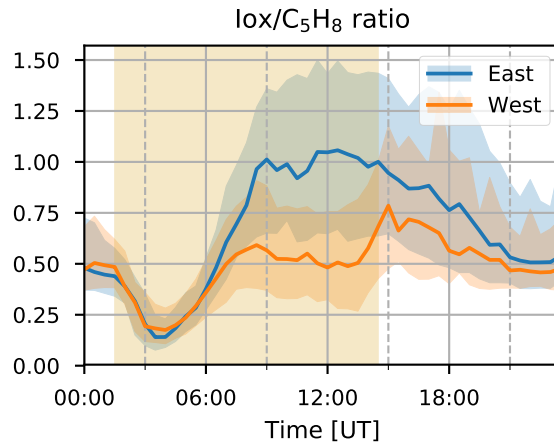
Figure 8. Median diel profile of ratio between isoprene oxidation products (Iox) and isoprene (C 5 H 8 ), separated according to the wind-direction observed at the Maïdo observatory, blue and orange for winds coming from the East and West respectively. Interquartile ranges for each direction is shown as shaded areas in the background with colors corresponding to the curve. The shaded yellow area in the back corresponds to median daylight period over the 2-year observation period.
