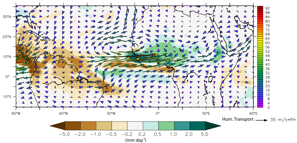
Figure 4. The contours represent the mean precipitation difference (mm d -1 ) due to the effect of absorbing dust obtained for the months JJAS for 30 years (1985 to 2014) by subtracting the precipitation fields of the experiment with dust and the experiments without dust in the IPSL-CM6 climate model where dust is run interactively. The arrows indicate the changes in mean humidity transport ( m/s*RH) for the same period.
