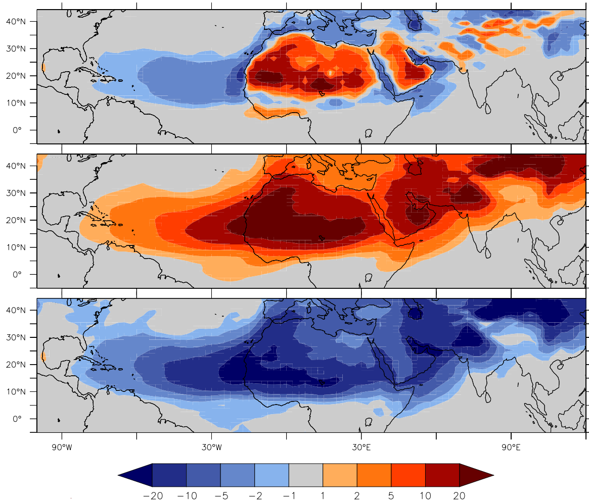
Figure 3. Top panel: Mean JJAS top-of-atmosphere (TOA) Dust Direct Radiative Effect (in W m -2 ); Middle panel: Mean JJAS dust Atmospheric Absorption (W m -2 ) which is obtained as the difference between top-of-atmosphere and surface effects; Bottom Panel: Mean JJAS surface Dust Radiative effect (W m -2 ) . Over the Sahel region (10°N to 20°N; 15°W to 35°E), at the TOA effect amounts to +6.0 W.m -2 (SW=+4.1, LW=+1.9); the atmospheric absorption amounts to +16.7 W.m -2 (SW=+19.9, LW=3.2); and the surface radiative effect amounts to -10.8 W.m -2 (SW=-15.8, LW=+5.1). In addition, Table 1 also indicates the values for the dust global direct radiative effect.
