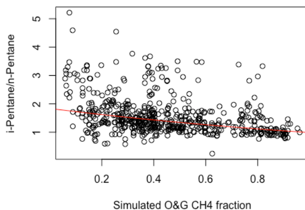
395 Figure 11. Scatter plot of the fraction of simulated methane due to O&G sources against i-pentane to n-pentane ratio. An exponential model is fitted to the data (red line).
