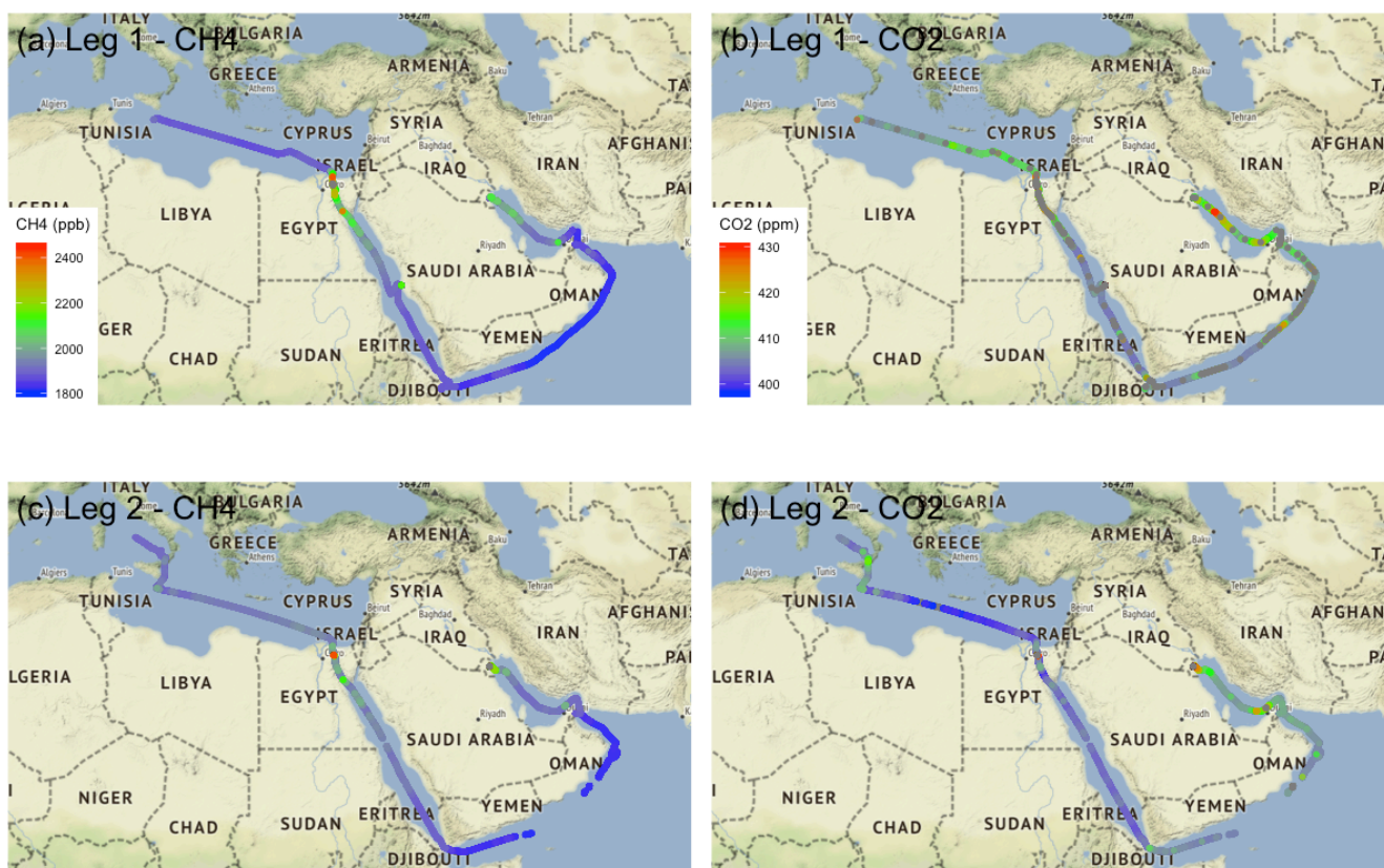
Figure 2. Measurements of methane (a, c) and carbon dioxide (b, d) collected during Leg 1 (top row) and Leg 2 (bottom row). Background map © OpenStreetMap contributors 2021. Distributed under a Creative Commons BY-SA License.
