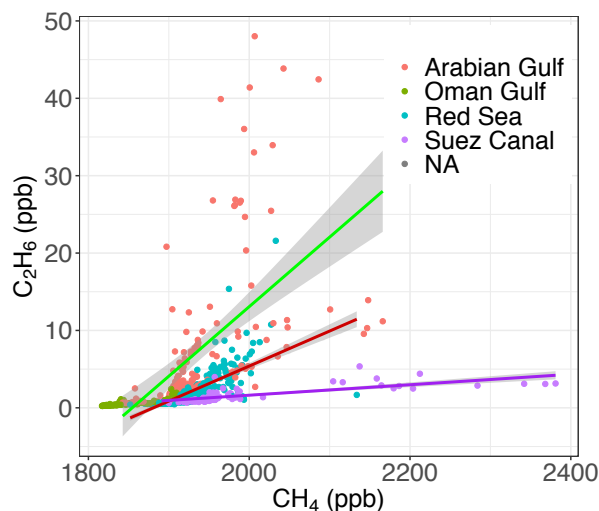
Figure 5. Scatter plot of ethane and methane for the Gulf of Oman gulf, Arabian Gulf, Red Sea and Suez Canal. The regression line and associated 95%-confidence interval are plotted for each of these 4 regions.
