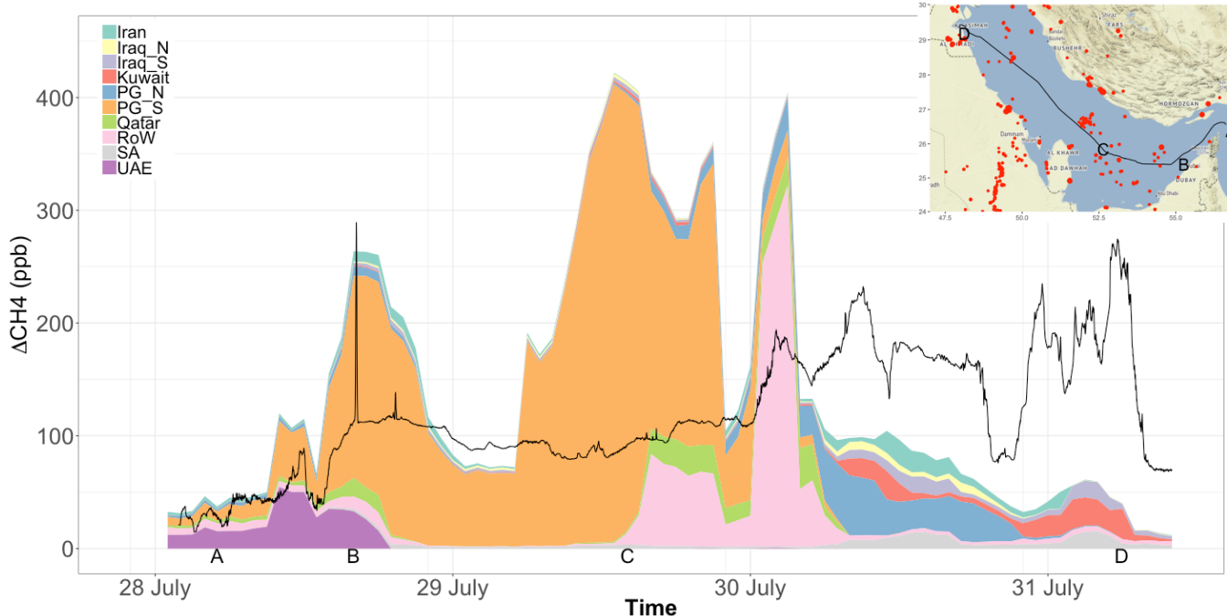
365 Figure 10. Simulation of \Delta\text{CH}_4 by country of origin over the Arabian Gulf. The solid line shows the measured \text{DCH}_4 . The simulated excess \text{CH}_4 is tagged and color-coded by country or area of origin. Iraq_N : Northern Iraq, Iraq_S: southern Iraq; PG_N: Persian (Arabian) Gulf, Northern half; PG_S: Persian (Arabian) Gulf, Southern half; RoW: Rest of the World; SA: Saudi Arabia; UAE: United Arab Emirates. The inset shows the trajectory of the ship corresponding to the simulation, and the labels A, B, C, D highlight points of the ship's route discussed in the main text. Red points correspond to flaring detected from space (see Fig. 4) at the time of the campaign. Inset background map © OpenStreetMap contributors 2021. Distributed under a Creative Commons BY-SA License.
