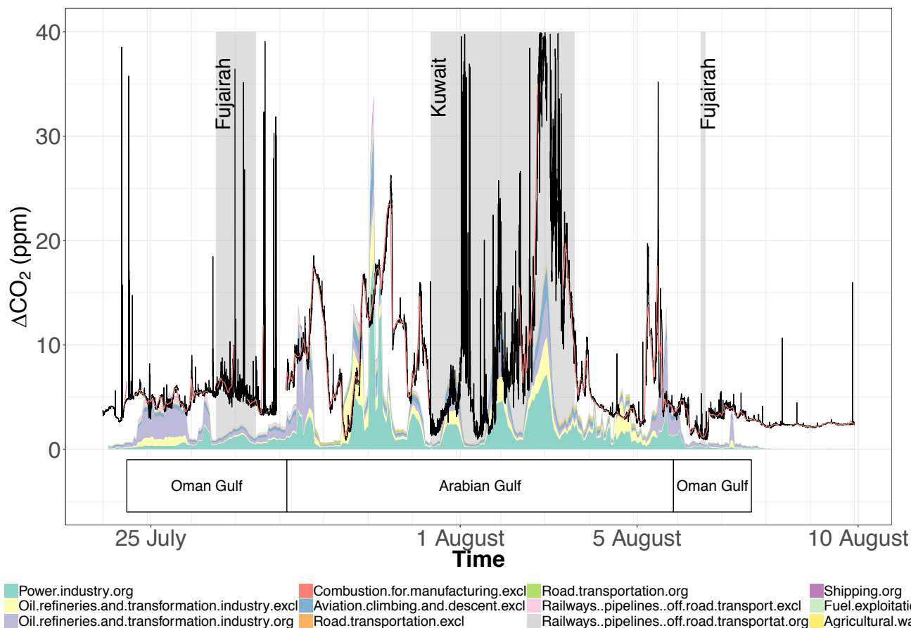
Figure 9. Comparison of simulated excess CO 2 time series at the receptor position in the Gulf of Oman and Arabian Gulf, and hourly average ΔCO 2 measured from the ship (black line). Flagged, hourly average data is shown in light red. The simulation combines Flexpart potential emission sensitivity and EDGAR inventory (stacked areas). The main source sectors are indicated as color code. The stops at harbor are indicated as shaded grey areas, with the names of harbors indicated at the top.
