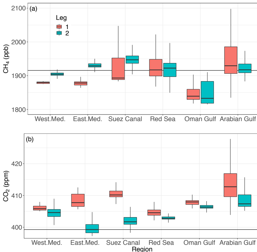
200 Figure 3. Methane (a) and carbon dioxide (b) mixing ratios observed during the cruise. Data from ship at rest or contaminated by ship own exhaust are excluded. The box plot shows the interquartile range (25-75%) and median values for each grouping of data. The bars extend to the lowest and highest values, (ignoring outliers beyond 1.5 times the interquartile range). The statistics of the two legs are represented separately. The horizontal black line is the mean methane mixing ratio at Mace Head, Ireland (NOAA) 205 during July and August 2017. The median mixing ratio of CO 2 over the Aden and Arabian Sea are comparable to Red Sea and Mediterranean values, contrary to CH 4 where mixing ratios were distinctly lower. CO 2 mixing ratios do however exhibit a much lower variability (interquartile range) compared to other regions.
