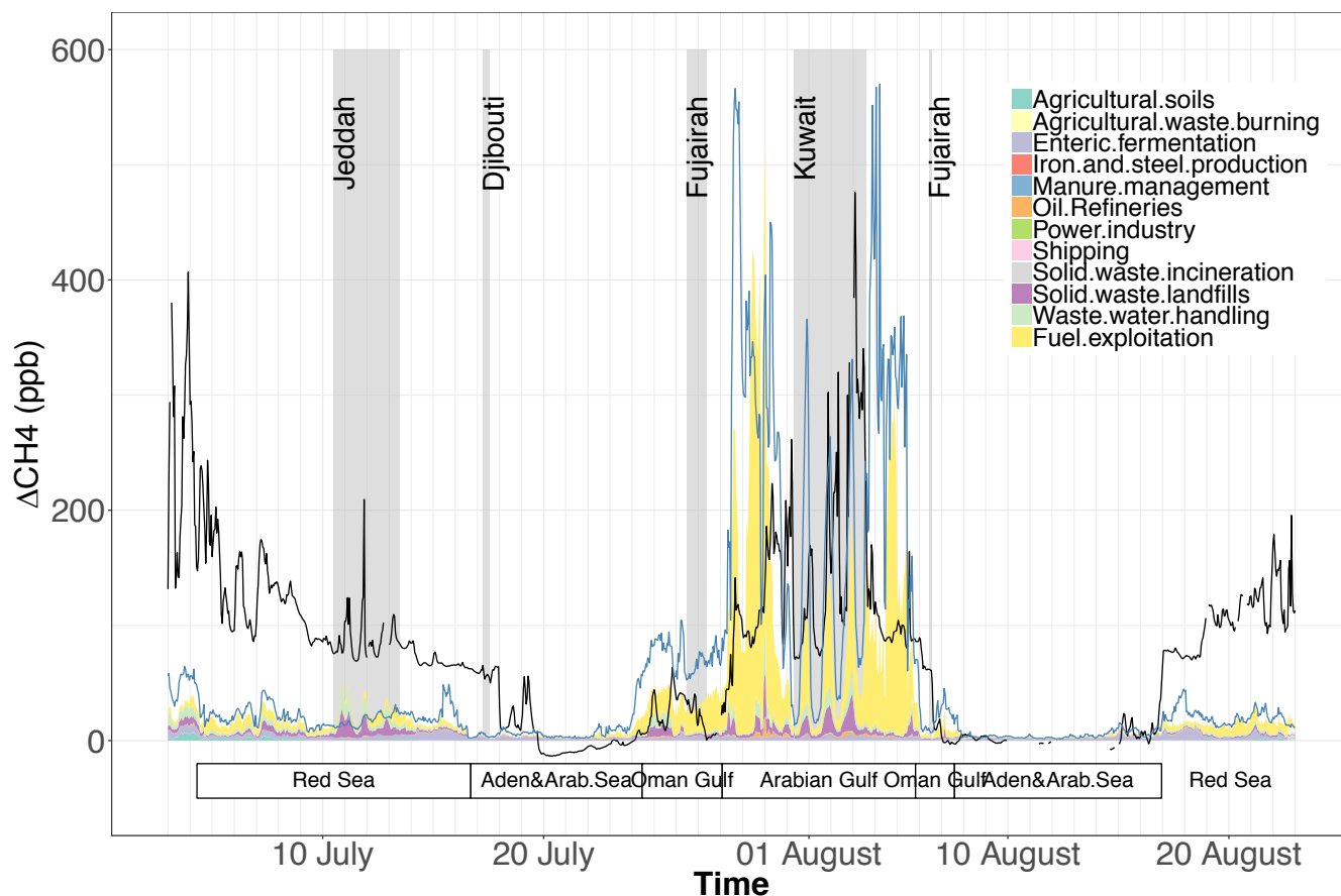
Figure 8. Comparison of simulated excess \text{CH}_4 time series at the receptor position, and hourly average \Delta\text{CH}_4 measured from the ship (black line). The simulation combines Flexpart potential emission sensitivity and EDGAR inventory (stacked areas). The main source sectors are indicated as color code. The potential emission sensitivity is also combined with the Eclipse inventory for comparison (blue line). The stops at harbor are indicated as shaded grey areas, with the names of harbors indicated at the top.
