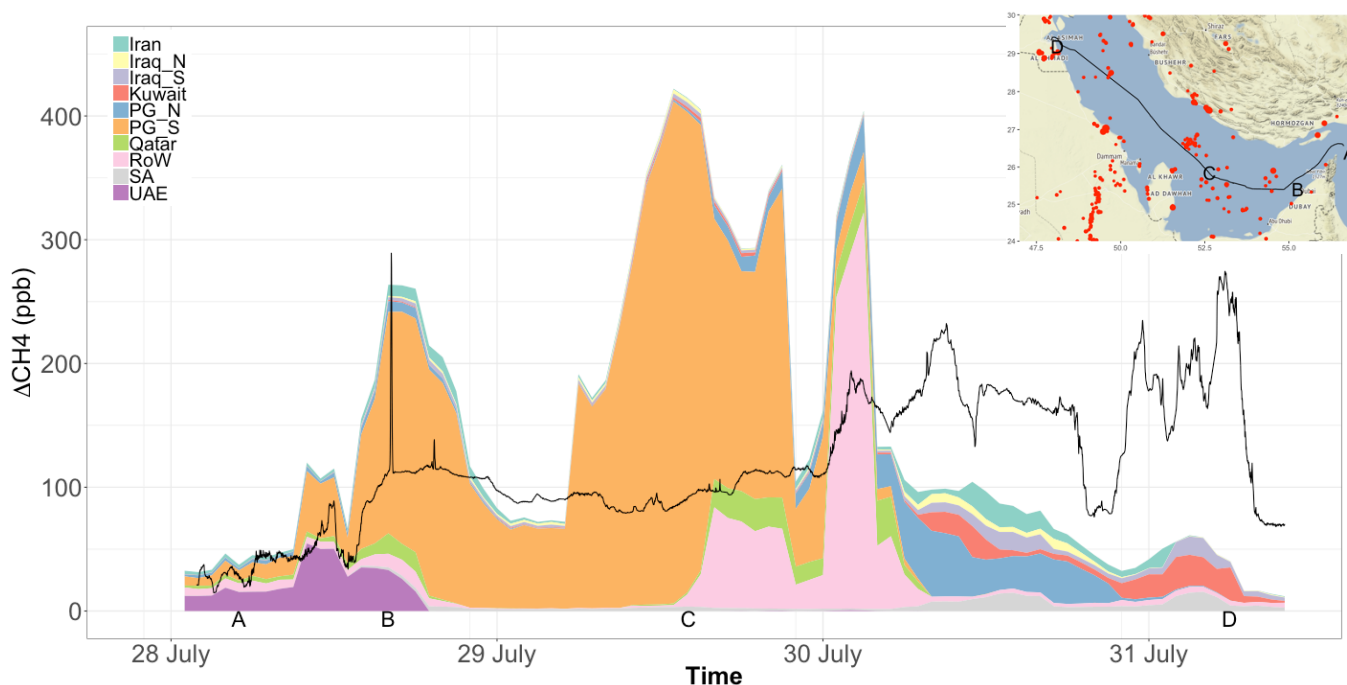
390 Figure 10. Simulation of \Delta\text{CH}_4 by country of origin over the Arabian Gulf. The solid line shows the measured \Delta\text{CH}_4 . The simulated excess CH 4 is tagged and color-coded by country or area of origin. Iraq_N : Northern Iraq, Iraq_S: southern Iraq; PG_N: Persian (Arabian) Gulf, Northern half; PG_S: Persian (Arabian) Gulf, Southern half; RoW: Rest of the World; SA: Saudi Arabia; UAE: United Arab Emirates. The inset shows the trajectory of the ship corresponding to the simulation, and the labels A, B, C, D highlight points of the ship's route discussed in the main text. Red points correspond to flaring detected from space (see Fig. 4) at the time of 395 the campaign. Inset background map © OpenStreetMap contributors 2021. Distributed under the Open Data Commons Open Database License (ODbL) v1.0.
