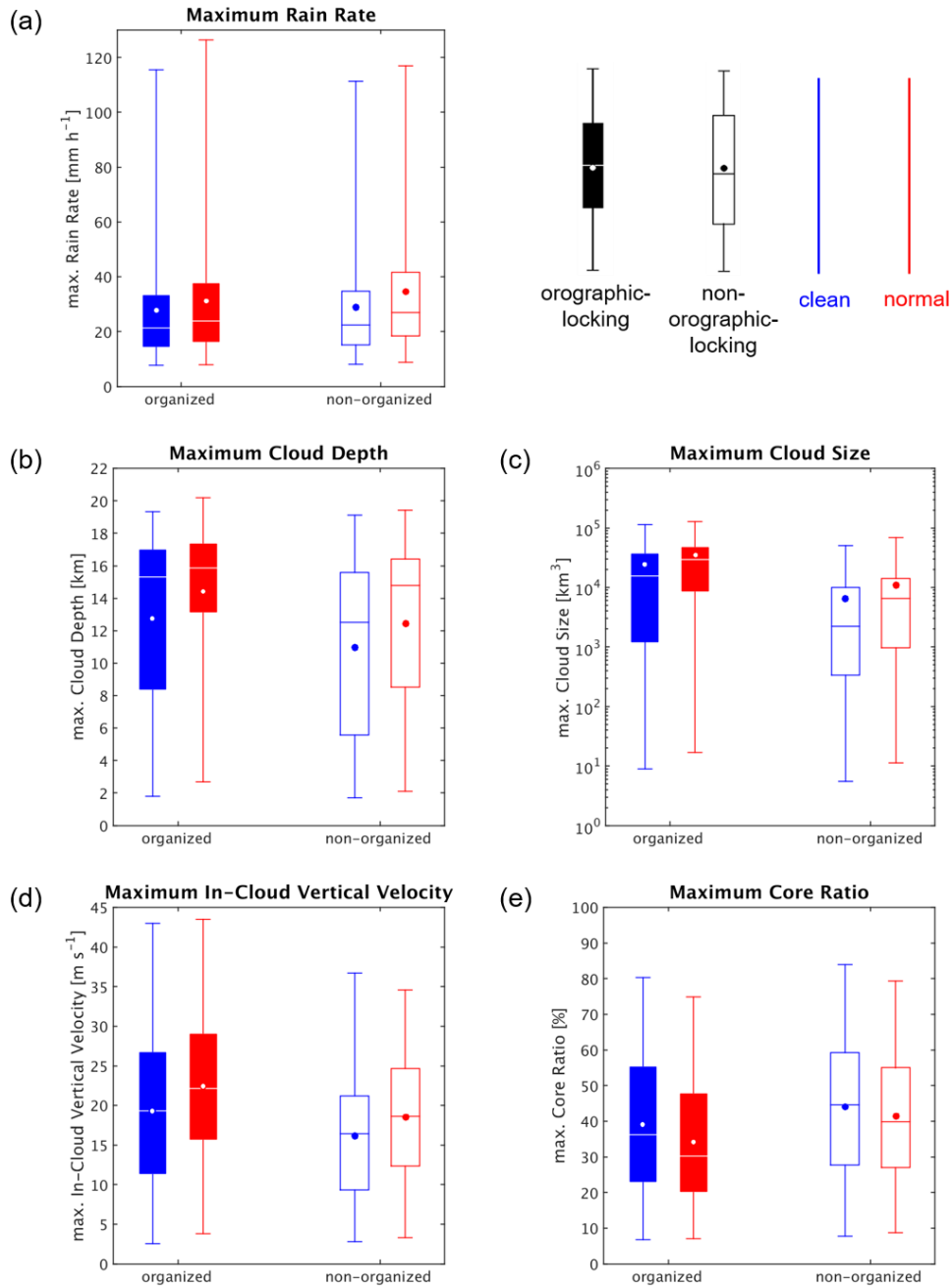
Figure 8. The box-whisker plots of the maximum (a) rain rate, (b) cloud depth, (c) cloud size, (d) in-cloud vertical velocity, and (e) core ratio during the lifetime of the diurnal precipitating systems. The core ratio is defined as the proportion of the clouds with a vertical velocity greater than 0.5 \text{ m s}^{-1} , indicating the ratio of the updraft region. The blue and the red boxes represent the results of the clean and the normal scenarios, respect. The filled boxes represent the organized regime, while the hollow boxes represent the non-organized regime. The dots on the box-whisker plots are the mean values.
