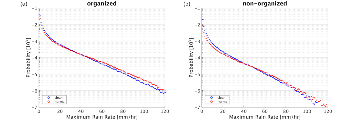
Figure 7. The probability density functions of the maximum rain rates of the convective cloud objects for the (a) organized regime and, (b) the non-organized regime. The blue and the red circles represent the results of the clean and the normal scenarios, respectively.
