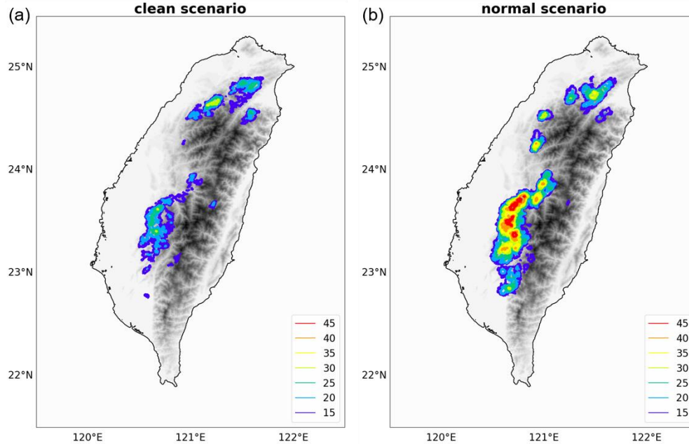
Figure 6. The occurrence counts of convective systems with maximum rain rate greater than 100 \text{ mm hr}^{-1} under (a) the clean scenario, and (b) the normal scenario.
