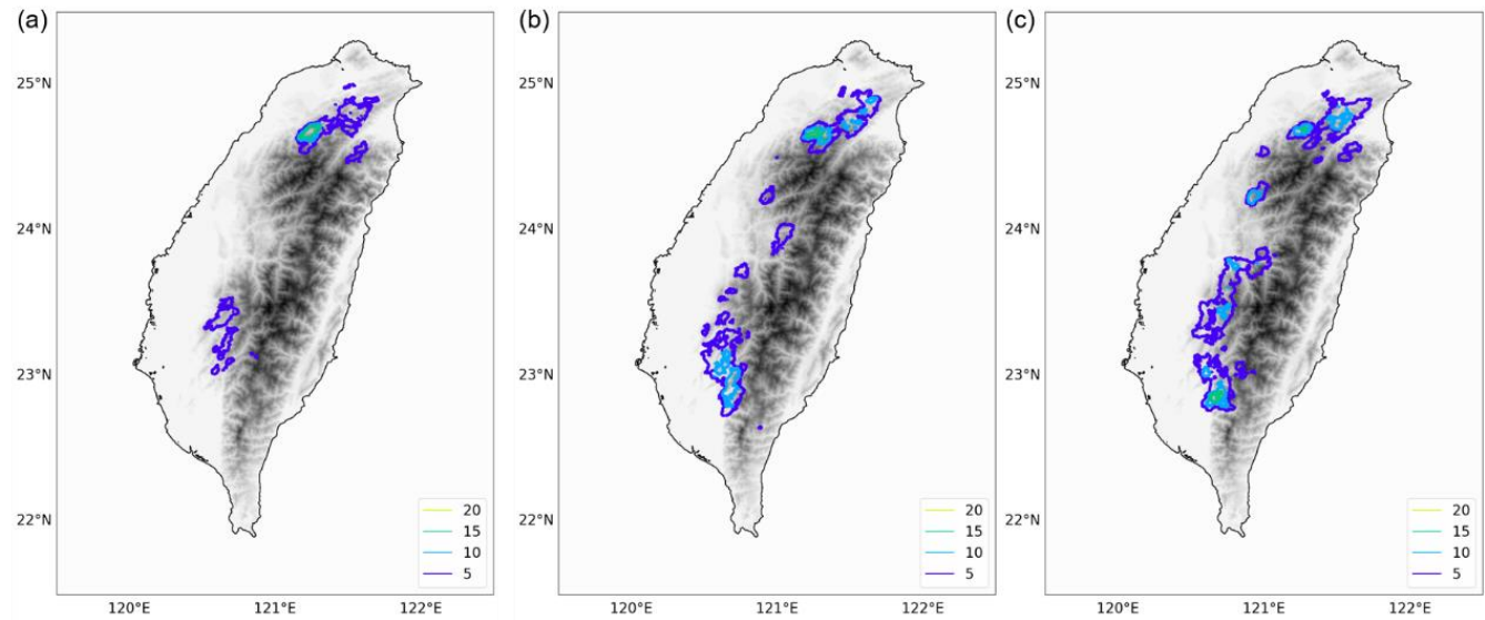
Figure B1. The occurrence counts of convective systems with maximum rain rate greater than 100 mm hr -1 when CCN concentration is (a) 3×10 8 kg -1 , (b) 3×10 9 kg -1 , and (c) 3×10 10 kg -1 .
