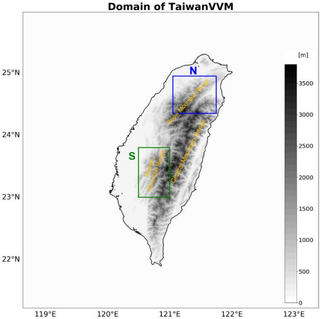
Figure 1. The domain of TaiwanVVM with the 500 m resolution topography of Taiwan Island (grey shading). The boxes are the mountain areas for subsequent statistical analyses: the blue box is the northern mountain area (area N), and the green box 135 is the southern mountain area (area S).
