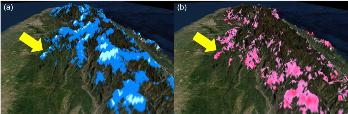
Figure 5. (a) The composite initiation time of precipitation under the clean scenario in area S. The light blue and dark blue areas represent the initiation time from 10:00 to 12:00 and from 12:00 to 13:00. (b) The area of precipitation initiation delaying for more than 1.5 hours due to increasing CCN in area S.
