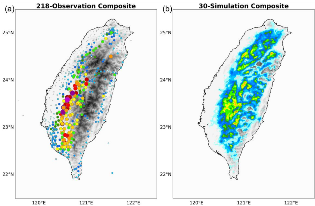
Figure 4. The composite daily mean precipitation of (a) all 218 weak-synoptic days from Central Weather Bureau rain gauge observations (the sizes of colored dots are scaled with the mean precipitation), (b) all 30 semi-realistic simulations under the clean scenario on Taiwan Island. Grey shadings show the orographic heights (same as Fig. 1).
