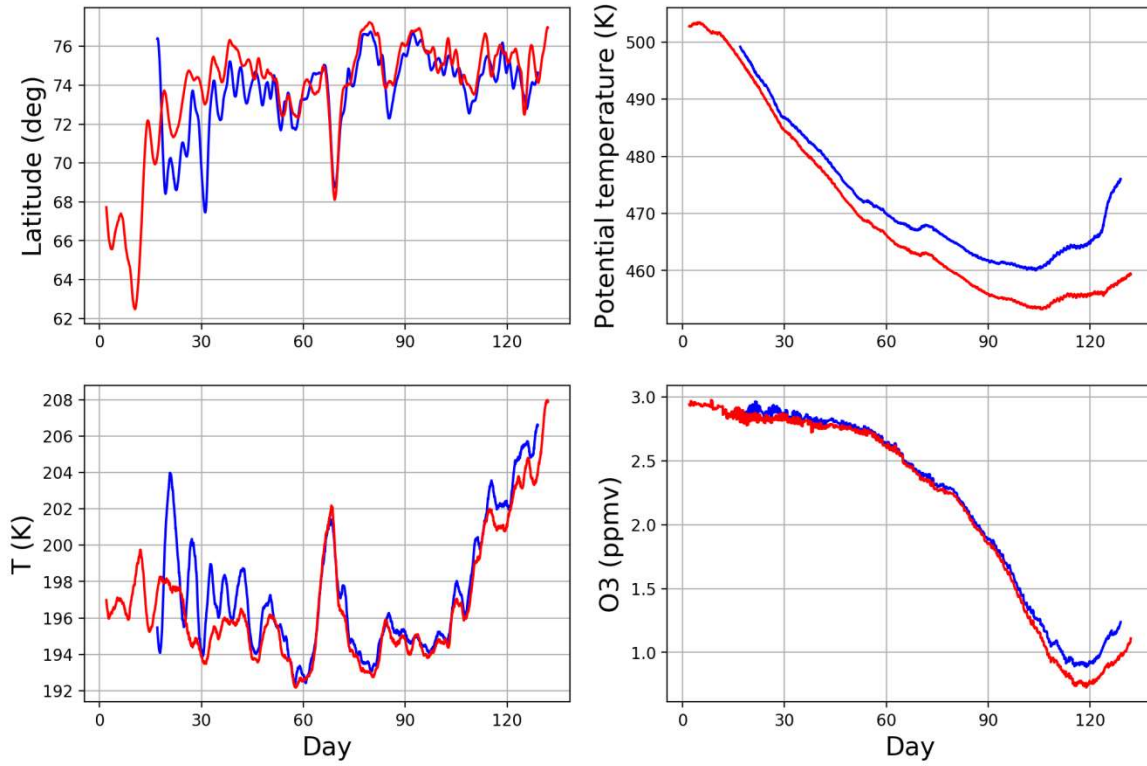
Fig.S2.3. Same as Fig. S2.1 for winter-spring 2019-2020.
