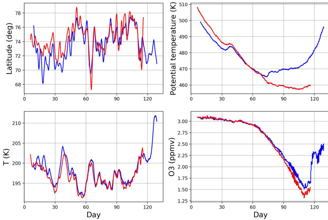
Fig.S2.1. Trajectory ensemble averaged latitude (top-left), potential temperature (top-right), temperature (bottom-left) and ozone (bottom-right); backward (red), forward (blue) for winter-spring 2010-2011.
