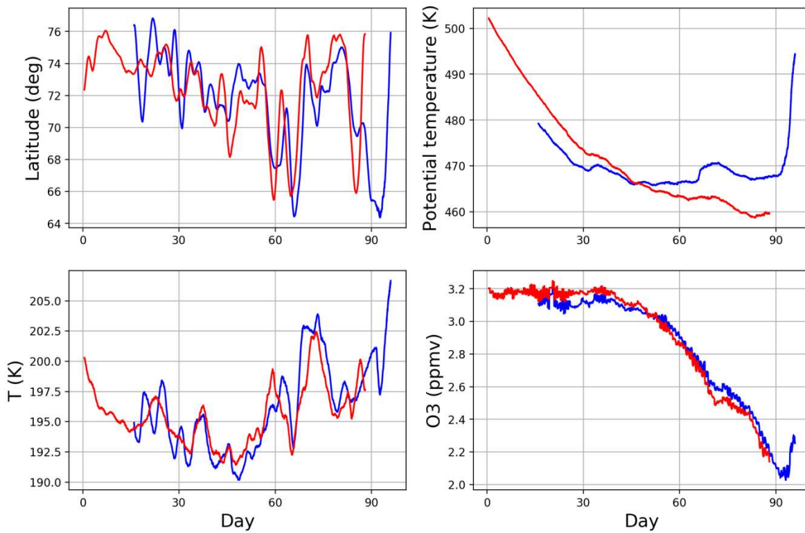
Fig.S2.2. Same as Fig.S2.1 for winter-spring 2015-2016.
