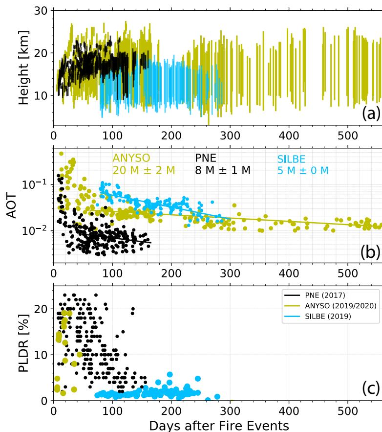
Figure 10. Comparison of geometrical and optical properties of three stratospheric fire smoke events measured with different Polly instruments. Day 0 is the 12 August 2017 (PNE), 23 July 2019 (SILBE), and 31 December 2019 (ANYSO). Canadian (PNE) and Siberian (SILBE) fire smoke data are taken from Baars et al. (2019) and Ohneiser et al. (2021), respectively. (a) Overview of Polly observations of UTLS smoke layers (colored bars from layer base to top) in days after smoke injection into the UTLS height regime. (b) 532 nm AOT times series for the different wildfire events, straight lines indicate the decay of the perturbations according to the given e-folding decay times in months (M). In the case of PNE and ANYSO observations, AOT for heights >13 km is used. (c) Particle depolarization ratios (layer mean values) for the different fire events.
