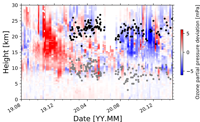
Figure 12. Deviation of the ozone partial pressure (with respect to the 2000-2020 mean value) at the Neumayer Station (data from NDACC, 2021). The base (grey dots) and top heights (black dots) of the Australian smoke layer measured with Polly at Punta Arenas indicate the smoke-polluted height range.
