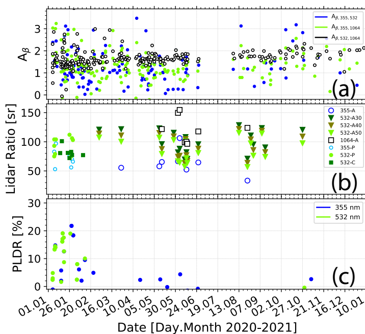
Figure 8. Smoke layer mean optical properties observed from 1 January 2020 to 10 January 2021: (a) Backscatter-related Ångström exponent A_{\beta} , (b) extinction-to-backscatter ratio (lidar ratio) from Polly (P) and CORAL (C) measurements in January–February 2020, and from combined lidar-AERONET observations (since March 2020) by using lidar ratios of 30 (A30), 40 (A, A40), and 50 sr (A50) in the estimation of the tropospheric 532 nm AOT from lidar observations (see further explanation in the text). Stratospheric lidar ratios at 355 nm (circles) and 1064 nm (squares) are shown for a lidar ratio of 40 sr in the tropospheric AOT retrieval. (c) Particle linear depolarization ratio (PLDR). The scatter in the data is mainly caused by signal noise and to a minor part by atmospheric variability.
