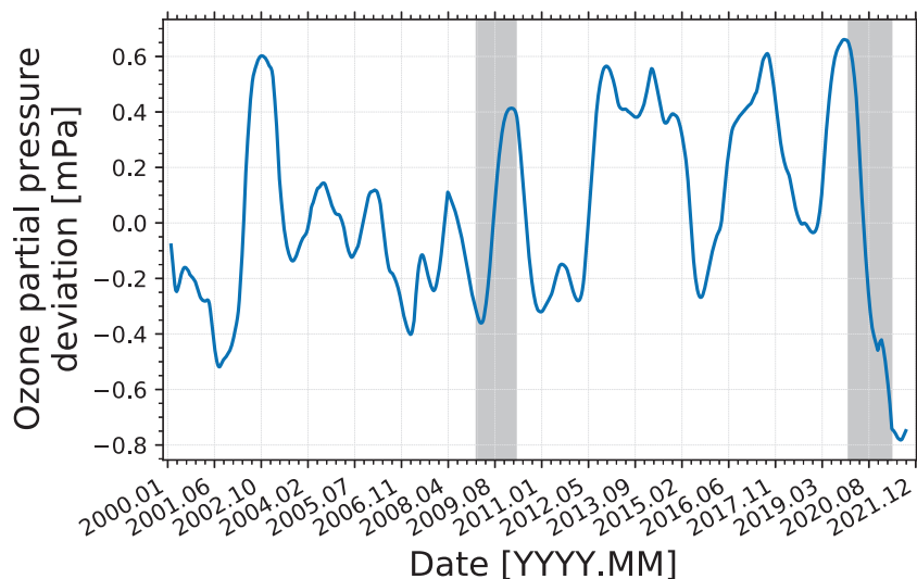
Figure 11. Deviation of the vertically averaged ozone partial pressure from the respective 2000-2020 long-term mean ozone value (of 5.9 mPa). Ozone profiles measured regularly (typically one ozonesonde launch per week) at Lauder (New Zealand), the German Antarctic Neumayer Station, and at the South Pole (data from NDACC, 2021) are considered. Grey columns mark two time periods after major Australian fire events in 2009 (Black Saturday) and 2019/2020 (Black Summer).
