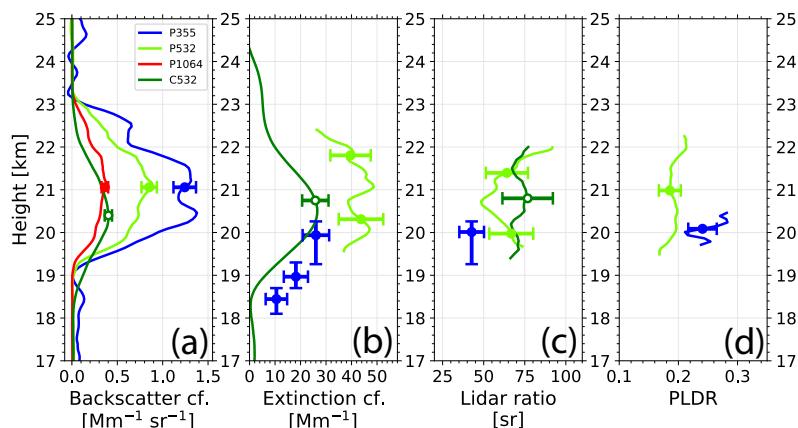
Figure 5. Profiles of smoke optical properties measured with Polly (P, closed circles) over Punta Arenas and with CORAL (C, open circles) over Río Grande on 26 January 2020 between 04:27–06:18 UTC (Polly) and 6:14–8:02 UTC (CORAL). (a) Particle backscatter coefficient at three wavelengths, (b) smoke extinction coefficient, (c) smoke extinction-to-backscatter ratio (lidar ratio), (d) particle linear depolarization ratio. Error bars show the estimated uncertainties. The extinction coefficient and lidar ratio profiles at 355 nm wavelength were noisy, so only a few trustworthy values are shown. Smoothing and regression window lengths are 500 m (Polly, backscatter, depolarization) and 2 km (extinction, lidar ratio). 2 km smoothing and regression window lengths are used in the case of the CORAL profiles.
