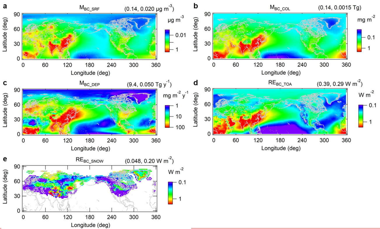
Figure 6: Spatial distributions of (a) M_{BC\_SRF} , (b) M_{BC\_COL} , (c) M_{BC\_DEP} , (d) RE_{BC\_TOA} , and (e) RE_{BC\_SNOW} in the Northern Hemisphere. The values in the parentheses are show global (left) and Arctic (right) mean values (annual mean). Purple shows areas where values are below the minimum shown on the colour bars.
