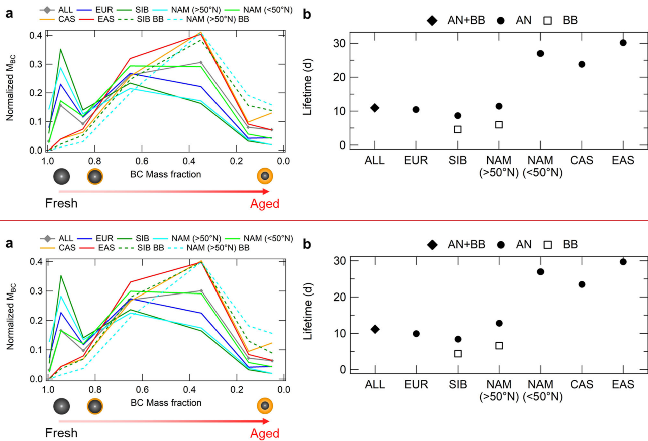
815 Figure 1244: (a) BC mixing state distributions for total BC mass (ALL) and for BC mass from the eight major sources (six anthropogenic (AN) sources and two biomass burning (BB) sources). BC particles are gradually shifted from the left (fresh BC with a lower MAC_{BC} ) to the right (aged BC with a higher MAC_{BC} ) by aging processes in the atmosphere. (b) Lifetimes in the Arctic for total BC (ALL) and for BC from eight major sources. Lifetimes were defined by the ratio of BC deposition flux to atmospheric BC loading in the Arctic.
