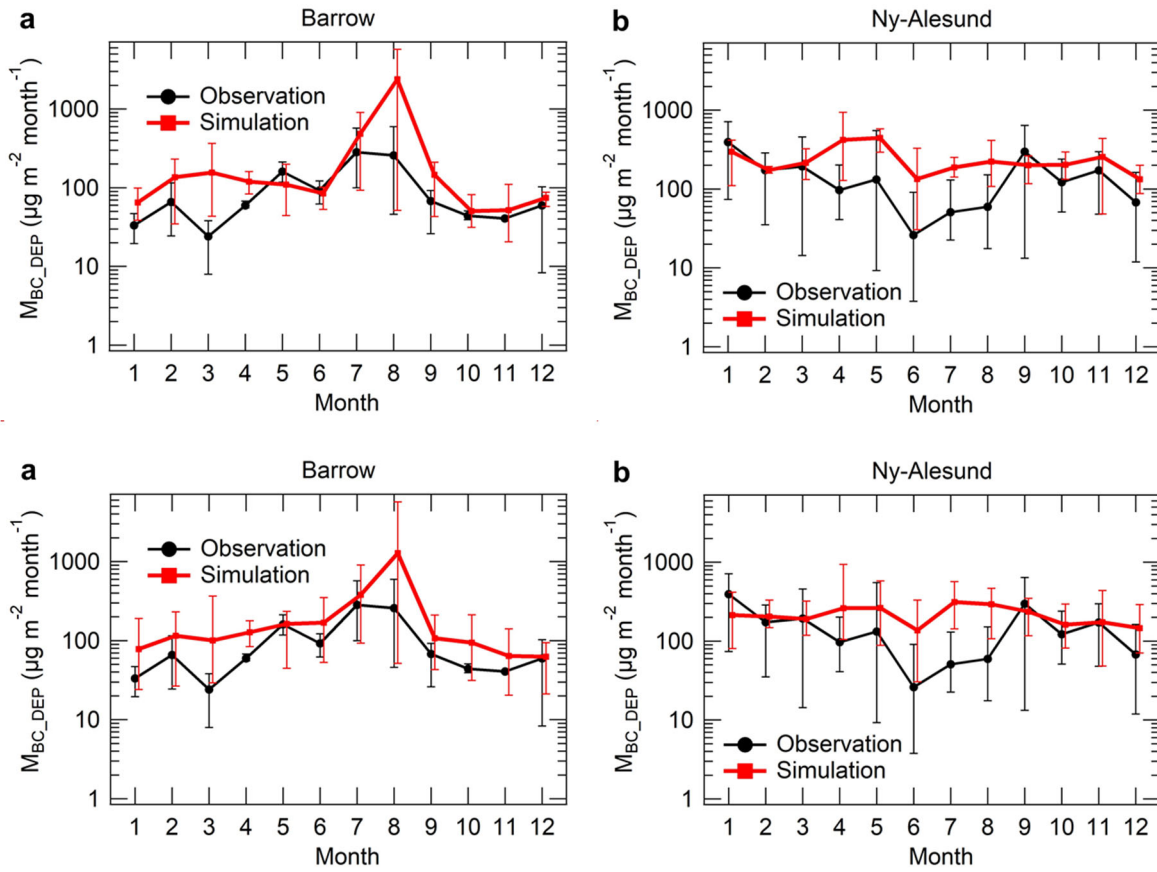
Figure 3: Comparisons between observations (black) and model simulations (red) for BC deposition flux ( M_{BC\_DEP} ) at (a) Barrow and (b) Ny-Ålesund. Model simulations in 2009– 2015 2011 were compared with observations in 2013–2017 because M_{BC\_DEP} observation data are available during 2013–2017 only . The error bars show the interannual variability ( maximum–minimum ranges ) of M_{BC\_DEP} the target variable .
