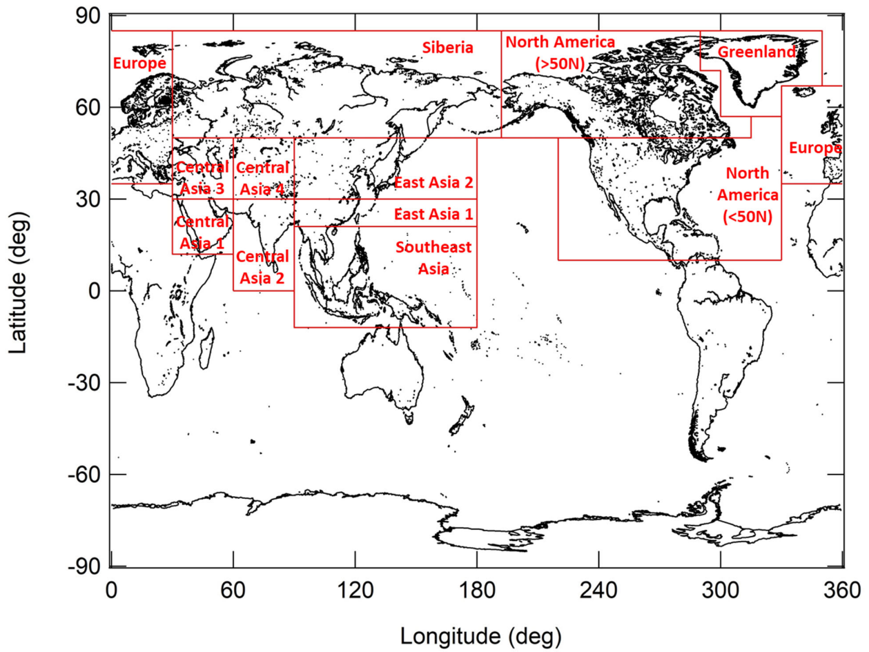
720 Figure 1: The definition of source regions used in this study. The 13 source regions are Europe (EUR), Siberia (SIB), Greenland (GL), North America north of 50°N (NAM (>50°N)), North America south of 50°N (NAM (<50°N)), Central Asia (CAS) 1–4, East Asia (EAS) 1–2, Southeast Asia (SAS), and Others. Anthropogenic and biomass burning BC from each source region are tracked by tag tracers in global aerosol model simulations using CAM-ATRAS (Sect. 2).
