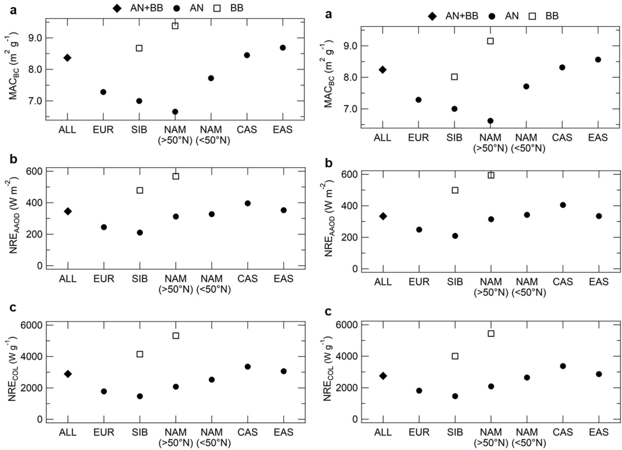
Figure 1149: Optical properties and radiative effect efficiencies in the Arctic for total BC (ALL; from all sources) and BC from the eight major sources (six anthropogenic (AN) sources and two biomass burning (BB) sources): (a) Mass absorption cross section of BC ( MAC_{BC} ), (b) BC radiative effect normalized by absorption aerosol optical depth (AAOD) of BC ( NRE_{AAOD} ; RE_{BC\_TOA} / AAOD_{BC} ) and (c) BC radiative effect normalized by M_{BC\_COL} ( NRE_{COL} ; RE_{BC\_TOA} / M_{BC\_COL} ).
