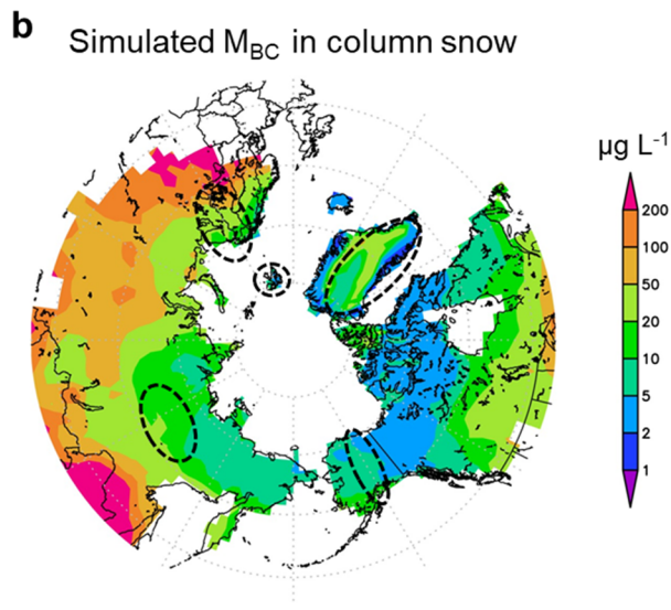
Figure 5: (a) Scatter plot of observed and simulated BC mass concentrations ( M_{BC} ) in snow in Finland (blue, circles), Alaska (light blue), Siberia (green), Greenland (black), and Ny-Ålesund (blue, squares). Observed data are taken from Mori et al. (2019). Simulation results (monthly averages) are shown for 3-year averages (2009–2011) for individual sampling points (latitude, longitude) and periods (years, months). Closed and open circles indicate M_{BC} in column snow and surface snow, respectively. The 1:1 line (solid black line) and the 10:1 and 1:10 lines (dashed lines) are also shown. (b) Simulated M_{BC} in column snow at high latitudes in the Northern Hemisphere in March (2009–2015/2011). Dashed circles indicate the approximate area where snow samplings were performed (Mori et al., 2019).
