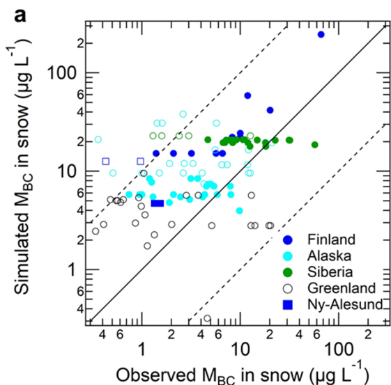
Figure 5: (a) Scatter plot of observed and simulated BC mass concentrations ( M_{BC} ) in snow in Finland (blue, circles), Alaska (light blue), Siberia (green), Greenland (black), and Ny-Ålesund (blue, squares). Observed data are taken from Mori et al. (2019). Simulation results (monthly averages) are shown for 3-year averages (2009–2011) for individual sampling points (latitude, longitude) and periods (years, months). Closed and open circles indicate M_{BC} in column snow and surface snow, respectively. The 1:1 line (solid black line) and the 10:1 and 1:10 lines (dashed lines) are also shown. (b) Simulated M_{BC} in column snow at high latitudes in the Northern Hemisphere in March (2009–2015/2011). Dashed circles indicate the approximate area where snow samplings were performed (Mori et al., 2019).
