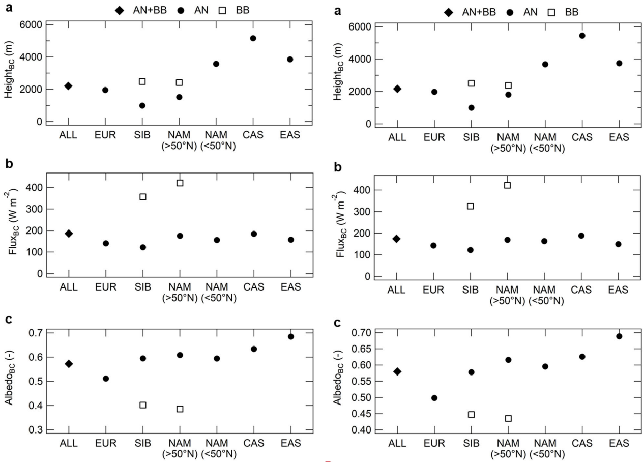
Figure 132: (a) Mean height (above sea level) ( Height_{BC} ), (b) mean solar radiation flux at the TOA ( Flux_{BC} ), and (c) mean surface albedo ( Albedo_{BC} ) weighted by BC concentrations in the Arctic (Eqs. 3–5) for total BC (ALL) and BC from eight major sources (six anthropogenic (AN) sources and two biomass burning (BB) sources).
