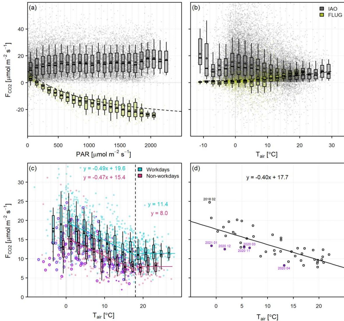
1502 1503 Figure 15: (a) 30-min daytime ( K_{\downarrow} > 5 \text{ W m}^{-2} ) observed CO 2 fluxes versus photosynthetically active radiation 1504 for all available data during the growing season (April-September, inclusive, but note that FLUG data are 1505 only available for 15 September 2017-22 May 2018); and (b) 30-min night-time ( K_{\downarrow} \leq 5 \text{ W m}^{-2} ) observed CO 2 1506 fluxes versus air temperature for the urban (IAO) and grassland (FLUG) sites. The dashed lines show (a) 1507 the light-response curve and (b) soil respiration rate for a grassland site in the nearby Stubai Valley 1508 (Wohlfahrt et al., 2005; Li et al., 2008). (c) Daily mean CO 2 flux versus daily mean air temperature separated 1509 into working and non-working days (daily values have been gap-filled using monthly median diurnal cycles 1510 for working and non-working days). Points outlined in purple occurred during Coronavirus restrictions. 1511 The vertical dashed line marks a base temperature of 18 ^{\circ}\text{C} above which F_{CO_2} does not decrease with 1512 temperature. (d) Average monthly observed CO 2 fluxes versus average monthly air temperature. Purple 1513 points indicate months with the strictest Coronavirus restrictions. In (a-c) boxes indicate the interquartile 1514 range, whiskers the 10 th -90 th percentile, horizontal bars the median and points the mean. In (c-d) solid lines 1515 are linear regressions with the equations given.
