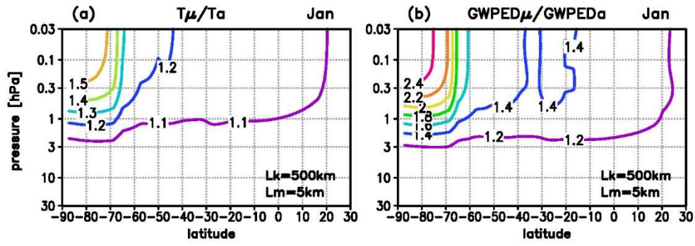
785 Figure 5: Cumulative amplification of the GW amplitude during the upward level-by-level propagation for a GW with L_k=500 \text{ km} and L_m=5 \text{ km} , (a) cumulative increase in the temperature amplitudes described by T_\mu/T_\alpha , (b) related increase in the gravity wave potential energy density (GWPED) described by E_\mu/E_\alpha ; background conditions: January 2001.
