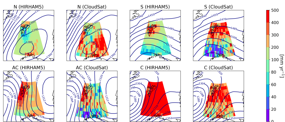
Figure 6. Snowfall rate composited to different CWTs, N (including N, NE, and NW) S (S, SE, and SW), C and AC, for the area of 10^{\circ} E- 40^{\circ} E (the colored sub-region is according Fig. 3d) between latitude bands 70^{\circ} - 81^{\circ} N for both HIRHAM5 and CloudSat. The mean 850 hPa geopotential height (gpdm) associated with the CWTs is also shown as blue contour lines.
