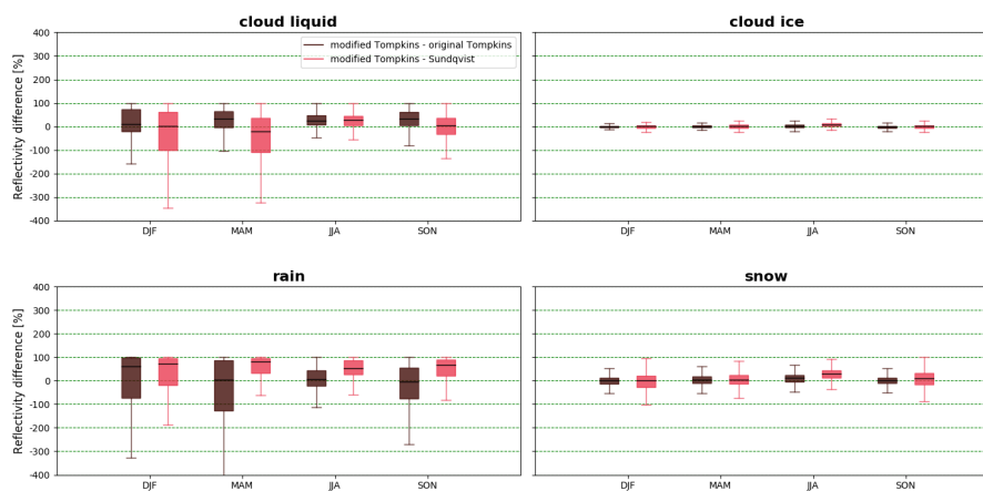
Figure A8. The box plot shows the differences in percents between the modified Tompkins scheme in respect to the two other schemes for different hydrometeors distributed seasonally.
