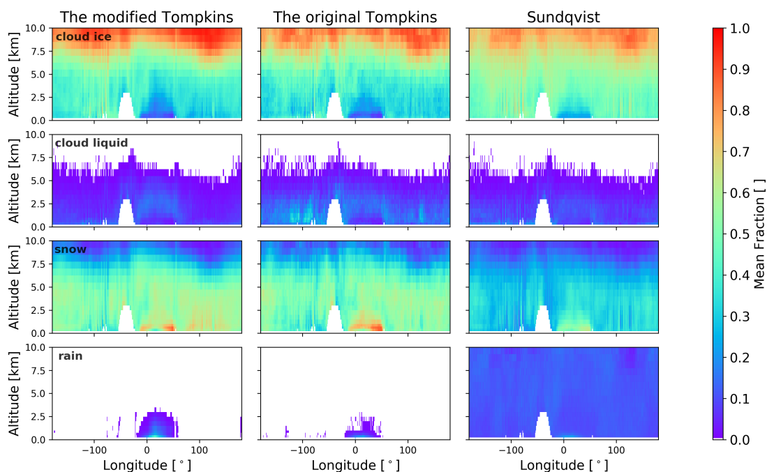
Figure A7. A mean fraction of reflectivity contributed by the different hydrometeors as a function of altitude for a latitude band of 72^{\circ} - 73^{\circ} N in winter(DJF) for the different microphysical schemes, the modified Tompkins (left panel), the original Tompkins (middle panel), and Sundqvist (right panel) schemes, respectively.
