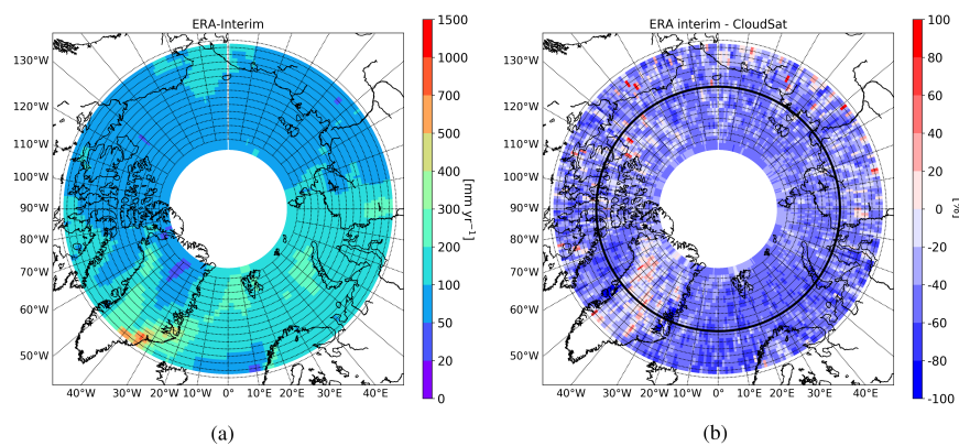
Figure A2. a) Yearly mean snowfall rate of ERA-Interim. b) Difference of snowfall rates between ERA-Interim and CloudSat.
