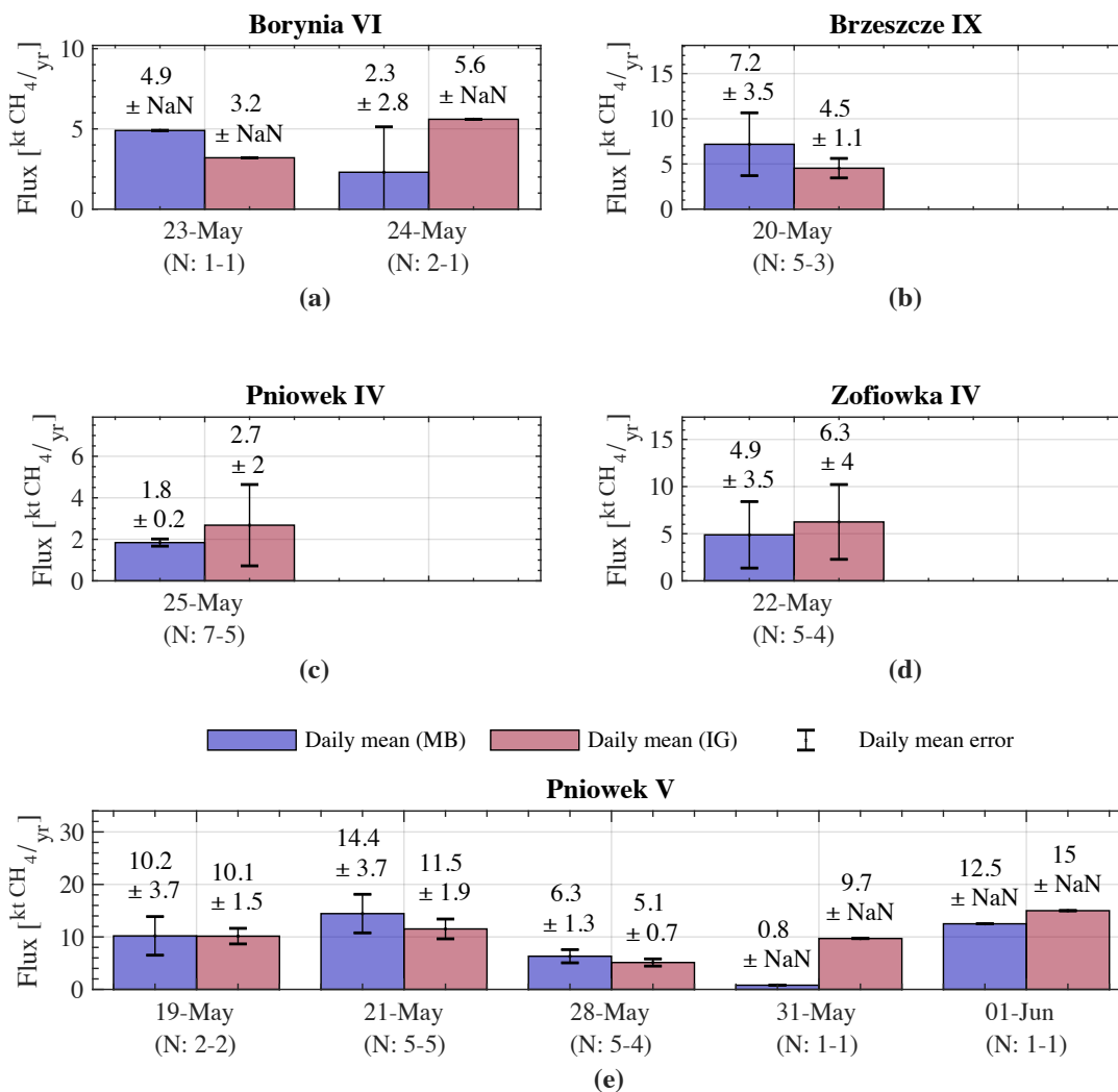
Figure 5. CH 4 emission estimates for each ventilation shaft per measurement day. light red: IG approach; light blue: MB approach. The bar height is the average of all flights during a specific day. Error bar indicates the standard deviation of the individual flights for that specific day, where the number of flights used for each bar is indicated with N. The two values for N refer to the MB approach and IG approach, respectively. The error is indicated as NaN when only one estimate is available.
