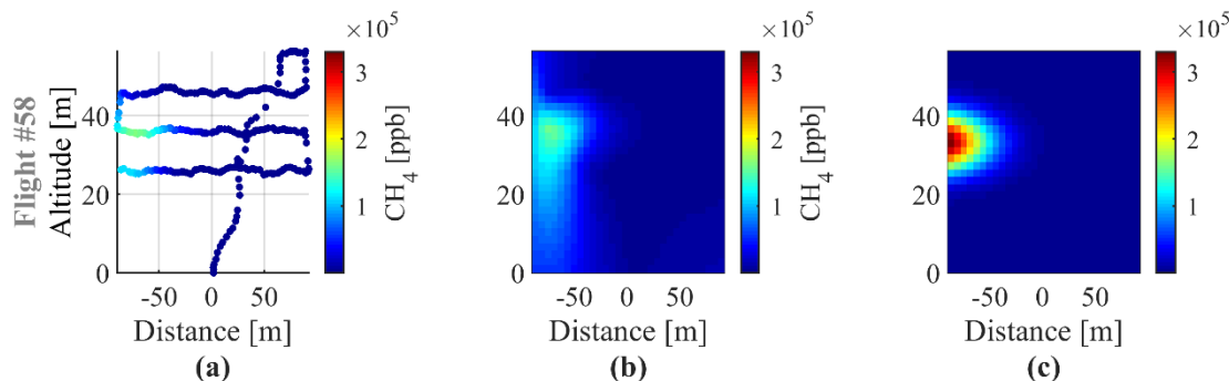
200 Figure 2. (a) a sampled downwind CH 4 mole fraction profile, (b) a kriged extrapolated 2D plane of CH 4 mole fractions for the MB approach and (c) an estimated 2D CH 4 mole fraction plane using the parameters retrieved from the IG approach.
