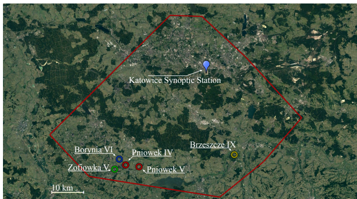
Figure 1. Google map showing the location of the 5 measured facilities (round markers) and the meteorological station where wind data for flights #5 to #33 was obtained. The red border indicates the total size of the Silesia Coal Basin where the majority of coal mining shafts were located. We have primarily performed measurements in the south-western part of the region.
