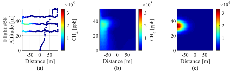
Figure 2. (a) a sampled downwind CH 4 mole fraction profile, (b) a kriged extrapolated 2D plane of CH 4 mole fractions for the MB approach and (c) an estimated 2D CH 4 mole fraction plane using the parameters retrieved from the JG approach.
