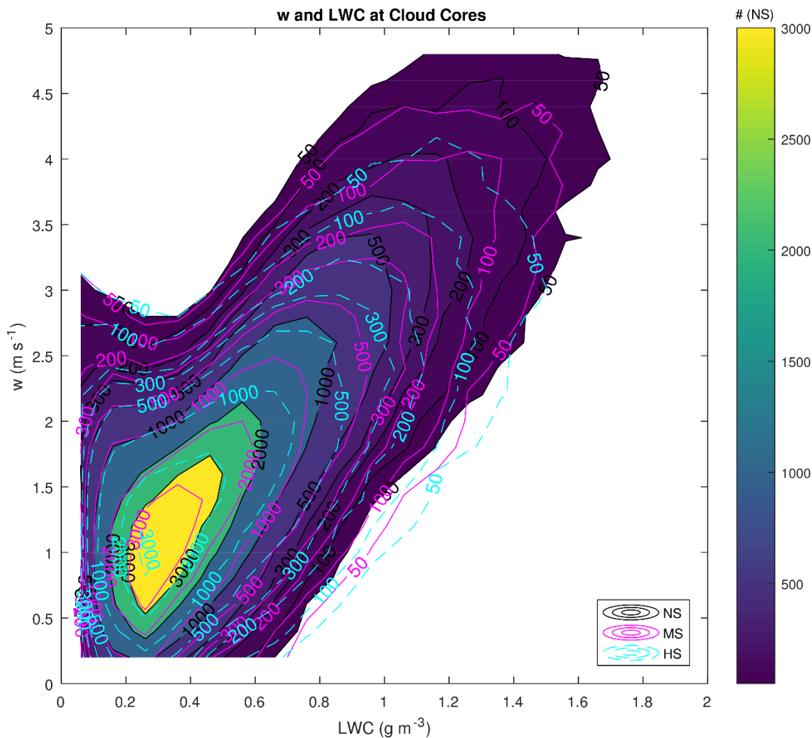
760 Figure 11: Distribution of the number of datapoints in the updraughts speed w – liquid water content LWC space for the cloud cores. The colours and the black continuous lines represent the NS run. The MS and HS runs are represented by continuous magenta and dashed cyan lines, respectively. The w interval is between 0.1 \text{ m s}^{-1} and 5 \text{ m s}^{-1} , with 0.2 \text{ m s}^{-1} bins. The LWC interval is between 0.01 \text{ g m}^{-3} and 2 \text{ g m}^{-3} , with 0.1 \text{ g m}^{-3} bins. The curves in this figure represent the datapoint numbers calculated for those bins.
