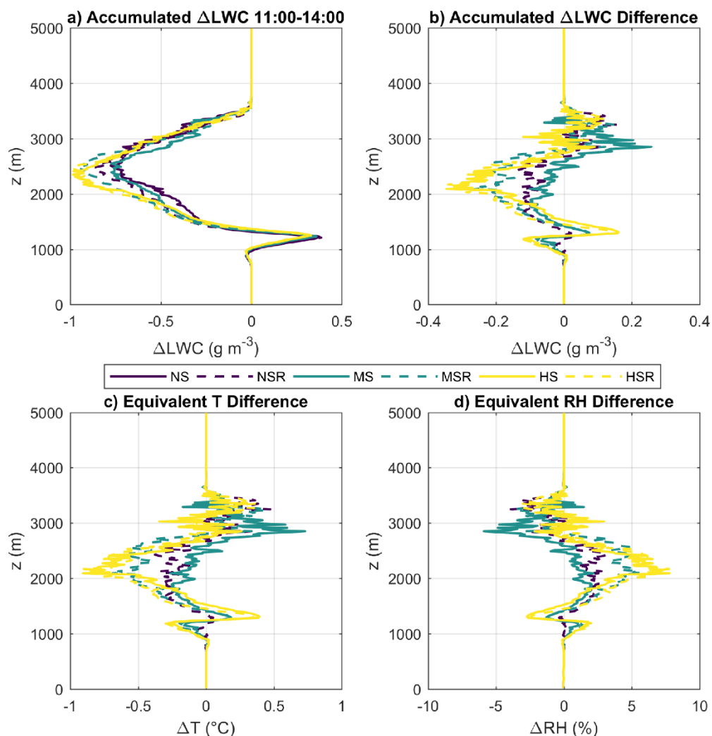
765 Figure 12: Average effect of the evaporation/condensation rates on the vertical temperature (T) and relative humidity (RH) profiles in the vicinity of clouds. Panel a) shows the time-integrated condensation/evaporation rates between 11:00 and 14:00 local time (i.e., the total water vapor converted to cloud liquid water or the reverse). Panel b) shows the same profiles, but as differences between the runs (having NS as reference). Panels c) and d) show the estimated T and RH differences as calculated from the curves of panel b). This estimate assumes L_v = 2.5 \times 10^6 \text{ J kg}^{-1} (latent heat of condensation) and c_p = 1005 \text{ J kg}^{-1} \text{ K}^{-1} (specific heat of air at constant pressure).
