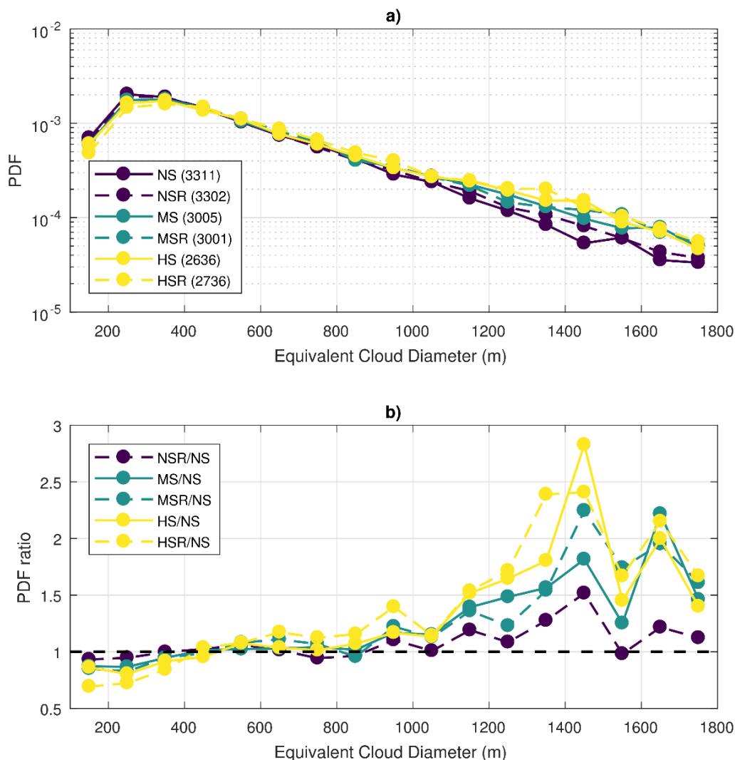
Figure 6: Probability density function (PDF) of equivalent cloud diameter. The equivalent diameter is calculated as the diameter of a circle having the same horizontal area as the tracked cloud shape. Panel a) shows the PDFs for all six simulations as function of the central diameter of every 100-m interval between 100 m and 1800 m. As such, the smallest trackable clouds (180 m) are in the first datapoint. The total number of clouds is shown in parenthesis in the legend of panel a). Panel b) shows the ratio of the PDFs, with the simulation NS as the reference. All datapoints represent at least about 50 clouds for statistical robustness.
