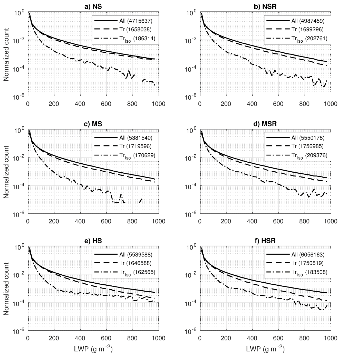
Figure 4: Normalized histograms of LWP for all six runs. The continuous black lines (“All” in the legend) represent the distribution for all pixels in the domain with LWP > 0.6 g m -2 . The dashed lines represent the distributions only for the pixels that are tracked by ForTraCC (“Tr” in the legend). The dot-dashed lines represent the distributions only for the pixels that are tracked by ForTraCC and for which no merger or split were detected (“Tr iso ” in the legend). Within the legend, the numbers in parentheses are the total number of pixels in each case. All 2-min output time steps between 11:00 and 18:00 local time are considered.
