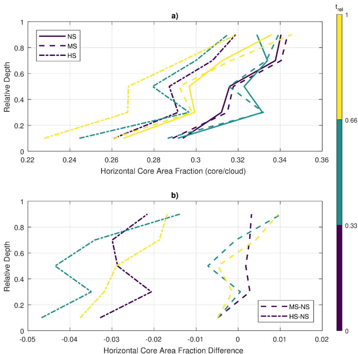
745 Figure 9: Similar to Figure 8, but the profiles represent the average core area fraction (i.e., the ratio of the core and cloud areas) in horizontal slices through the clouds. Panel a) shows the actual fraction values, while b) shows the differences between the MS/HS runs and NS. The standard deviation of the area fraction represents approximately 70% of the averages close to cloud base, decreasing to 50% close to cloud top.
