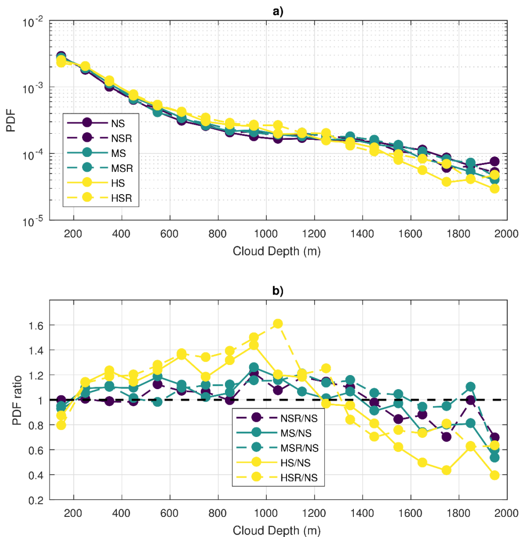
Figure 7: Same as Figure 6 but for cloud depth. Cloud depth is calculated as the height difference between cloud top and cloud base (using the maximum and minimum height with LWC > 0.01 \text{ g m}^{-3} , respectively).
