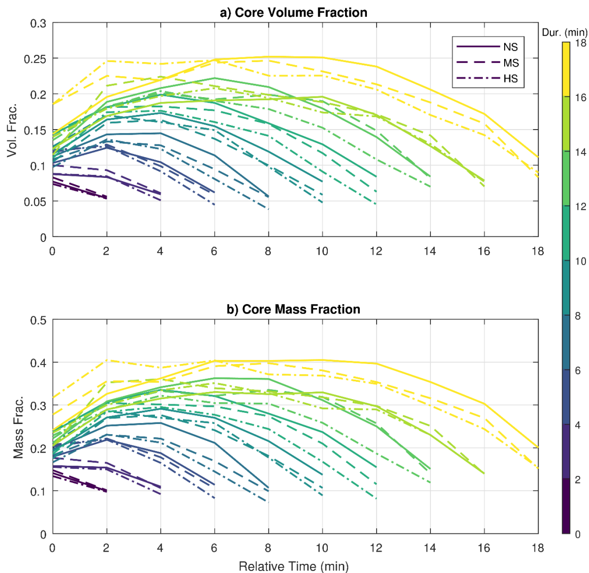
750 Figure 10: Cloud core volume and mass fraction as a function of cloud life cycle and total duration. The fractions are obtained by the ratio of the total core volume or mass by the total cloud volume or mass. The total duration is given by the number of time steps representative of each tracked cloud. Clouds only present in two time steps are assumed to have 2-min duration time, three time steps equating to 4-min duration and so on. The volume and mass fractions standard deviations are relatively similar for the time steps of clouds sharing the same duration. For the volume fraction, the standard deviations reach up to approximately 0.15. 755 For mass fractions, they have values up to 0.22 approximately.
