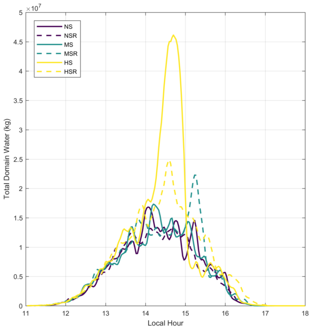
725 Figure 5: Time series of the total domain water (kg), calculated as the 3D integration of the cloud and rain liquid water contents over the entire simulation domain.
