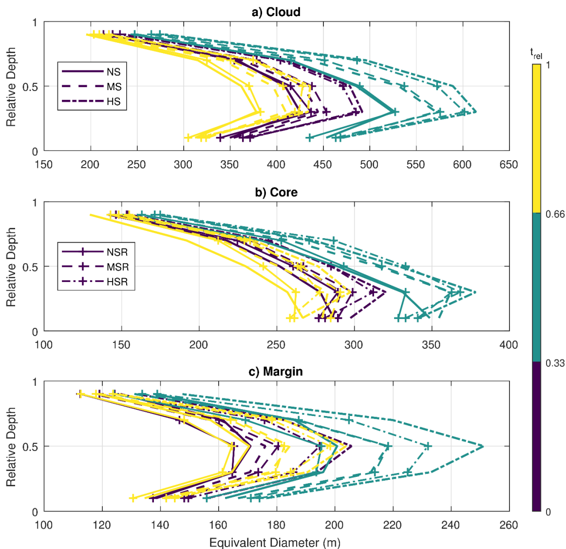
Figure 8: Averaged dimensions of the a) clouds, b) cloud cores and c) cloud margins as a function of the cloud life cycle and relative depth. The relative depth is a normalized height based on cloud base and cloud top. Values of 0 equate to the cloud base, while 1 represents cloud top. We use 5 relative depth intervals of 0.2, plotting the datapoints in the centre of them. The cloud life cycle is also normalized ( t_{rel} , in colours), being 0 at the first initial detection by ForTraCC and 1 at its latest time step. We set 3 life cycle intervals, representing initial, mature, and dissipating stages. The standard deviations are omitted for figure clarity, but they represent approximately 80% of the averages in the depth interval closest to cloud base, decreasing to about 50% close to cloud top.
