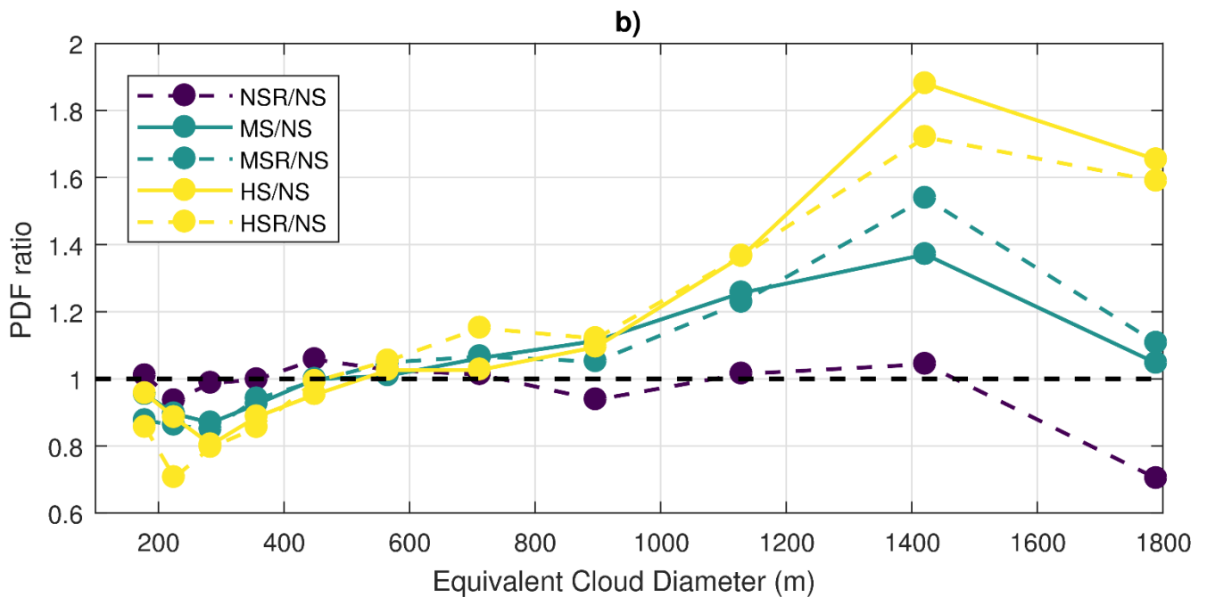
825 Figure 8: Probability density function (PDF) of equivalent cloud diameter. The equivalent diameter is calculated as the diameter of a circle having the same horizontal area as the tracked cloud shape. Panel a) shows the PDFs for all six simulations as function of the central diameter of every 100-m interval between 100 m and 1800 m. As such, the smallest trackable clouds (180 m) are in the first datapoint. The total number of clouds is shown in parenthesis in the legend of panel a). Panel b) shows the ratio of the PDFs, with the simulation NS as the reference. All datapoints represent at least about 50 clouds for statistical robustness.
