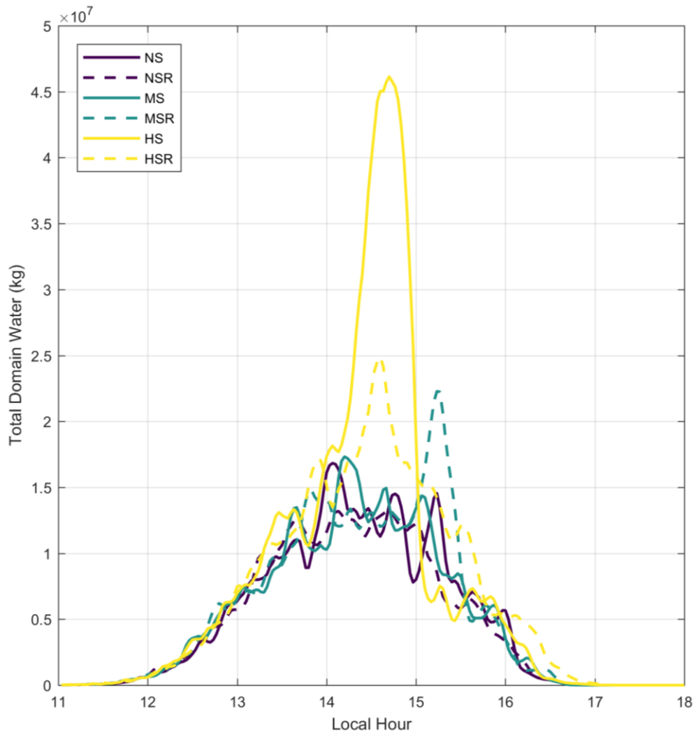
820 Figure 7: Time series of the total domain water (kg), calculated as the 3D integration of the cloud and rain liquid water contents over the entire simulation domain.
