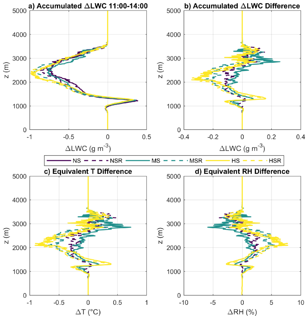
865 Figure 14: Average effect of the evaporation/condensation rates on the vertical temperature (T) and relative humidity (RH) profiles in the vicinity of clouds. Panel a) shows the time-integrated condensation/evaporation rates between 11:00 and 14:00 local time (i.e., the total water vapor converted to cloud liquid water or the reverse). Panel b) shows the same profiles, but as differences between the runs (having NS as reference). Panels c) and d) show the estimated T and RH differences as calculated from the curves of panel b). This estimate assumes L_v = 2.5 \times 10^6 \text{ J kg}^{-1} (latent heat of condensation) and c_p = 1005 \text{ J kg}^{-1} \text{ K}^{-1} (specific heat of air at constant pressure).
