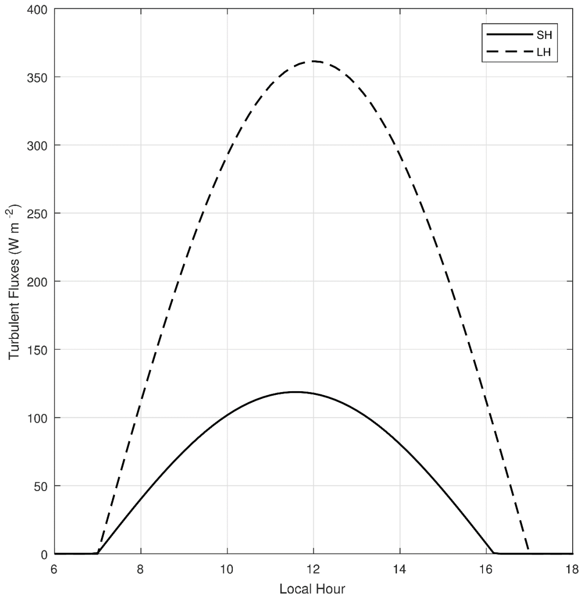
785 Figure 1: Prescribed surface turbulent fluxes of all DALES simulations performed in this study. SH and LH are the sensible and latent heat fluxes, respectively. The Bowen ratio SH/LH is mostly between 0.1 and 0.4, consistent with tropical rainforest environment.
