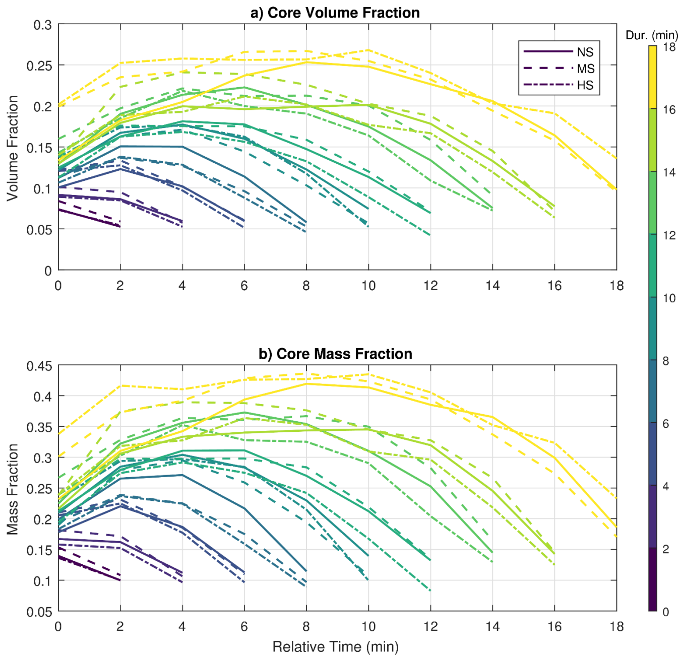
850 Figure 12: Cloud core volume and mass fraction as a function of cloud life cycle and total duration. The fractions are obtained by the ratio of the total core volume or mass by the total cloud volume or mass. The total duration is given by the number of time steps representative of each tracked cloud. Clouds only present in two time steps are assumed to have 2-min duration time, three time steps equating to 4-min duration and so on. The volume and mass fractions standard deviations are relatively similar for the time steps of clouds sharing the same duration. For the volume fraction, the standard deviations reach up to approximately 0.15. For mass fractions, they have values up to 0.22 approximately.
