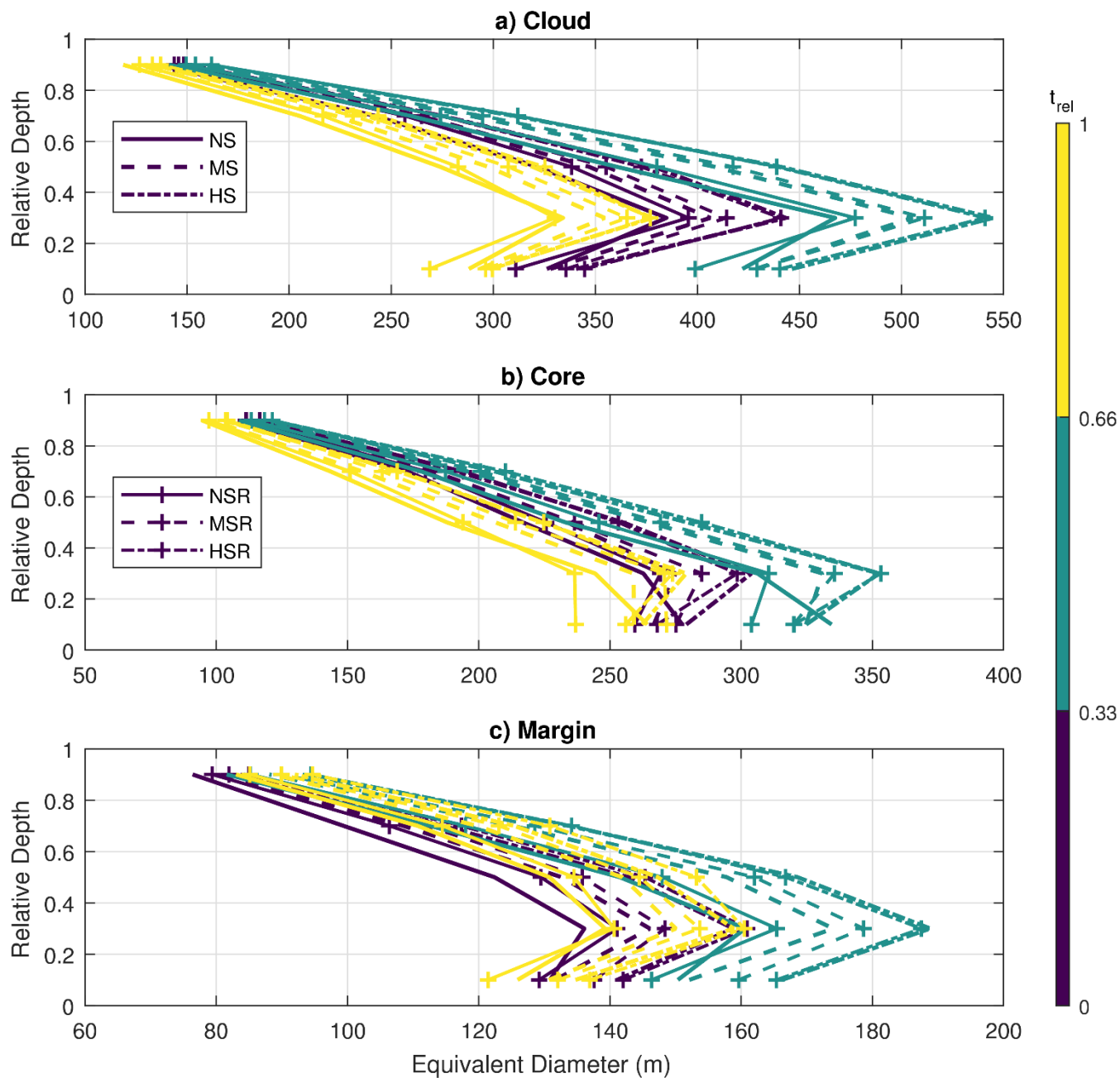
835 Figure 10: Averaged dimensions of the a) clouds, b) cloud cores and c) cloud margins as a function of the cloud life cycle and 840 relative depth. The relative depth is a normalized height based on cloud base and cloud top. Values of 0 equate to the cloud base, while 1 represents cloud top. We use 5 relative depth intervals of 0.2, plotting the datapoints in the centre of them. The cloud life cycle is also normalized ( t_{rel} , in colours), being 0 at the first initial detection by ForTraCC and 1 at its latest time step. We set 3 life cycle intervals, representing initial, mature, and dissipating stages. The standard deviations are omitted for figure clarity, but they represent approximately 80% of the averages in the depth interval closest to cloud base, decreasing to about 50% close to cloud top.
