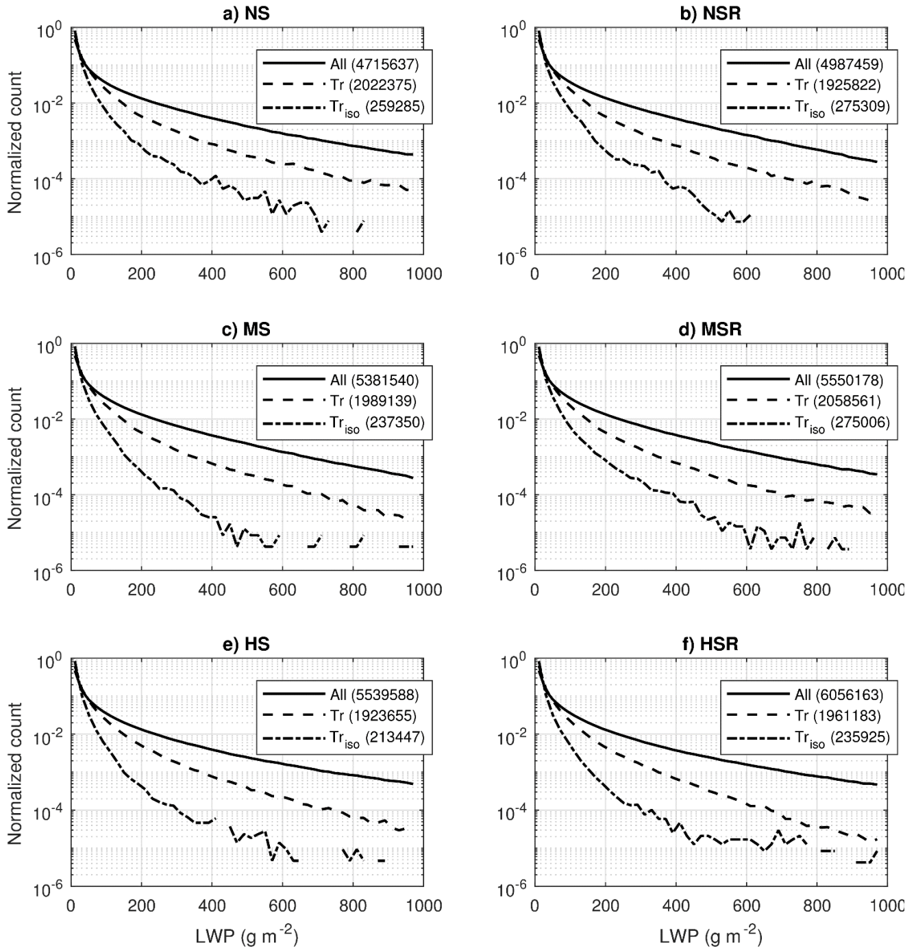
Figure 6: Normalized histograms of LWP for all six runs. The continuous black lines (“All” in the legend) represent the distribution for all pixels in the domain with LWP > 0.6 \text{g m}^{-2} . The dashed lines represent the distributions only for the pixels that are tracked by ForTraCC (“Tr” in the legend). The dot-dashed lines represent the distributions only for the pixels that are tracked by ForTraCC and for which no merger or split were detected (“Tr iso ” in the legend). Within the legend, the numbers in parentheses are the total number of pixels in each case. All 2-min output time steps between 11:00 and 18:00 local time are considered.
