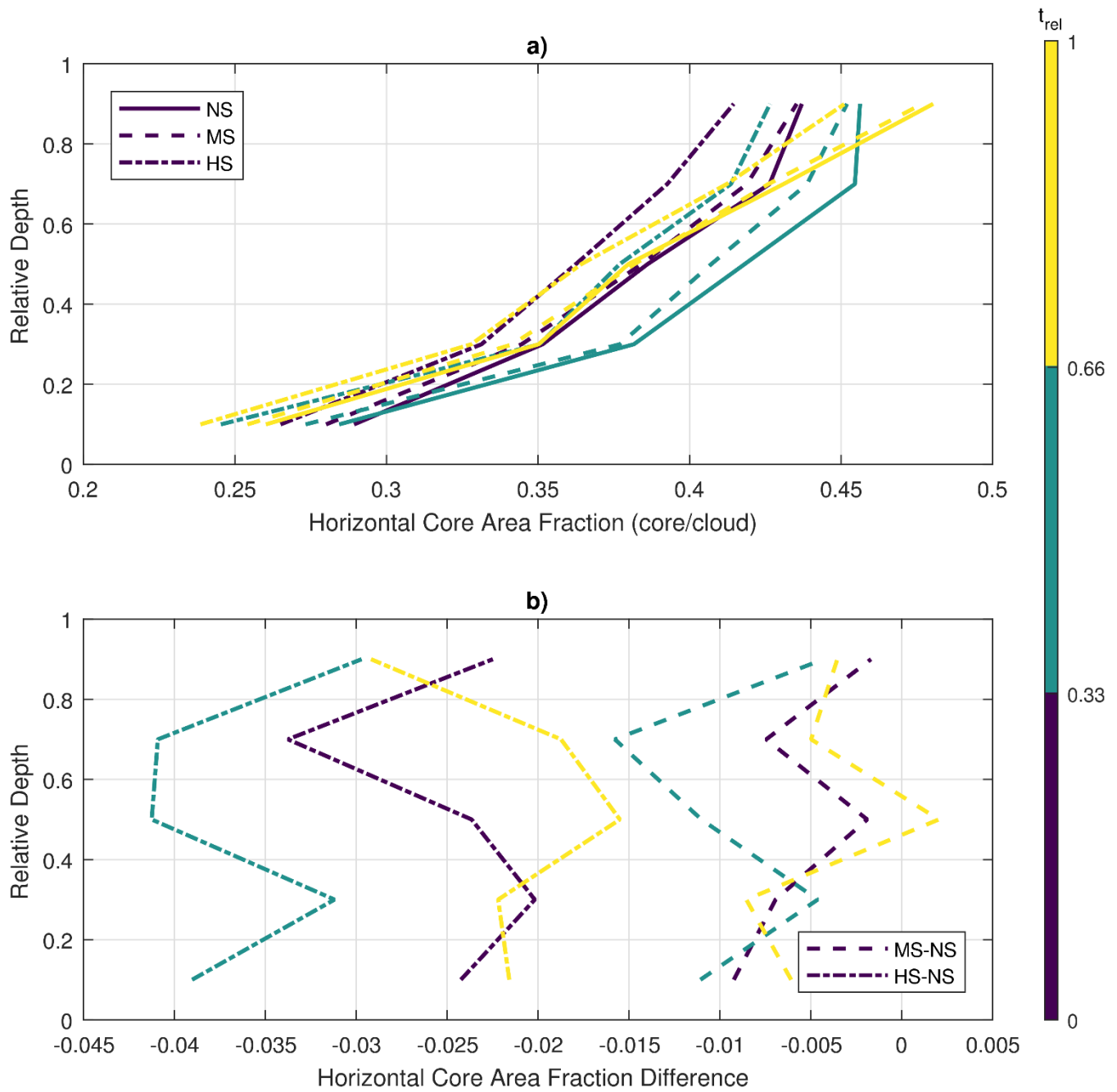
845 Figure 11: Similar to Figure 8, but the profiles represent the average core area fraction (i.e., the ratio of the core and cloud areas) in horizontal slices through the clouds. Panel a) shows the actual fraction values, while b) shows the differences between the MS/HS runs and NS. The standard deviation of the area fraction represents approximately 70% of the averages close to cloud base, decreasing to 50% close to cloud top.
