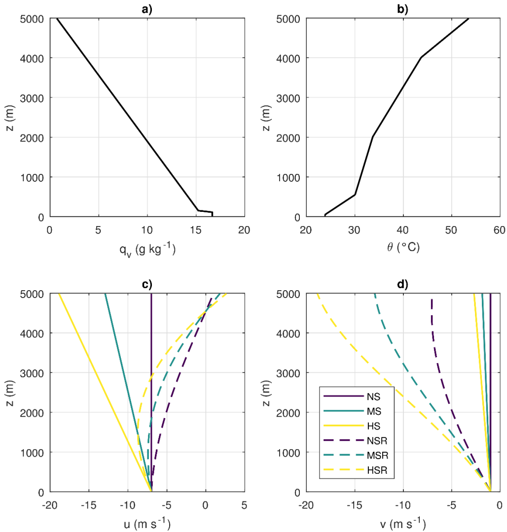
790 Figure 2: Input profiles of a) water vapor specific humidity q_v , b) potential temperature \theta , c) zonal wind component u and d) meridional wind component v . The large-scale wind forcing is the same as the initial conditions of the respective runs, remaining unchanged throughout the whole simulations. The initial profiles of both q_v and \theta are the same for every run, the only difference being the vertical wind variability. Three levels of wind speed shear are defined: no wind speed shear (NS), moderate wind speed shear (MS) and high wind speed shear (HS). A counterclockwise rotation of 90^{\circ} in wind direction between 0 km and 5 km is applied in the NSR, MSR and HSR runs, which have the same wind speed shear as NS, MS and HS, respectively.
