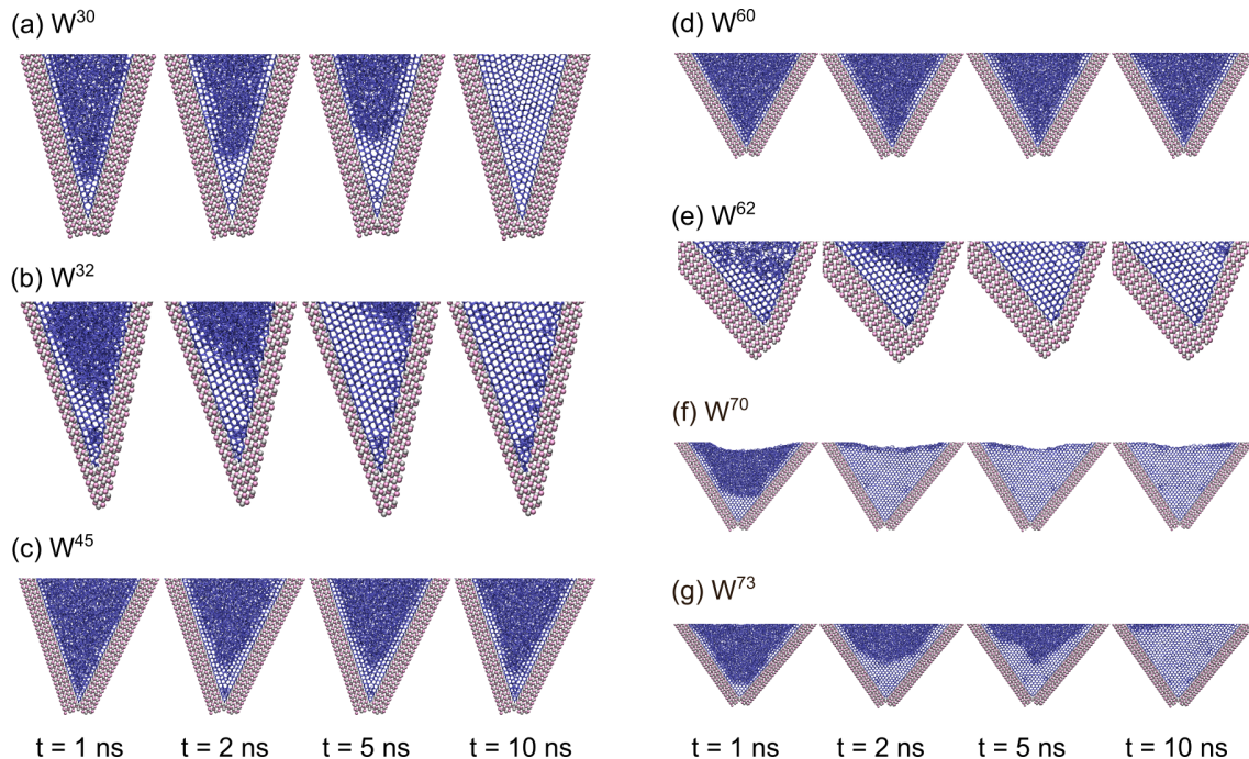
Figure 6. Simulation snapshot details of ice growth at times t = 1, 2, 5, 10 ns in wedge systems (a) W^{30} , (b) W^{32} , (c) W^{45} , (d) W^{60} , (e) W^{62} , (f) W^{70} , and (g) W^{73} , using the mW model. Ag and I are colored in silver and pink, respectively, and the hydrogen bond network between mW water molecules is indicated by blue sticks.
