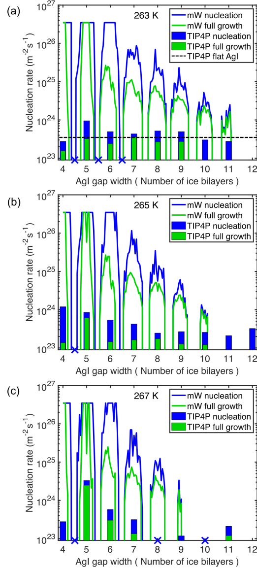
Figure 11: Nucleation rates in AgI slit simulations and inverse of time at which full ice growth in the AgI slit is observed, at (a) 263 K, (b) 265 K, and (c) 267 K, with mW model (continuous line) and TIP4P/Ice model (bar plot). Blue crosses indicate TIP4P/Ice simulations in which nucleation was not observed. The nucleation rate at 263 K on the flat AgI(0001) surface using the TIP4P/Ice model is indicated by the dashed black line in panel (a).
