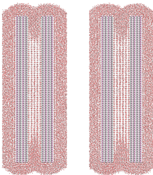
Figure 1: Snapshots of the final configurations of ice nucleation simulations at T = 263 K using the TIP4P/Ice water model in AgI slit systems with a gap width of 5 (left) and 6 (right) ice bilayers. Ag and I are shown in silver and pink, respectively, and water molecules are shown as red and white sticks. In both systems, ice cannot grow close to the slab edges.
