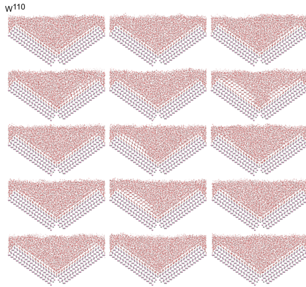
Figure 8: Simulation snapshot details of the last frames of 15 independent simulations of wedge systems W^{110} at T = 263 K using the TIP4P/Ice model. Ag and I are shown in silver and pink, respectively, and water molecules are shown as red and white sticks.
