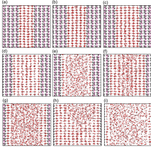
Figure 3: Snapshot details of the last frame of TIP4P/Ice simulations at 267 K for AgI slit systems with gap widths of (a) 4 ice bilayers, (b) 5 ice bilayers, (c) 6 ice bilayers, (d) 7 ice bilayers, (e) 8 ice bilayers, (f) 9 ice bilayers, (g) 10 ice bilayers, (h) 11 ice bilayers and (i) 12 ice bilayers. Ag and I are shown in silver and pink, respectively, and water molecules are shown as red and white sticks.
