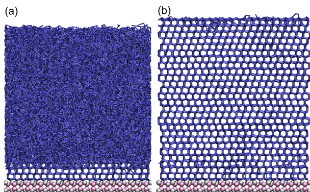
Figure 7: Simulation snapshot details of maximum ice growth observed in ice nucleation simulations on the flat AgI(0001) surface using the mW model (a) at T = 263 K in 60 ns, and (b) at 262 K in 20 ns. Ag and I are colored in silver and pink, respectively, and the hydrogen bond network between mW water molecules is indicated by blue sticks.
