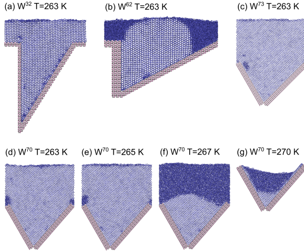
Figure 10: Simulations of ice outgrowing wedge systems at T = 263 K, and the effect of temperature on the ice growth in the W^{70} system using the mW model. (a) W^{32} and (b) W^{62} at T = 263 K, (c) W^{73} at T = 263 K, (d) W^{70} at T = 263 K, (e) W^{70} at T = 265 K, (f) W^{70} at T = 267 K, and (g) W^{70} at T = 270 K. Ag and I ions are shown in silver and pink, respectively, and the hydrogen bond network between mW water molecules is shown by blue sticks.
