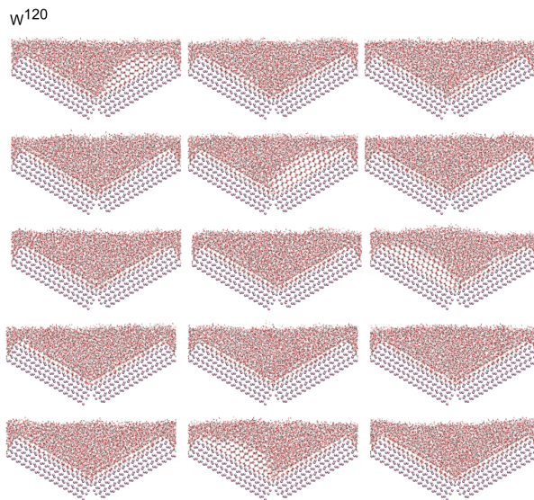
Figure 9: Simulation snapshot details of the last frames of 15 independent simulations of wedge systems W^{120} at T = 263 K using the TIP4P/Ice model. Ag and I are shown in silver and pink, respectively, and water molecules are shown as red and white sticks.
