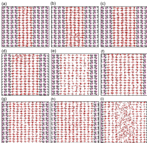
Figure 2: Snapshot details of the last frame of TIP4P/Ice simulations at 265 K for AgI slit systems with gap widths of (a) 4 ice bilayers, (b) 5 ice bilayers, (c) 6 ice bilayers, (d) 7 ice bilayers, (e) 8 ice bilayers, (f) 9 ice bilayers, (g) 10 ice bilayers, (h) 11 ice bilayers and (i) 12 ice bilayers. Ag and I are shown in silver and pink, respectively, and water molecules are shown as red and white sticks.
