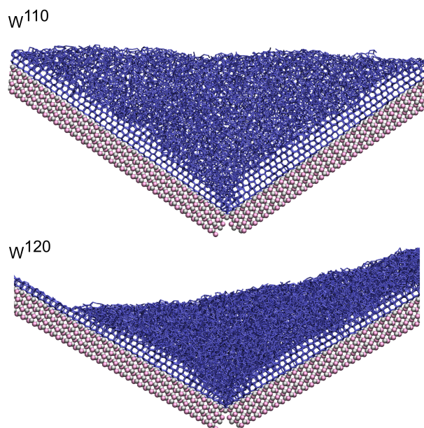
Figure 6: Simulation snapshot details of the last frame ( t = 150 ns) for wedge systems W^{110} (top) and W^{120} (bottom) at T = 263 K, using the mW model. Ag and I are colored in silver and pink, respectively, and the hydrogen bond network between mW water molecules is indicated by blue sticks.
