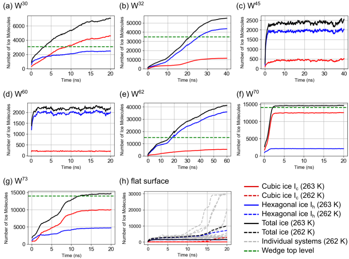
Figure 4: Time evolution of the average number of mW water classified as cubic or hexagonal ice and their sum in wedge systems with different angles at T = 263 K (a-g) and on the flat AgI(0001) surface at T = 263 K and 262 K (h). Top level indicates when the ice front has grown up to the top of the AgI wedge structure. In some systems, ice growth out of the wedge can be observed.
