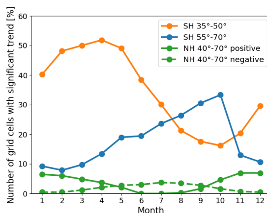
Figure 8. Number of grid cells indicating a significant trend as a function of month for the latitude bands 40^{\circ} – 70^{\circ} N (green), 35^{\circ} – 50^{\circ} S (orange), and 55^{\circ} – 70^{\circ} S (blue). The number is provided in percent of the total number of grid cells in the respective band. For the Northern Hemisphere (green) a division between significant positive (solid curve) and significant negative trends (dashed curve) is made.
