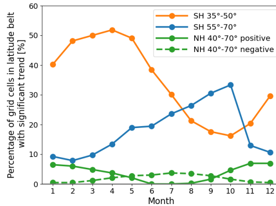
Figure 8. Number-Percentage of grid cells indicating a significant trend as a function of month for the latitude bands 40°–70°N (green), 35°–50°S (orange), and 55°–70°S (blue). The number is provided in percent of the total number of grid cells in the respective band. For the Northern Hemisphere (green) a division between significant positive (solid curve) and significant negative trends (dashed curve) is made.
