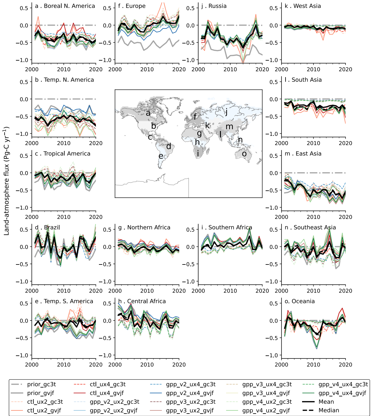
Figure 6. Interannual variation of terrestrial land \text{CO}_2 fluxes derived from 16 sets of inversion. The variations are shown for 15 aggregated regions shown in the map. The negative values are counted as \text{CO}_2 removals from the atmosphere, while \text{CO}_2 emissions are counted positively.
