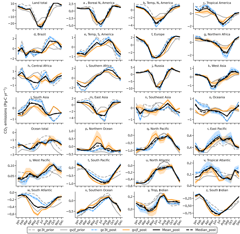
Figure 9. Seasonal variations in monthly-mean CO 2 fluxes at regional scales over 15 lands (upper four rows) and 11 oceans (lower three rows) regions, along with global land and ocean totals. We prepare the average (2001 - 2020) separately for inversion ensemble cases based on “gc3t” (broken line) and “gvjf” (solid line) prior. The shade around means shows \pm 1\sigma
