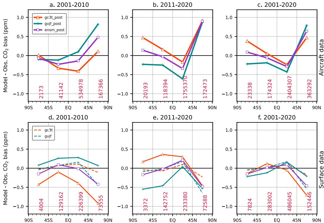
Figure 12. Evaluation of the atmospheric inversion products (solid lines; legends in panel a). The mean of model-observation differences is shown for four latitude bands of 45° intervals in three time periods: (a,d) 2001–2010, (b,e) 2011–2020, (c,f) 2001–2020. The simulations from three inversion cases are compared to independent CO 2 measurements made onboard aircraft (a-c: top row) over various parts of the world between 2 and 8 km above sea level. Bottom row shows the model-observation differences for 50 surface sites that are used in the inversion (d-f), and mismatches between the a posteriori model (as obtained after optimising regional sources by inversion) and CO 2 data (broken lines; legends in panel d). Land and ocean data are used without distinction. The number in each panel shows the total number of data points used for computing bias for each latitude bin. The observation data are taken from obspack_co2_1_GLOBALVIEWplus_v6.1 (Schuldt et al., 2021).
