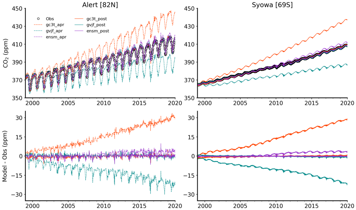
Figure 2. Time series of observed and model CO 2 time series for two a priori (apr) simulation cases (gc3t and gvjf), and posterior (post) flux simulation cases using control MDU and PFU case ux4 (top row). Results for the mean of two a priori flux cases and ensemble mean inversion case are also shown. The model-observation differences are shown in the bottom row. Results are shown for two sites, Alert (82°N, 63°W; measurements by Environment Canada), and Syowa (69°S, 40°E; measurements by Tohoku University/National Institute of Polar Research).
