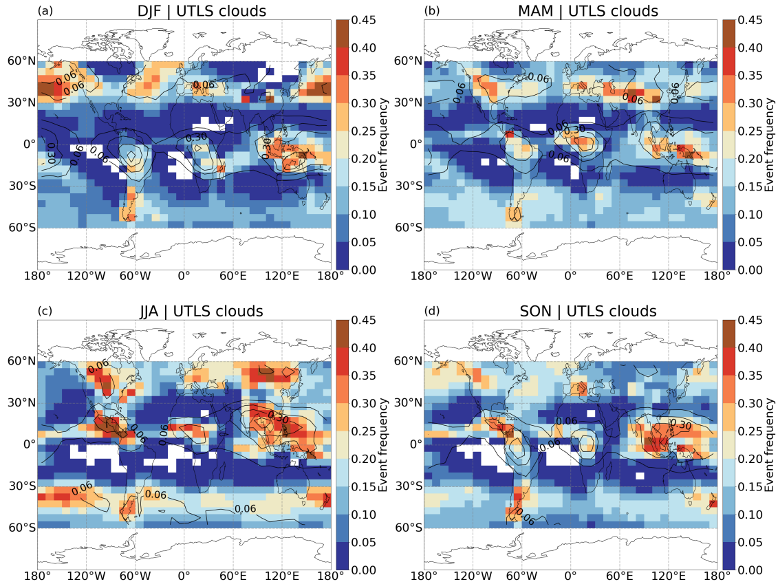
Figure 5. Seasonal event frequency of UTLS clouds derived from AIRS during 2007-2019. Occurrence frequencies of SICs (data in Figure 1a-d) are shown in black contours with the interval of 0.12.
