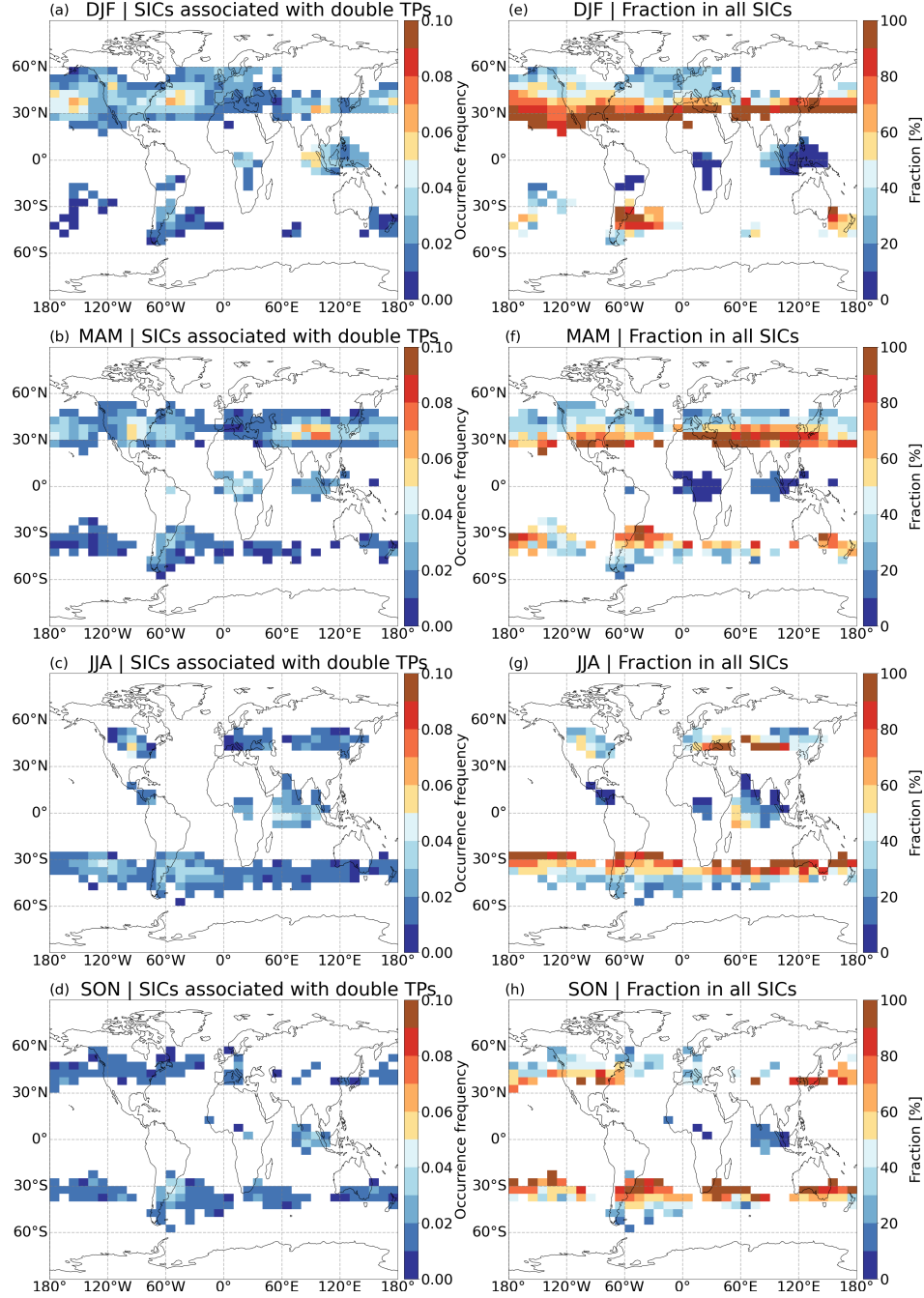
Figure 3. Occurrence frequencies of SICs associated with double tropopause with respect to all profiles (a-d) and the fraction of SICs associated with double tropopause to total SICs (e-h).
