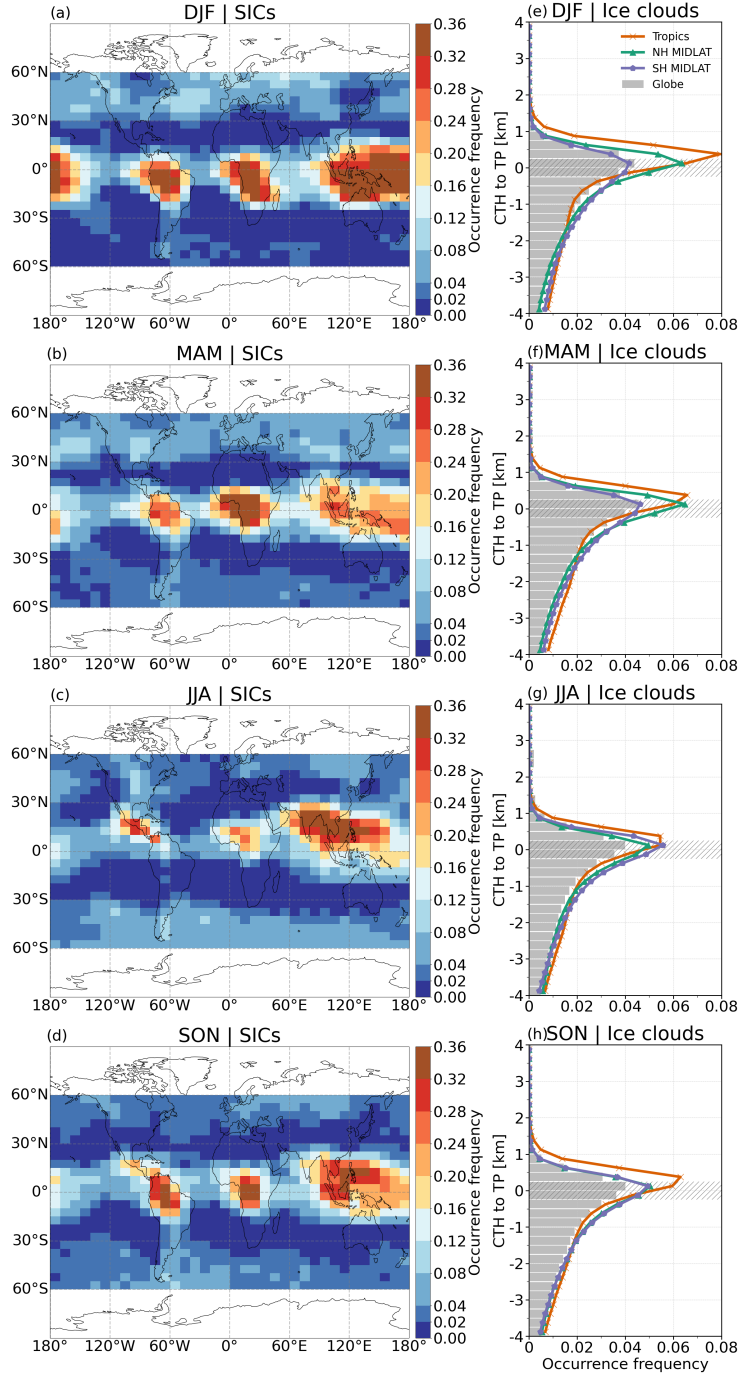
Figure 1. Occurrence frequencies of SICs on a 5^\circ \times 10^\circ (latitude \times longitude) grid (a-d) and occurrence frequencies of ice cloud top heights (CTHs) in the altitude range from -4 to 4 km with respect to the first thermal tropopause (e-h) in DJF, MAM, JJA and SON from CALIPSO measurements. In e-h, the data are shown as zonal averages, globally (gray bars), for the tropics ( 20^\circ\text{S} - 20^\circ\text{N} , orange lines) and midlatitudes ( 40^\circ - 60^\circ , green lines for NH and purple lines for SH). The hatched areas are tropopause uncertainties of \pm 250 m.
