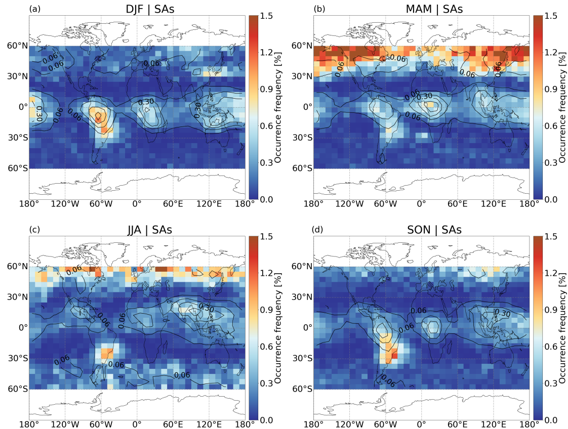
Figure 8. Seasonal occurrence frequency of stratospheric aerosols from CALIPSO during 2007-2019. Black contours are occurrence frequencies of SICs shown in Figure 1a-d.
