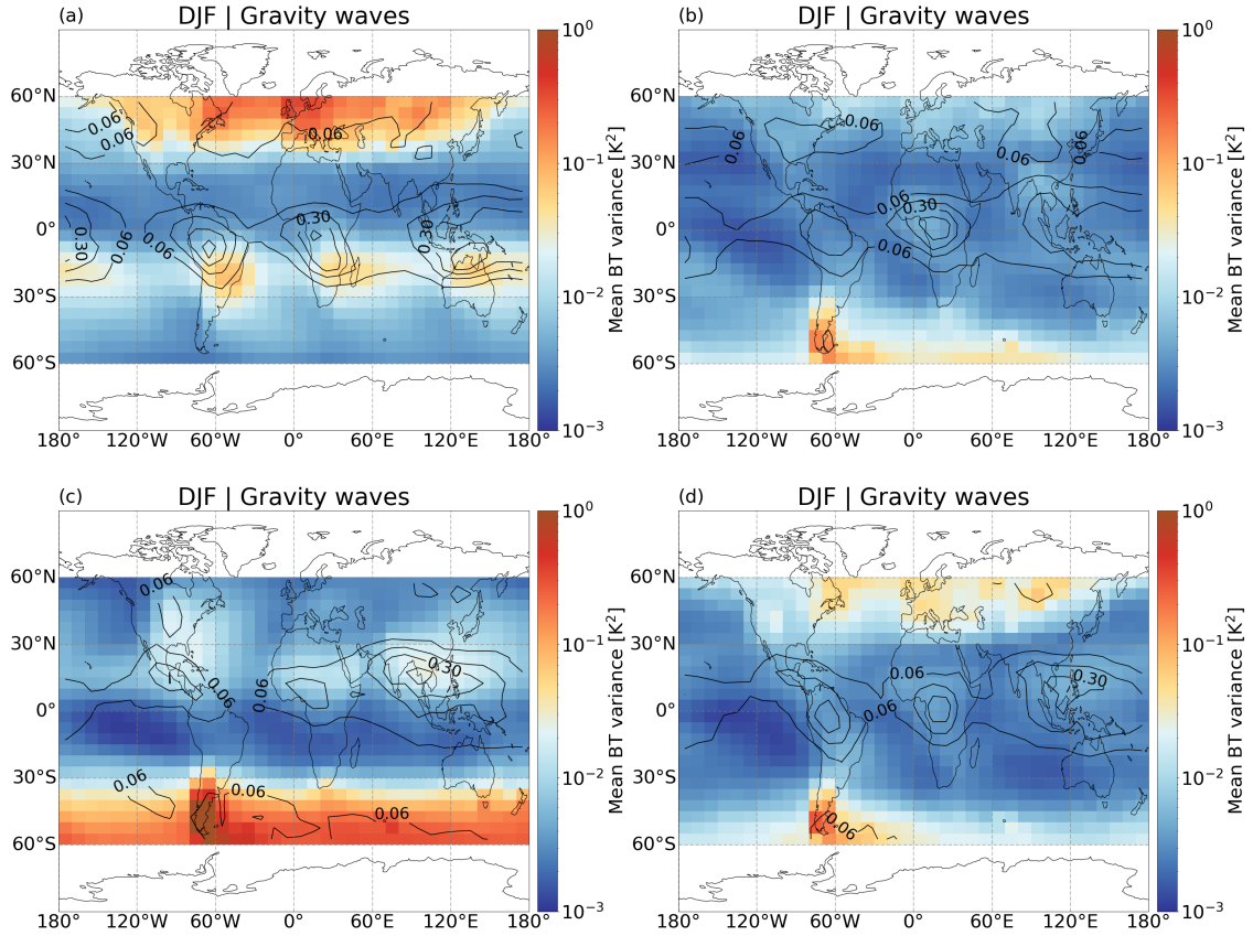
Figure 7. Mean brightness temperature variance at 4.3 \mu\text{m} from AIRS measurements, which correlates with the amplitude of gravity waves. Black contours are occurrence frequencies of SICs shown in Figure 1a-d.
