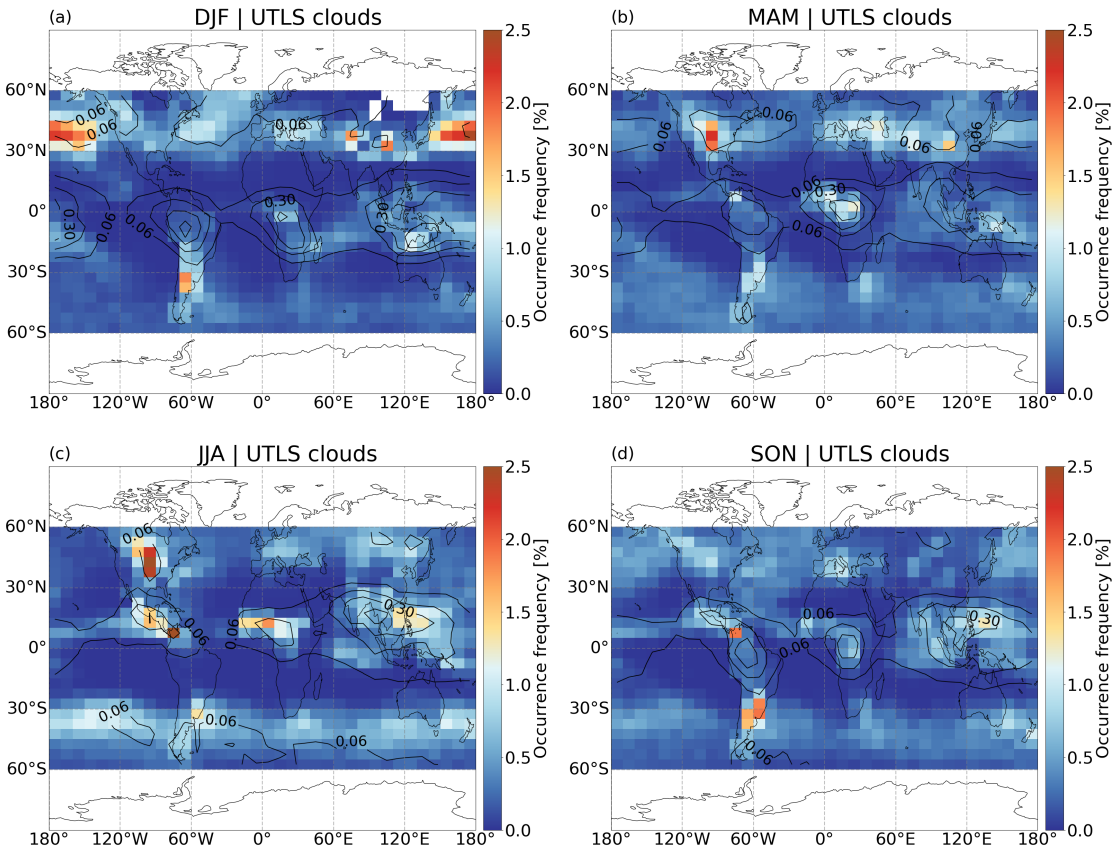
Figure B1. Seasonal mean occurrence frequency of UTLS clouds derived from AIRS measurements during 2007-2019. Black contours are occurrence frequencies of SICs shown in Figure 1a-d.
