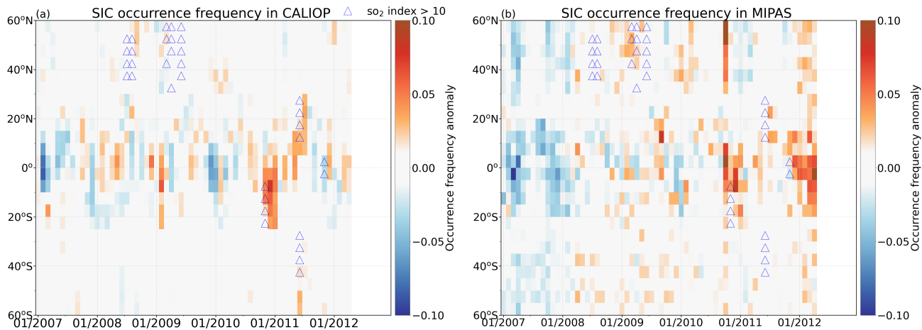
Figure 12. Monthly anomalies of SIC occurrence frequencies from CALIOP (a) and MIPAS (b) measurements. Blue triangles are data with SI > 10 K derived from AIRS observations.
