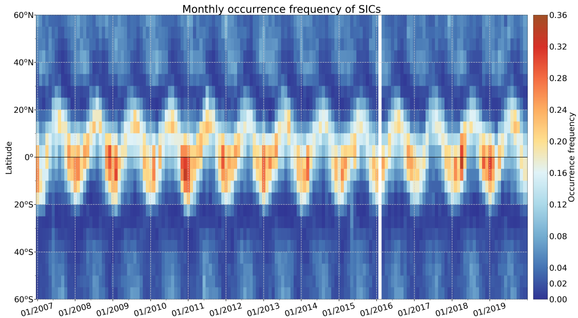
Figure 2. Monthly occurrence frequencies of SICs in latitude band of 5^\circ from 2007 to 2019.
