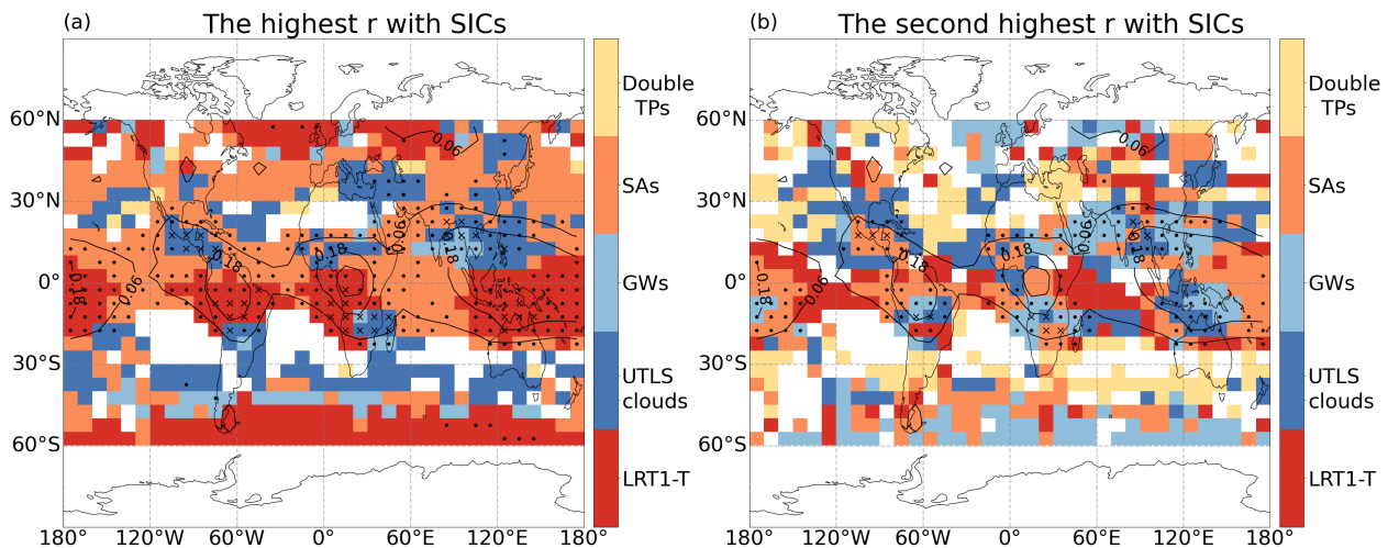
Figure 10. The highest and second-highest correlation coefficients between SIC occurrence frequency and all processes (LRT1-T, UTLS clouds, gravity waves (GWs), stratospheric aerosols (SAs) and double tropopauses (Double TPs)). Only grid boxes with absolute r \geq 0.3 are presented, and grid boxes filled with '.' means 0.6 \leq \text{absolute } r < 0.8 , 'x' means 0.8 \leq \text{absolute } r < 1.0 . Black contours are occurrence frequencies of SICs shown in Figure 1a-d.
