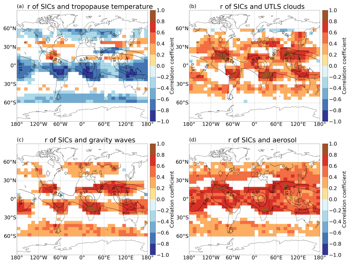
Figure 9. Spearman correlation coefficients of SIC occurrence frequency and the first tropopause temperature, UTLS cloud event frequency, gravity waves, and stratospheric aerosol occurrence frequency from 2007 to 2019 with grid cell in 5^\circ latitude \times 10^\circ longitude. Only grid boxes with SIC occurrence frequency > 0.02 and \geq 80 data points in each grid box and at 99 % significance level are presented. Occurrence frequency of SICs shown in black contours with an interval of 0.12 are data presented in Figure 1a-d.
