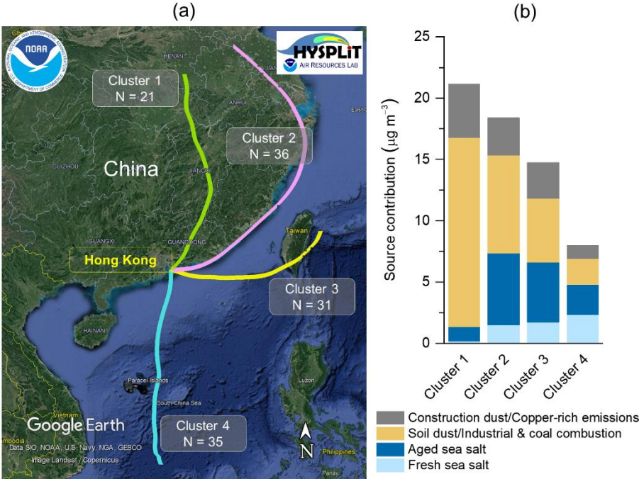
Figure 3. Source contributions to PM_{coarse} grouped by air masses associated with different back-trajectory clusters. Past 48-hour backward trajectory of air mass reaching Hong Kong (height = 300 m above ground level) during the end of each sampling event at midnight are considered. Figure (a) shows the mean trajectories of the four clustered trajectories (Map data: Google Earth, Data SIO, NOAA, U.S. Navy, NGA, GEBCO, Image Landsat/Copernicus) while Fig. (b) shows the source contributions for the corresponding clusters.
