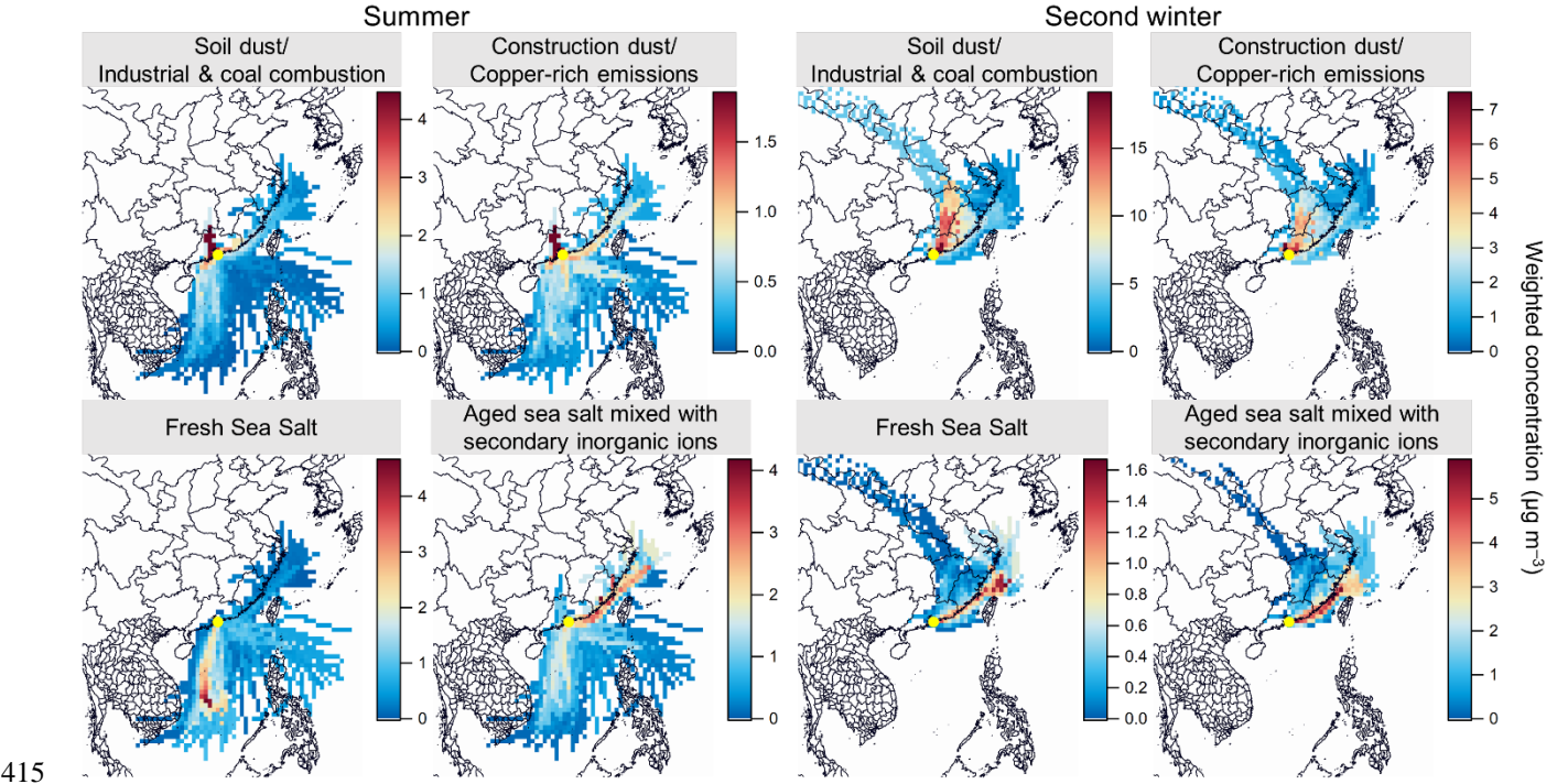
415 Figure 5. Concentration-Weighted Trajectory results for individual PM_{coarse} contributing sources in summer and the second winter. The location of the receptor site (Hong Kong) is represented by the yellow marker. The results for the other seasons are provided in Fig. S7 in the Supplement.
