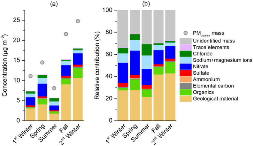
Figure 1. Seasonal variations in concentration and composition of \text{PM}_{\text{coarse}} observed at the Tuen Mun Air Quality Monitoring Station in Hong Kong. Figure (a) and (b) show the results in absolute concentration and relative contribution, respectively.
