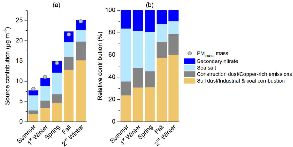
Figure 4. Source contributions to PM coarse during the study period. Figure (a) shows the results in \mu\text{g m}^{-3} while Fig. (b) shows the results in percentage share. The circle markers on the left figure represent the PM coarse concentration measured by gravimetric analysis.
