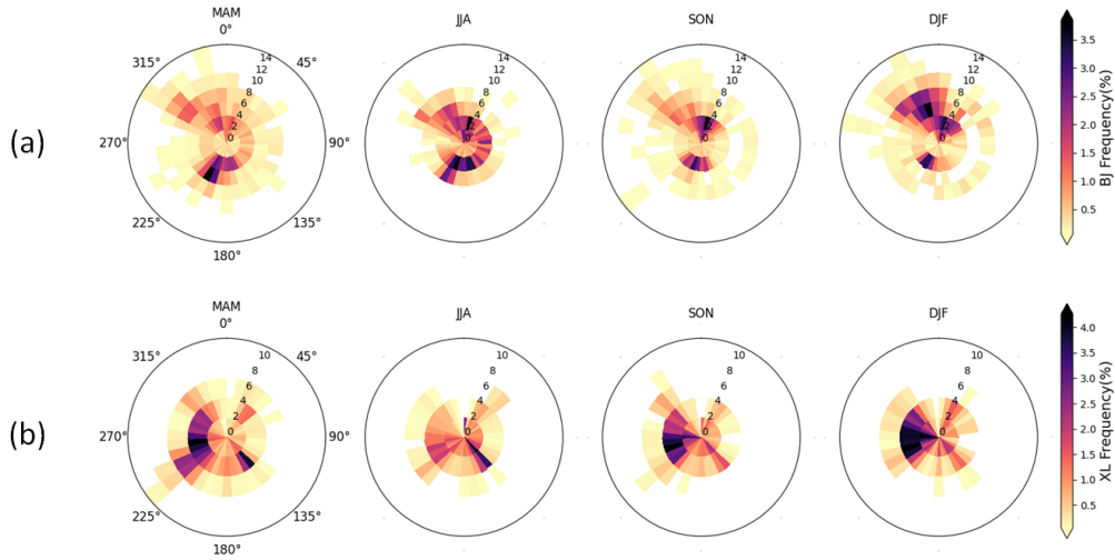
Figure 3. Wind frequency as a function of wind speed ( \text{m.s}^{-1} ) and wind direction ( ^{\circ} ) in each season spring (MAM) , summer (JJA) , autumn (SON) and winter (DJF) at BJ (a) and XL (b) from October 2018 to September 2019.
