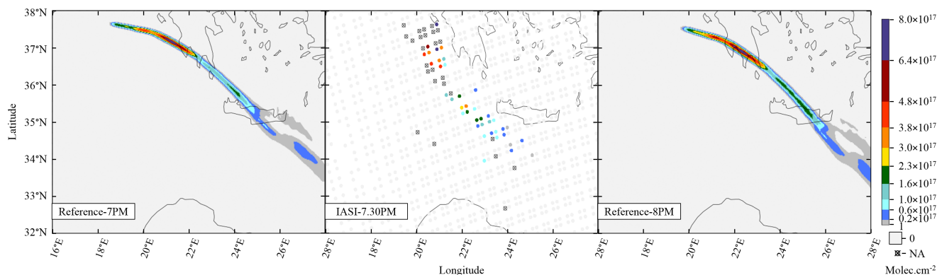
Figure 2. Columns of \text{SO}_2 from CHIMERE simulations and IASI measurements. IASI NAs data are shown as a crossed circle. Null values are shown in light gray. IASI sounding corresponds to 7.30PM UTC (center). CHIMERE Reference simulation is displayed for 7PM (left) and 8PM UTC (right).
