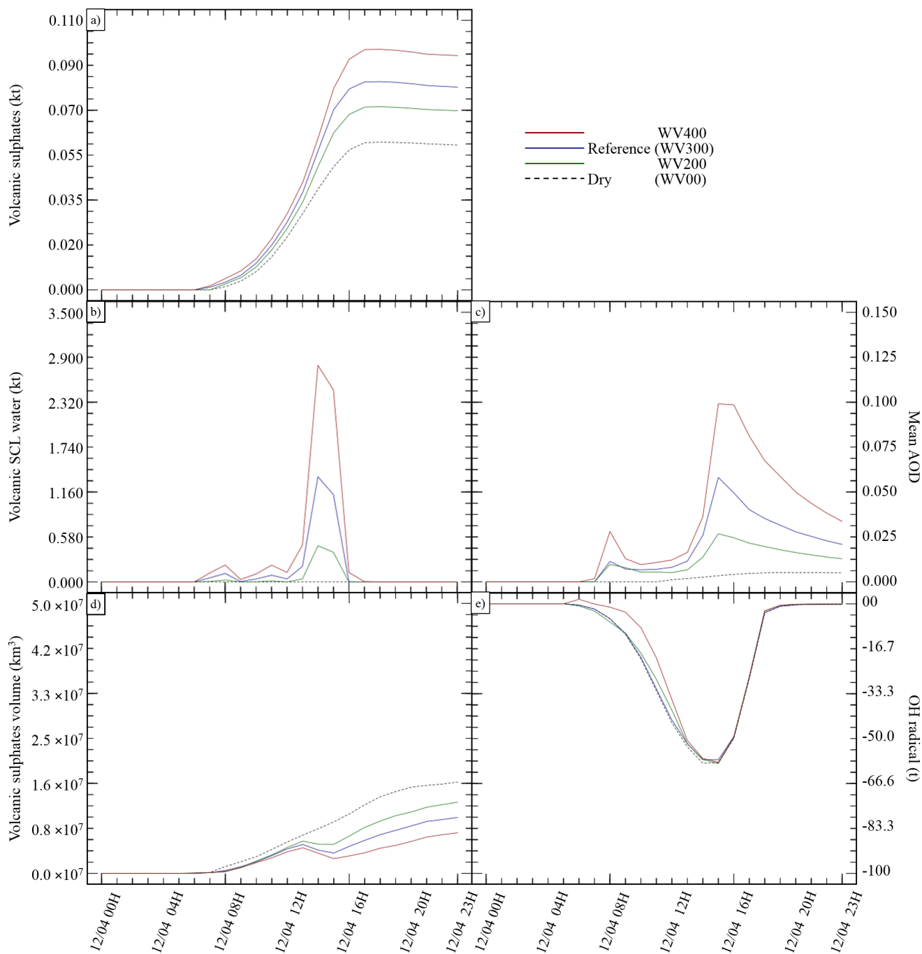
Figure 4. Sensitivity tests on vertical transport schemes. a) \text{SO}_{4(\text{p})}^{2-} (kt), b) SCLW (kt), c) AOD for plume \subset 25 % of \text{SO}_{4(\text{p})}^{2-} mass, d) Minimum volume ( \text{km}^3 ) \subset 25 % of \text{SO}_{4(\text{p})}^{2-} mass, e) OH radical (t).
