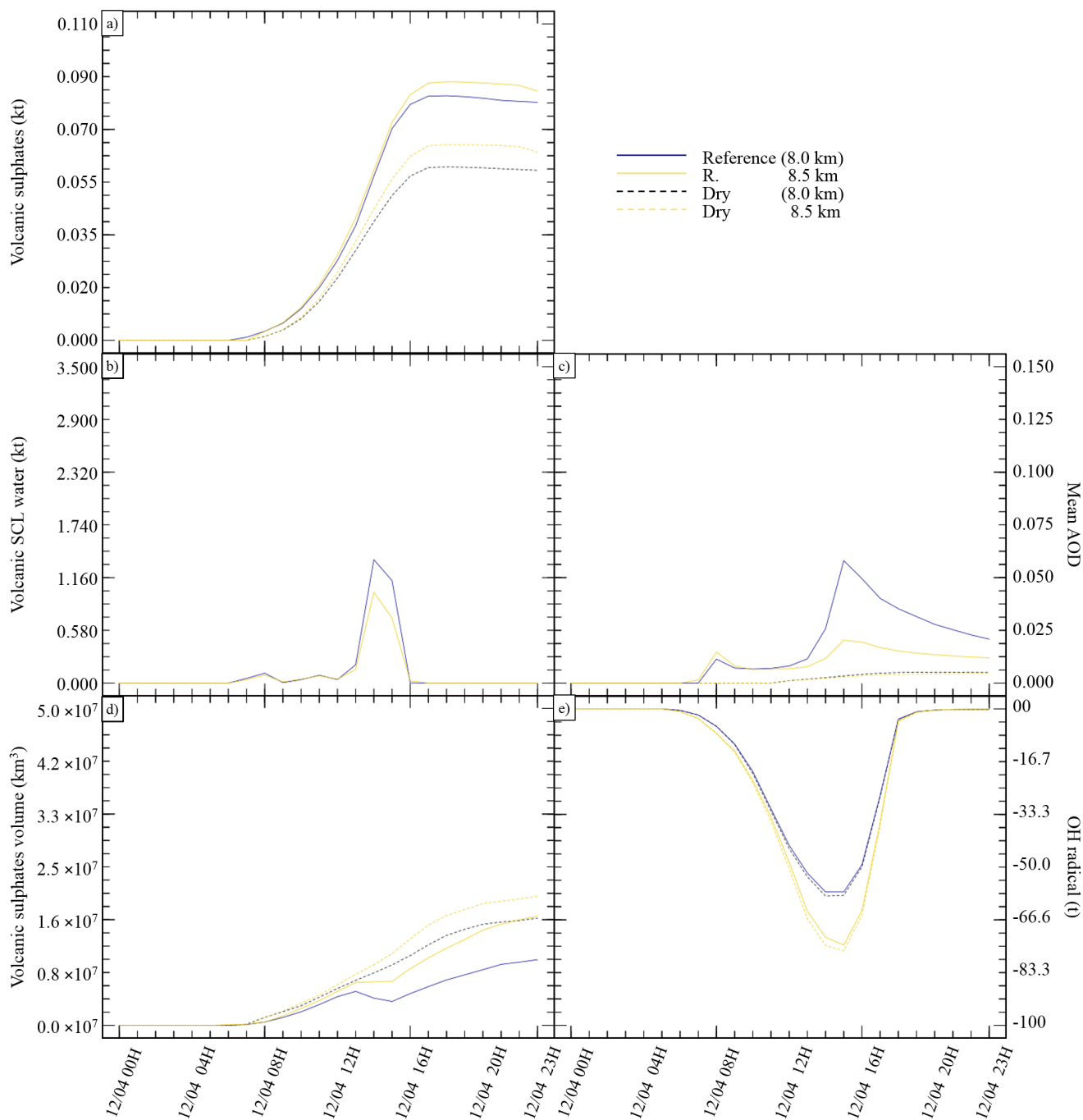
Figure 6. Sensitivity tests on vertical transport scheme. a) \text{SO}_{4(\text{p})}^{2-} (kt), b) SCLW (kt), c) AOD for plume \subset 25 % of \text{SO}_{4(\text{p})}^{2-} mass, d) Minimum volume ( \text{km}^3 ) \subset 25 % of \text{SO}_{4(\text{p})}^{2-} mass, e) OH radical (t).
