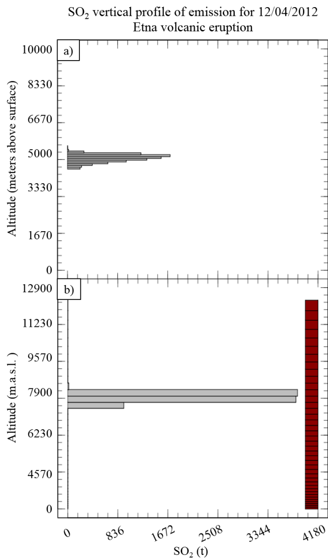
Figure 1. SO 2 vertical profile of emission for 12/04/2012 Etna volcanic eruption. a) Emission distribution following a skewed distribution. b) Emissions in the model after adaptation to the vertical grid used in CHIMERE (shown as red boxes).
