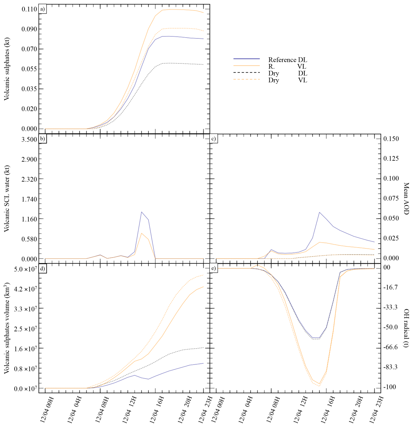
Figure 7. Sensitivity tests on injection height. a) \text{SO}_{4(\text{p})}^{2-} (kt), b) SCLW (kt), c) AOD for plume \subset 25 % of \text{SO}_{4(\text{p})}^{2-} mass, d) Minimum volume ( \text{km}^3 ) \subset 25 % of \text{SO}_{4(\text{p})}^{2-} mass, e) OH radical (t).
