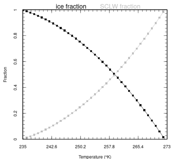
Figure A2. SCLW and ice fraction depending on temperature
