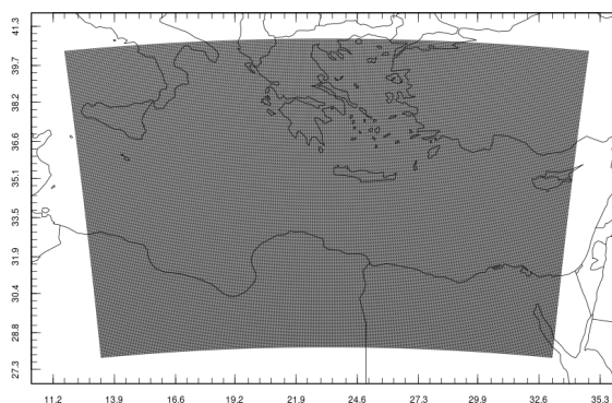
Figure A1. The CHIMERE simulation domain contains 874 \times 624 cells at 2.250 km resolution
