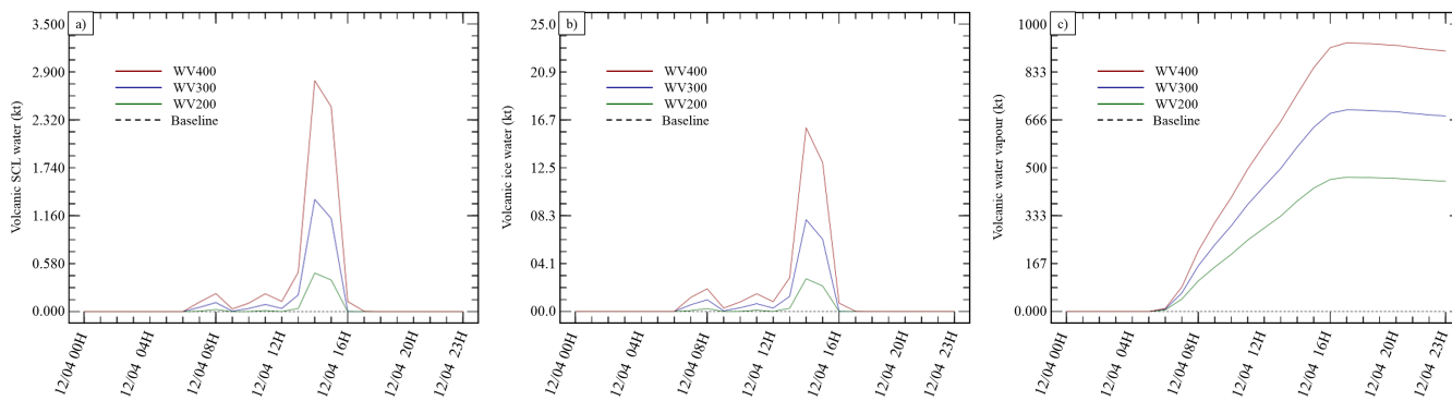
Figure B1. Water apportionment between its various states. a) SCL Water, b) ice, c) water vapour.
