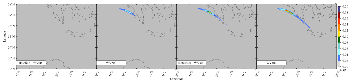
Figure 5. CHIMERE modelled 200 nm AOD from Volcanic sulphates.
