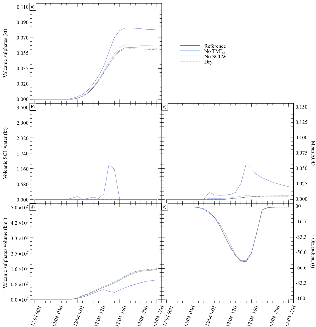
Figure 3. Sensitivity tests on vertical transport scheme. a) \text{SO}_{4(\text{p})}^{2-} (kt), b) SCLW (kt), c) AOD for plume \subset 25 % of \text{SO}_{4(\text{p})}^{2-} mass, d) Minimum volume ( \text{km}^3 ) \subset 25 % of \text{SO}_{4(\text{p})}^{2-} mass, e) OH radical (t).
