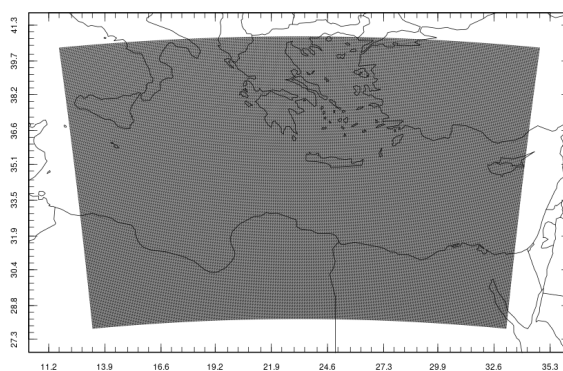
Figure A2. The CHIMERE simulation domain contains 874 \times 624 cells at 2.250 km resolution
