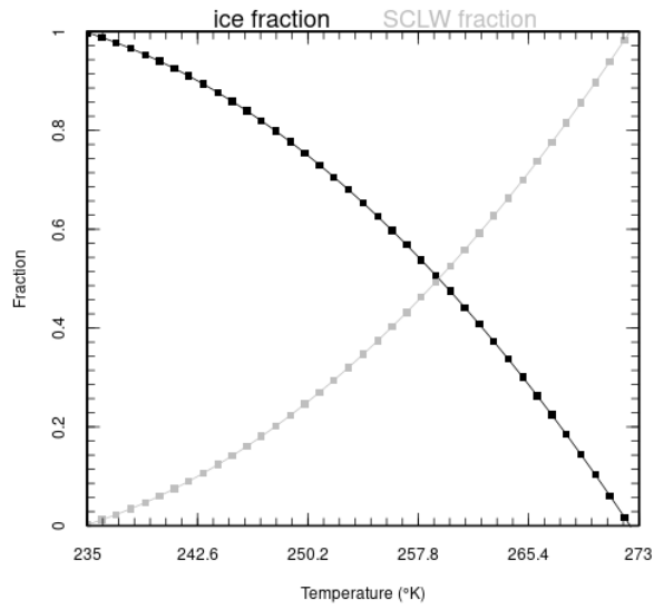
Figure A3. SCLW and ice fraction depending on temperature
