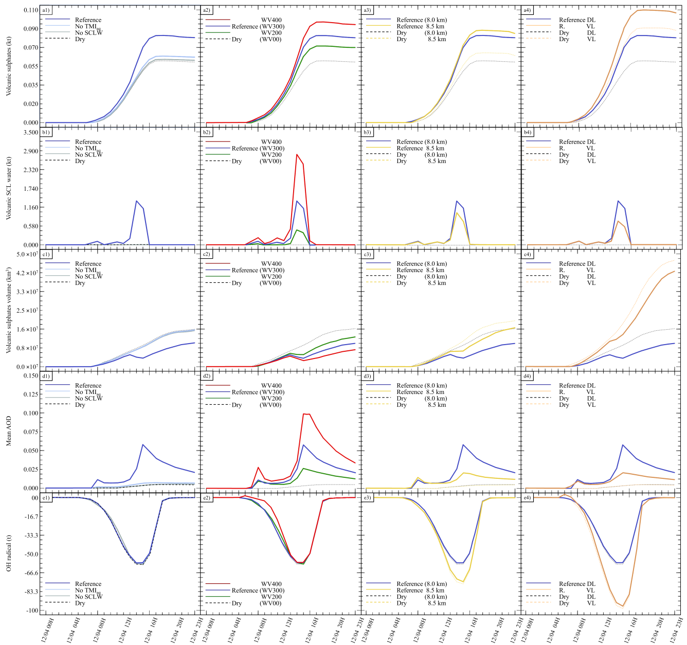
Figure A2. Gathering of the various performed experiences' results. a) \text{SO}_{4(p)}^{2-} (kt), b) Super Cooled Liquid Water (kt), c) Minimum volume ( \text{km}^3 ) \subset 25\% of \text{SO}_{4(p)}^{2-} mass, d) AOD for plume \subset 25\% of \text{SO}_{4(p)}^{2-} mass and e) OH radical (t). The Reference simulation is the closest to a realistic case.
