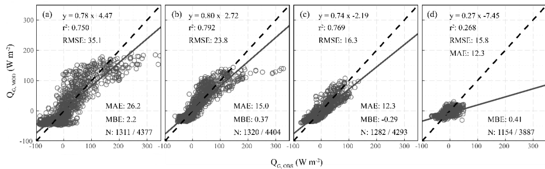
645 Figure B2: Weishan station modelled and observed soil heat flux, with statistical evaluation metrics (root mean square error (RMSE), coefficient of determination ( r^2 ), mean absolute error (MAE) and mean bias error (MBE)). N: evaluation data / total observations available) for (a) spring, (b) summer, (c) autumn and (d) winter.
