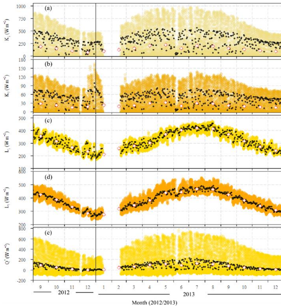
260 Figure 3: Observed 30 min (colour), daily (black) and monthly (white diamonds) means at Miyun (September 2012 to December 2013) of (a) incoming shortwave radiation ( K_{\downarrow} ), (b) outgoing shortwave radiation ( K_{\uparrow} ), (c) incoming longwave radiation ( L_{\downarrow} ), (d) outgoing longwave radiation ( L_{\uparrow} ), and (e) net all-wave radiation ( Q^* ). Data gap in January and February 2013 due to instrument failure. For the daily fluxes they are daytime ( K_{\downarrow} > 5 \text{ W m}^{-2} ) for the shortwave fluxes but 24 h for the others. 265
