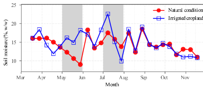
Figure 14: Gravimetric soil moisture (%) at a depth of 0.1 m measured on the 8th, 18th and 28th of each month at the MY site from 18 March to 18 November 2013 under natural condition and irrigated cropland. The shading is May and July 2013, respectively.
