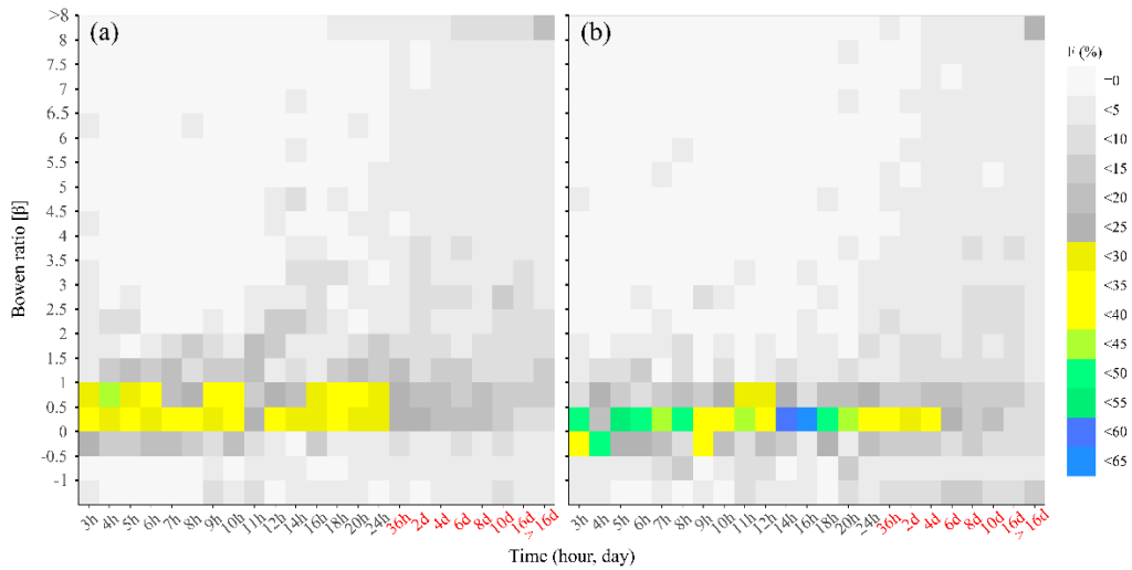
515 Figure 17: Frequency (F, %) of Bowen ratio \beta values by time since last rainfall for (a) building-dominant (210-360°) and (b) farmland-dominant (30-150°) directions.
