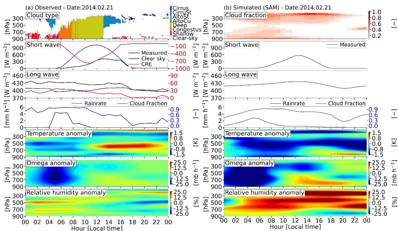
Figure 5 - Daily cycle of cloud type, cloud fraction profile, longwave and shortwave radiation fluxes for cloud and clear-sky sky ( W m^{-2} ), precipitation rate ( mm h^{-1} ), integrated cloud fraction and temperature (K), omega ( mb h^{-1} ) and relative humidity (%) anomaly from 2014.02.21 for the (a) observed data and (b) simulated with the SAM model.
