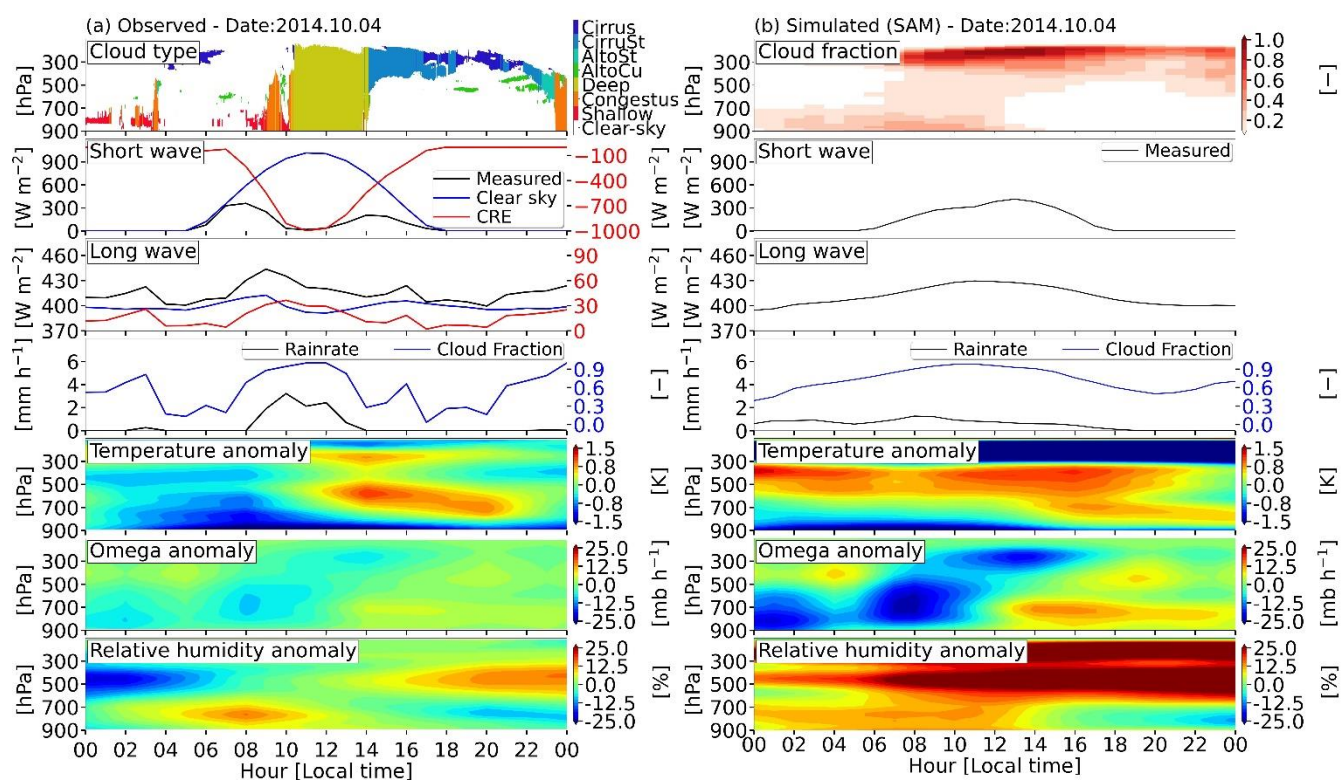
Figure 6 - Daily cycle of cloud type, cloud fraction profile, longwave and shortwave radiation fluxes for cloud and clear-sky sky ( W m^{-2} ), precipitation rate ( mm h^{-1} ), integrated cloud fraction and temperature (K), omega ( mb h^{-1} ) and relative humidity (%) anomaly from 2014.10.04 for the (a) observed data and (b) simulated with the SAM model.
