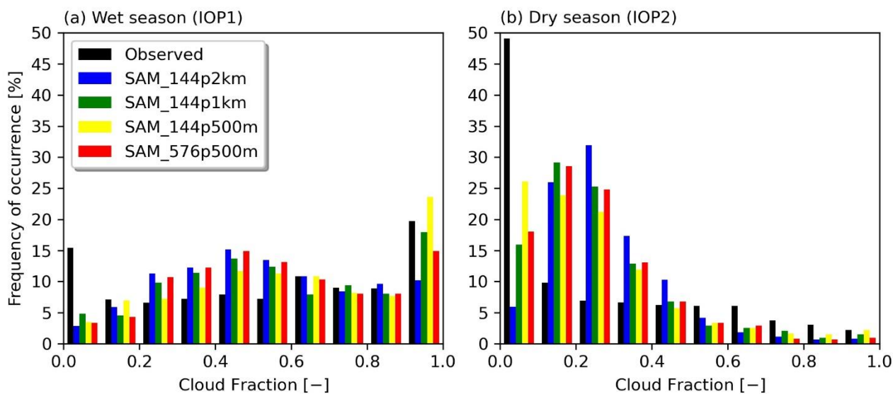
Figure 4 - Histogram of the integrated cloud fraction distribution (clear-sky 0 and cloud-sky 1) for the observed and simulated data with the SAM model in different resolutions for the periods of IOP1 (a) and IOP2 (b).
