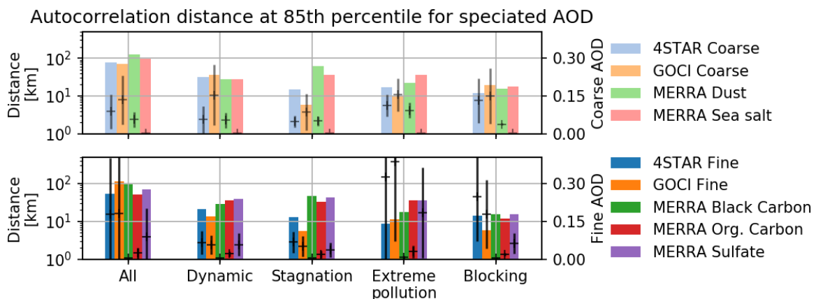
Figure 12 - The distance for the 85 th percentile autocorrelation, or which the autocorrelation is decreased by 15%, for a variety of speciated AODs, including fine and coarse mode AOD for 4STAR and GOCI, and dust, sea salt, black carbon
