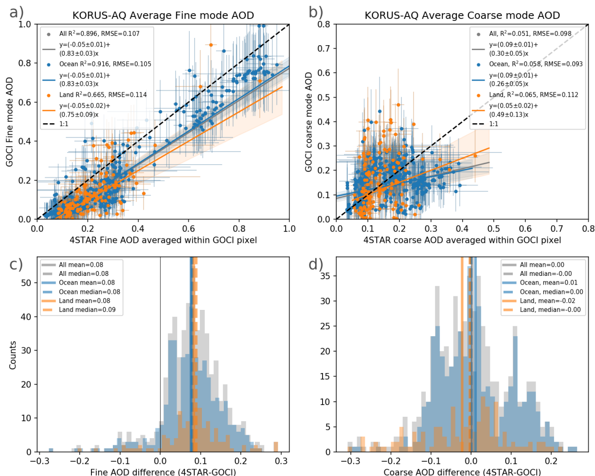
Figure B2 - Average 4STAR (a) fine and (b) coarse mode AOD within the different GOCI pixels matched on the same observation times and locations for all measurements under 500 m. The uncertainty in GOCI is using those characterized by Choi et al. (2018). 4STAR fine and coarse mode AOD is the standard deviation within the matched GOCI pixels. The linear relationship is quantified using a bivariate fit described by York et al. (2004). The differences between the observations by 4STAR and GOCI is found for fine mode AOD in (c) and for coarse mode AOD in (d). This comparison is subset between AOD measured over land (in orange) and over the ocean (in blue). The separation between land and ocean was achieved using the 1-km resolution GLOBE data (Hastings and Dunbar, 1999) ported for use in python (Karin, 2020).
