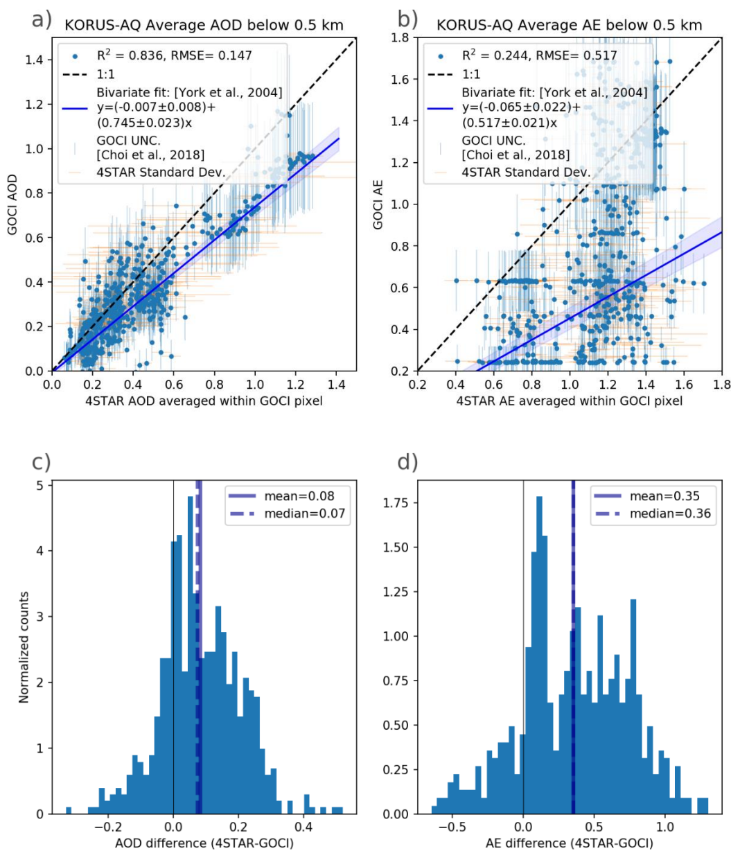
920 Figure B1 - Comparison of AOD at 500 nm from GOCI retrievals as compared to 4STAR measurements below 500 m. For each cloud cleared GOCI pixel, the nearby 4STAR samples (within 30 minutes of GOCI retrievals) are averaged together for this comparison, shown in the upper pair of graphs (a for AOD and b for AE). The linear fit used here is the bivariate fit described by York et al. (2004), and reinforced for use by Cantrell (2008). The difference between the matched 4STAR to GOCI values are presented in the bottom pair of histograms (c for AOD and d for AE).
