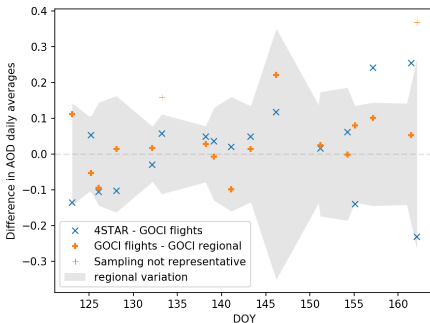
470 Figure 6 - Difference in daily average AOD as a function of the DOY depending on the sampling: GOCI regional averages, GOCI flights - subset to match spatial and time of flight observations, and differences between 4STAR matched to the GOCI flights. The grey shaded regions indicate one standard deviation of the AOD in the region as observed by GOCI.
