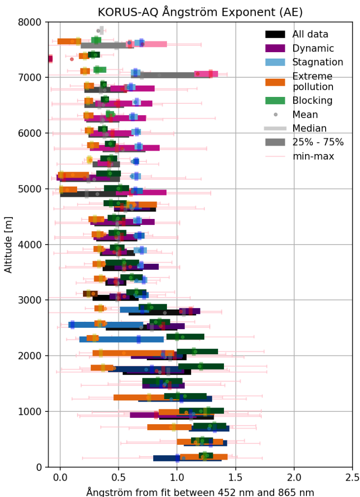
535 Figure 9 - Ångström Exponent (AE) box-plot distribution measured at different altitudes separated by different meteorological periods, during KORUS-AQ, and for all data (black). The number of days sampled within each vertical bin and meteorological regime is illustrated by the shading of the color. The vertical bar indicates the median of each altitude bin, while the center dot represents the mean. The interquartile range of the data in each vertical bin is represented by the thick horizontal bar. The range of values observed at the given altitude is presented as horizontal, colored, error bars.
