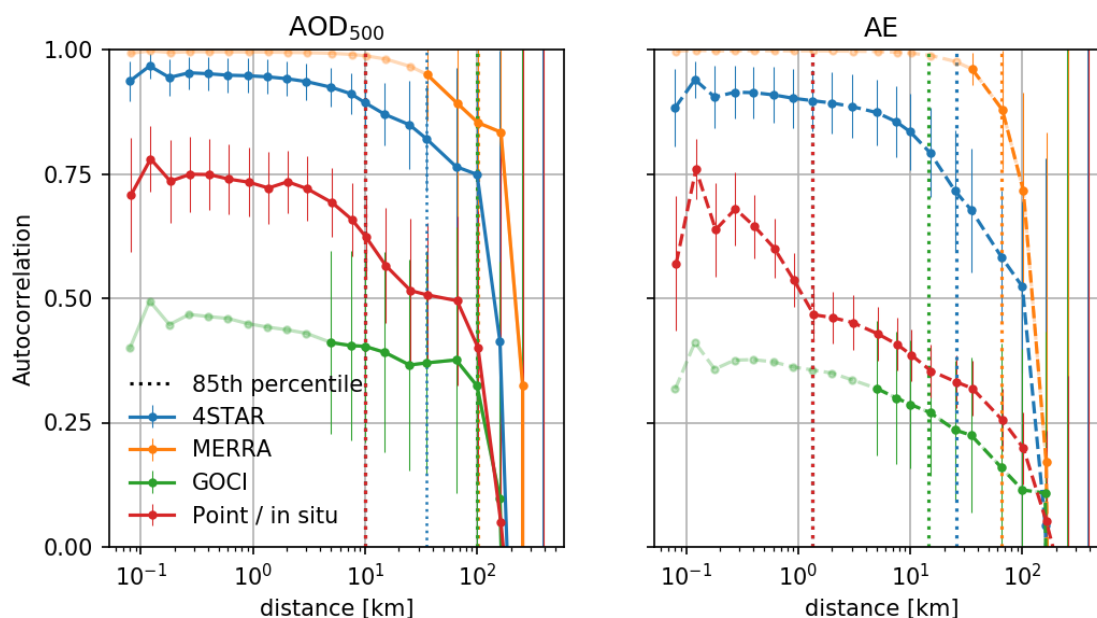
Figure 10 - The autocorrelation distances of the aerosol properties measured and modeled during KORUS-AQ, separated by either aerosol intensive properties (right, AE, relating to aerosol size, dashed lines) or extensive properties (left, column AOD, solid lines). The point / in situ denotes the autocorrelation from the aerosol extinction coefficient instead of the column values of all others. The colors denote the source of the data presented here. The vertical error bars represent the standard deviation of the 50-member ensemble Monte Carlo subsampling at 30% of flight segments. The vertical dotted lines represent the autocorrelation distance of the 85 th percentile, which is the location that the autocorrelation is reduced by 15% when compared to the autocorrelation of the shortest distance. The lighter colored lines for GOCI and MERRA-2 represent the autocorrelation for distances smaller than the diagonal length from one pixel center to another, which are closest to the NASA DC-8 flight path.
