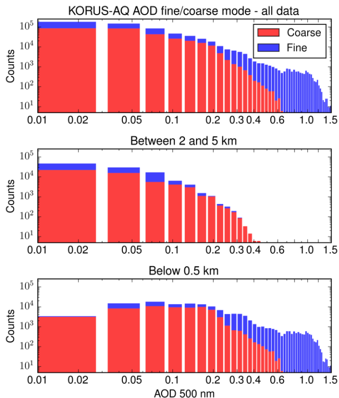
Figure 8 - Histograms of fine and coarse mode AOD measured during KORUS-AQ for all data (top), AOD measured between 2 km and 5 km (middle), and below 500 m (bottom). The total length of the histogram bar indicates the total AOD in that bin, while the red/blue differentiation indicates the portion of the total AOD due to AOD from either fine or coarse mode aerosol.
