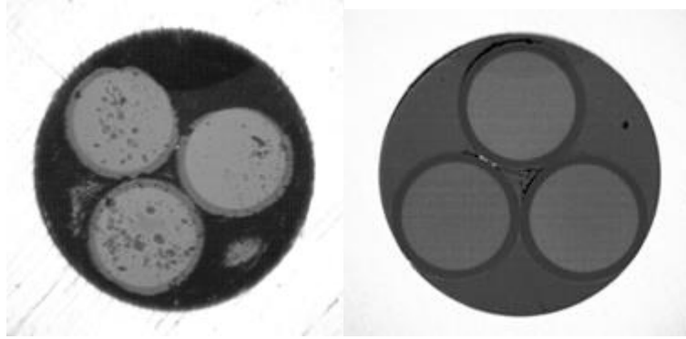
870 Figure A1 - Image of 3-element fiber optic bundle endface that is part of the solar direct beam measurement optical path of 4STAR. Before polishing is seen on the left, while after polishing on the right. The uneven fiber flatness, severe contamination and pocked endface increased scattered light and was linked to distortions in the instrument field of view. The polished fiber face has a very planar endface, with no pocking and contamination resulting in a much more predictable light measurement.
