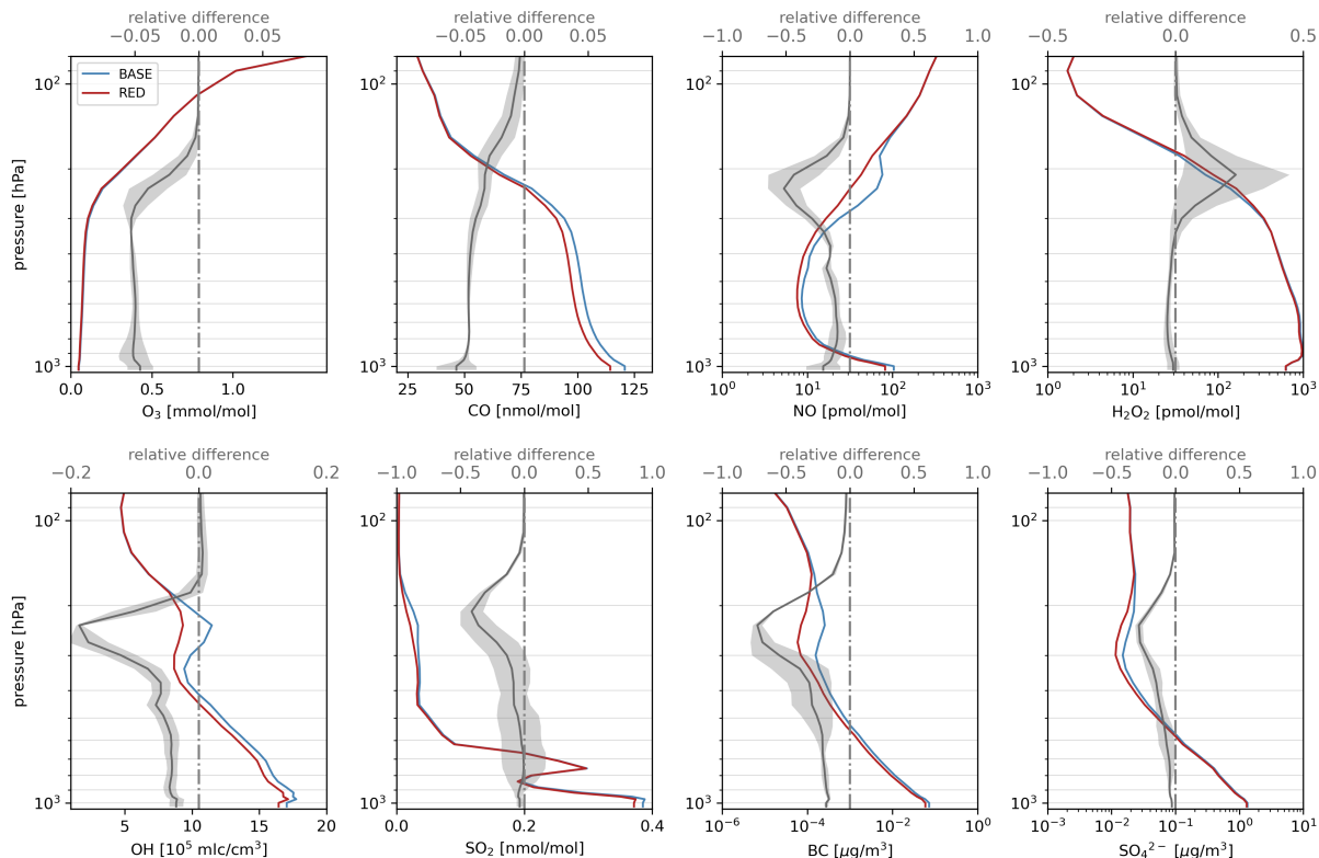
Figure 5. Vertical profiles from BASE and RED simulations and their relative difference ((\text{RED}-\text{BASE})/\text{BASE}) . The grey area represents one standard deviation of the spatial-temporal mean (grey line). Please note the different scales for the relative differences.
