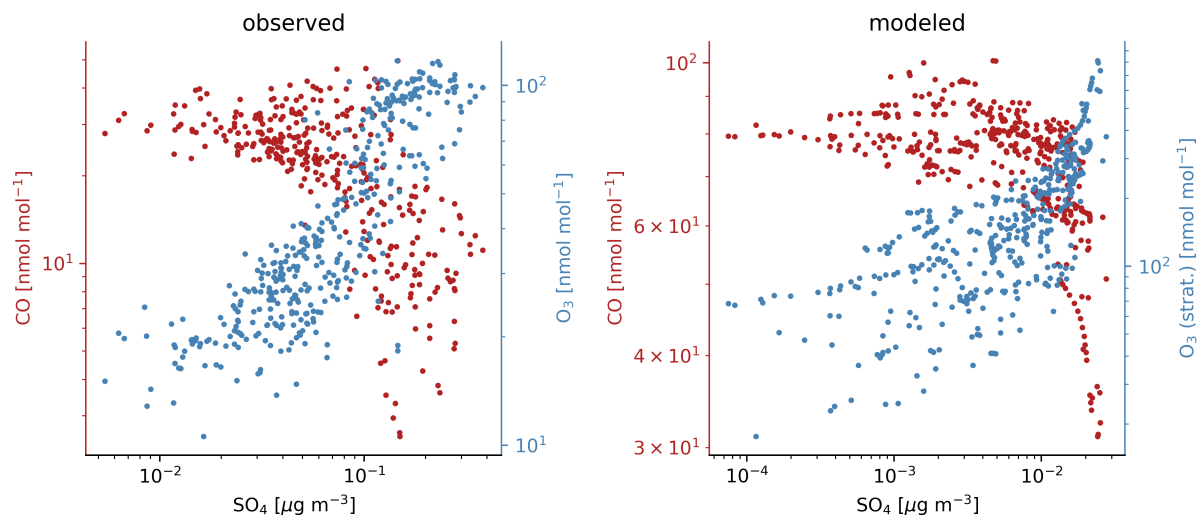
Figure 4. Scatter plot of co-located \text{SO}_4 and \text{CO} (red) and \text{O}_3 (blue) abundance between 350 and 150 hPa from observations (left) and the RED simulation (right).
