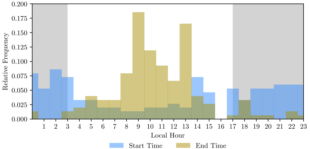
Figure 7. Histograms of the start time (blue) and end time (brown) of pockets of open-cell stratocumulus are shown.
