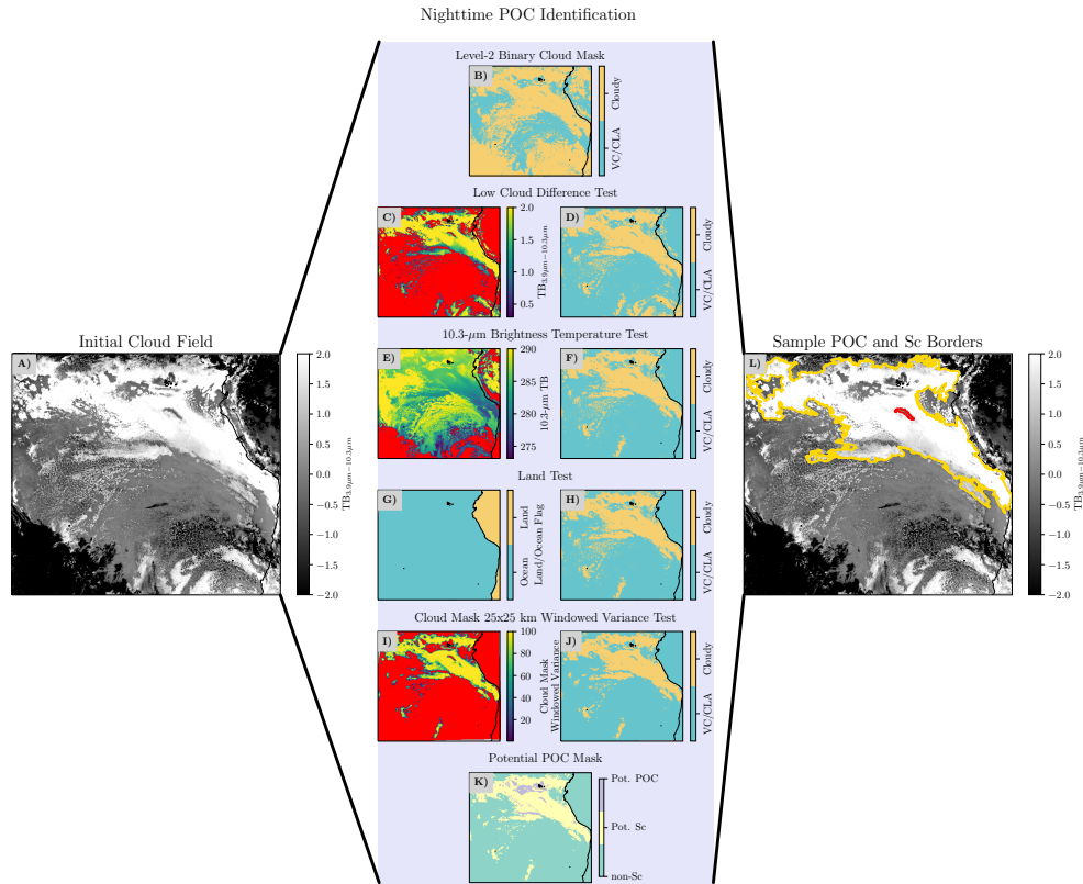
Figure 3. Shown above are the steps used to identify pockets of open-cell (POCs) stratocumulus during the night. In the third column, the stratocumulus deck borders are in yellow and POC borders are in red.
