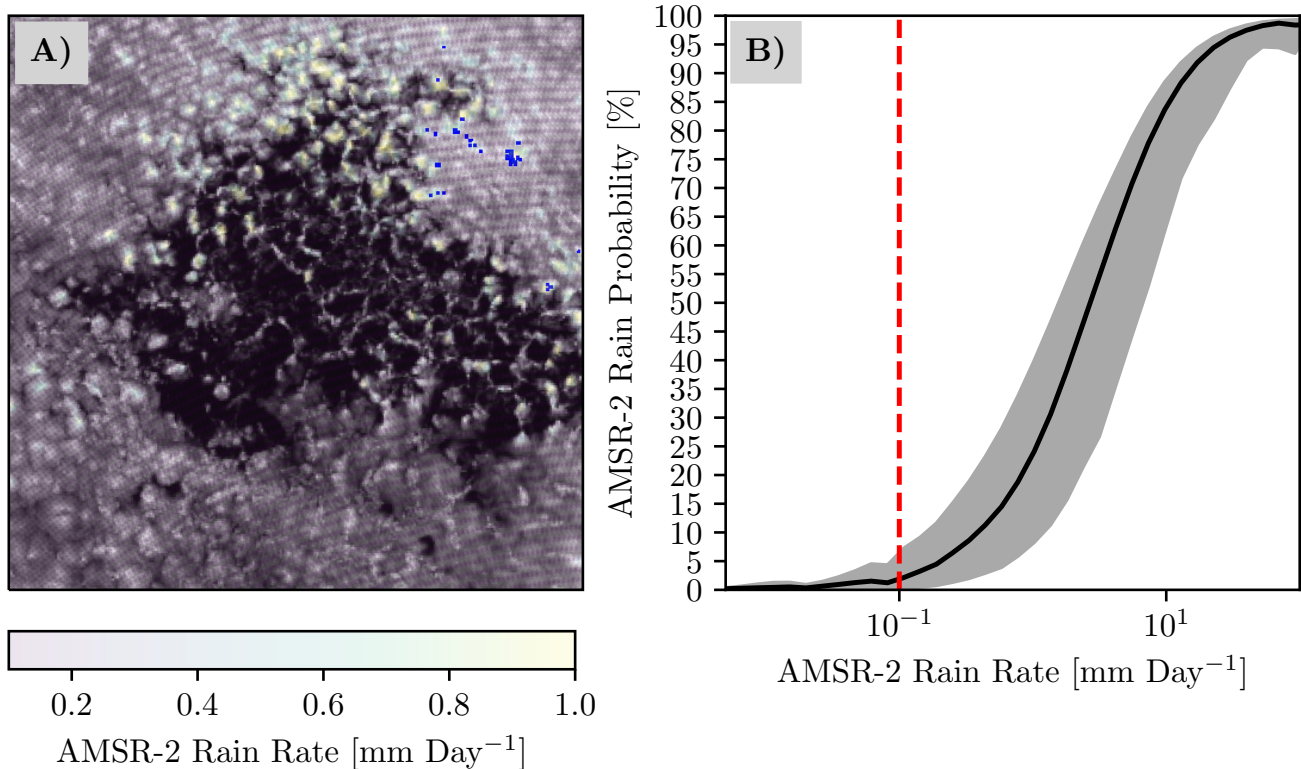
Figure 4. Advanced Microwave Scanning Radiometer 2 (AMSR-2) rain rates matched to the POC shown in Figure 2 overlaid on GOES-16 0.64\text{-}\mu\text{m} reflectance are shown in panel A). AMSR-2 rain probability as a function of rain rate for all September-November 2019 data over the entire domain are shown in panel B), where the solid black line represents the median probability at a given rain rate, grey fill represents the 10^{\text{th}} - 90^{\text{th}} percentile spread at a given rain rate, and the dashed red line represents the rain rate threshold of 0.1 \text{ mm day}^{-1} .
