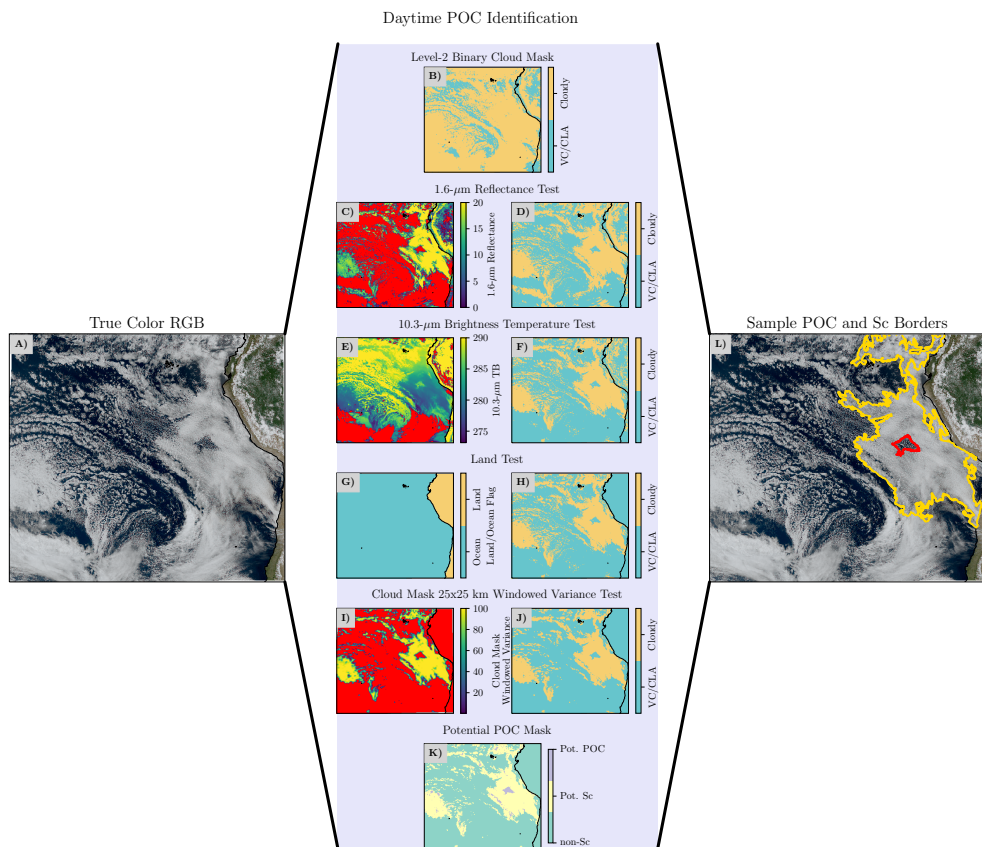
Figure 2. Shown above are the steps used to identify pockets of open-cell (POCs) stratocumulus during the day. In the third column, the stratocumulus deck borders are in yellow and POC borders are in red.
