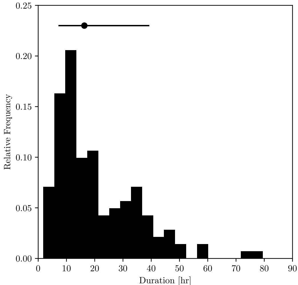
Figure 6. A histogram of the duration of pockets of open-cell stratocumulus is shown. The black dot above the histogram represents the median and the horizontal black line represents the 10 th to 90 th percentile spread.
