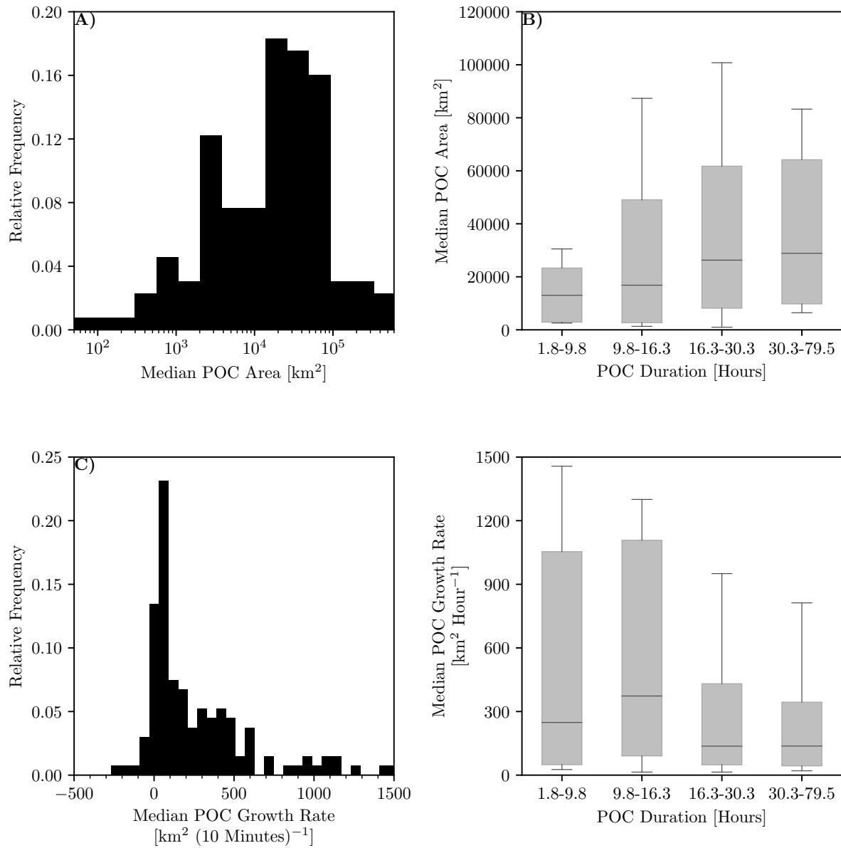
Figure 8. The Histogram of the median area of pockets of open-cell stratocumulus (POCs) is shown in panel A), the distribution of median POC area as a function of POC duration is shown as box plots in panel B), where the solid line represents the median duration, the Histogram of POC median growth rate is shown in panel C), and the distribution of median POC growth rate as a function of POC duration is shown as box plots in panel B). Note that in the boxplots, the shaded boxes represent the interquartile range, the solid lines inside the shaded regions represent the median, and the whiskers represent data between the 10 th and 90 th percentiles.
