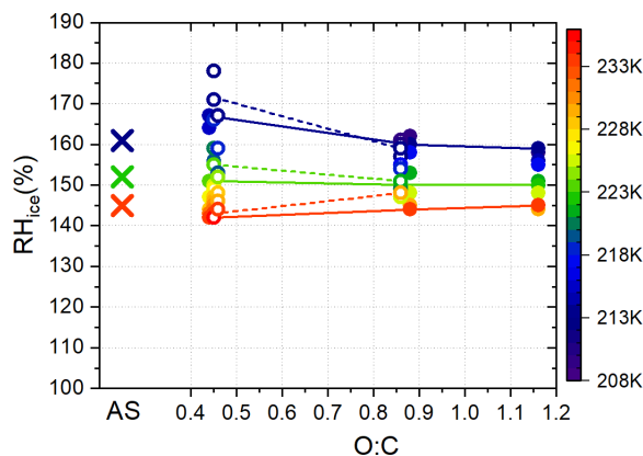
Figure 3. Relative humidity of ice formation on 1% of 100 nm \alpha -pinene SOA particles as function of O:C ratio (circles) in comparison to ammonium sulfate (AS, shown as crosses). AS data from Welti et al. (2020). Open circles indicate experiments with \alpha -pinene particles preconditioned at RH_w < 1\% , filled circles RH_w = 10\% . Trendlines are shown for experiments at 213 K, 223 K and 233 K. Temperature is indicated by the color scale.
