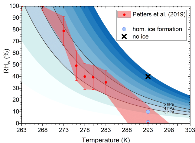
Figure 5. Comparison of SOA pre-treatment conditions to SOA phase transition (viscosity 4e5 to 6e6 , red envelope) from Petters et al. (2019). We note that the phase transition coincides with a partial water vapor pressure (shown in blue) of 3-5 hPa. Homogeneous ice nucleation was only observed for SOA particles exposed to low water vapor pressure during pre-conditioning.
