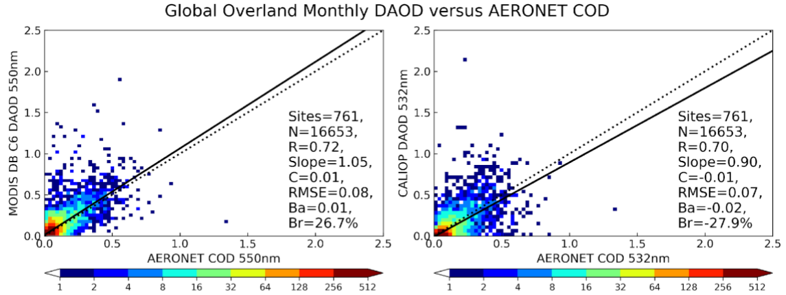
Figure 1. Scatter density histogram comparing monthly (from 2007 to 2019) MODIS DAOD (on the left panel) and CALIOP DAOD (on the right panel) with monthly coarse mode COD_{SDA} retrieved at 550nm for MODIS comparison and at 532nm for CALIOP comparison from the Level 2 (cloud screened and quality assured) Spectral Deconvolution Algorithm (SDA) version 4.1 (O'Neill et al., 2003). The 1 to 1 line and linear regression line are shown by dotted and solid lines, respectively. The number of sites (Sites), of matchups (N), correlation (R), slope (S), constant (C), and root mean square error (RMSE) of the linear regression as well as absolute bias (Ba) and relative Bias (Br) are indicated in the lower right of the panel. Ba, Br and RMSE are defined as:
