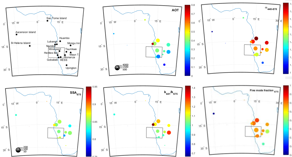
Figure 4: Mean values of AOD at 550 nm, \alpha_{440-870} , SSA at 675 nm, ratio of the imaginary part of the refractive index ( k ) between 441 nm and 675 nm, and the fine to coarse mode fraction of the aerosol volume concentration from 15 AERONET sites in the South-Eastern Atlantic region. The selected period is from the 15 August to the 15 September 2017. The black box corresponds to the AEROCLO-sA flight domain. Circle size is linked to the availability of the data in number of measurements.
