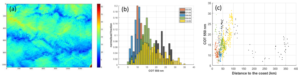
Figure 11: a) Full OSIRIS image Cloud Optical Depth at 550 nm retrieved on 7 September at 09:37 UTC from OSIRIS measurements. b) COT histogram for the 5 selected flight. c) Relation between COT and the distance from the measurement to the coastline.
