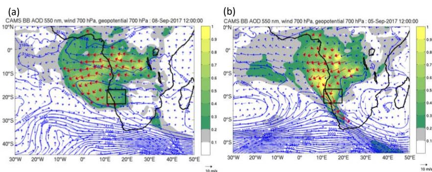
Figure 2: Regional atmospheric circulation and aerosol for a) the 8th of September 2017 and b) the 5th of September 2017 at 12:00 UTC. Geopotential height (contours) and wind (arrows) at 700 hPa and biomass burning AOD at 550 nm (shadings) from CAMS reanalysis are displayed. Red arrows highlight wind vectors at grid points where the AOD is higher than the 90 th percentile of the regional AOD. The AEROCLO-sA campaign region is located with a black rectangle in the Namibian region.
