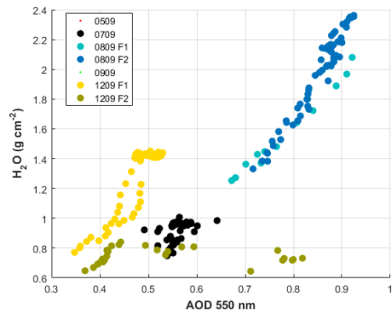
Figure 10: Column water vapour in function of AOD at 550 nm both measured by the PLASMA2 Sun-photometer during the AEROCLO-sA campaign.
