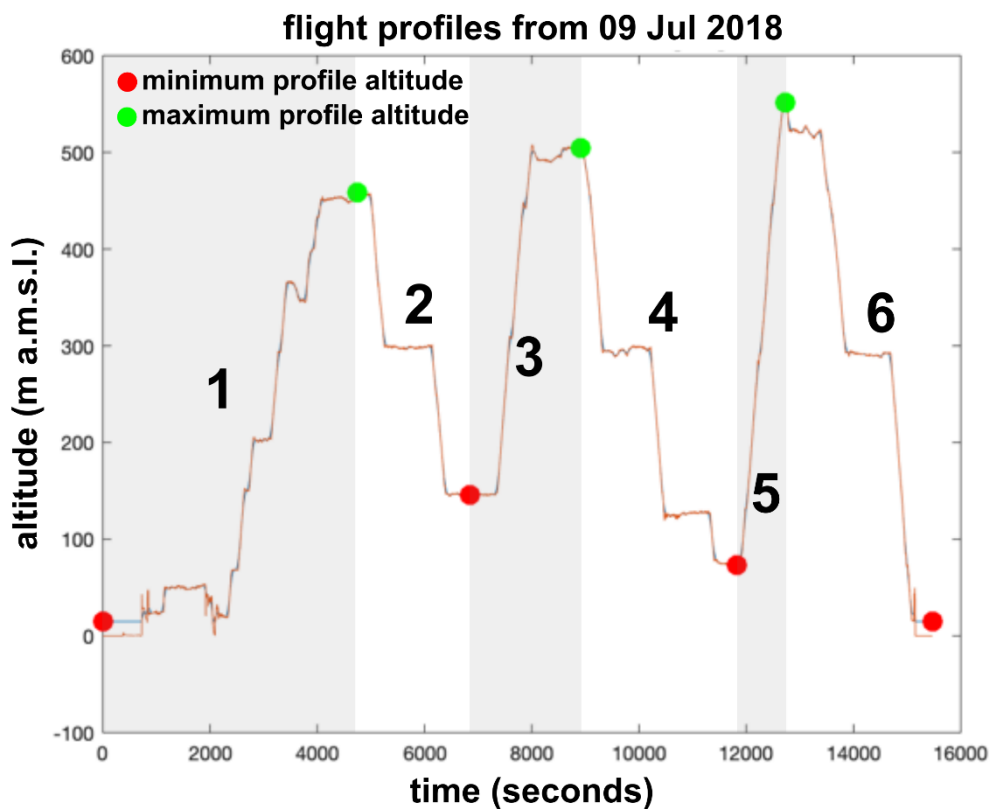
425 Figure 2: Example of how flight profiles are defined from 09 Jul 2018. The red and green markers represent the minimum and maximum altitude of each profile, respectively, and thus define the start and end points of each profile. This example consisted of 6 profiles for the entire flight time period.
