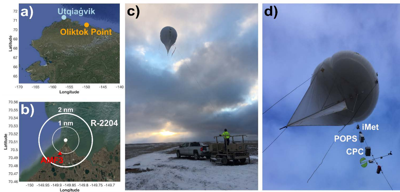
Figure 1: Maps illustrating a) the location of Oliktok Point, Alaska and b) the scale (in nautical miles, nm) of the restricted airspace area (R-2204) set up for operation of the TBS and location of AMF3 (red triangle). The map was created using satellite imagery obtained through the © Google Earth Application Programming Interface. Also shown are images of the TBS (34 m 3 helikite), including c) the Sandia National Laboratories winch trailer used for flight and d) a close-up of a typical instrument payload. Only the instruments mentioned in this manuscript are labelled.
