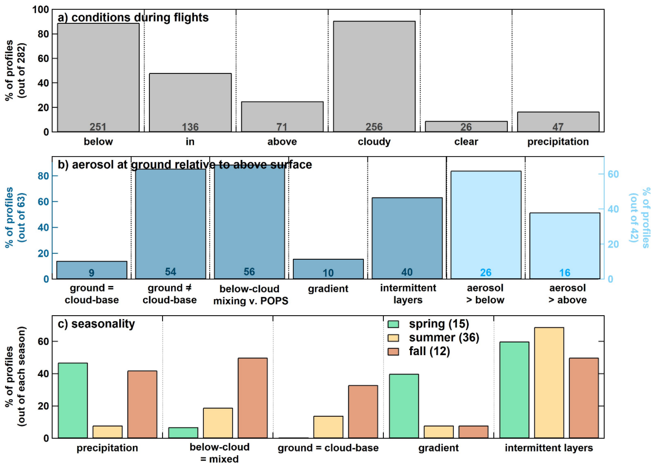
475 Figure 9: Statistics from all profiles with POPS data (282 total) during the ARM TBS campaigns, including a) when the POPS flew below, in, and above cloud and conditions during the flights (clear or cloudy), and precipitation. Out of the profiles that POPS was operational at cloud base and at the ground (63 total), b) shows cases where aerosol concentrations were equivalent and not equal at ground and cloud base. When not equal, cases are categorized into an increasing or decreasing gradient with height when intermittent layers were present, and cases where below-cloud mixing can explain the stratification of the aerosol. Also shown are 480 cases where the POPS measured above and below cloud within the same profiles (42 total) and which cases had higher aerosol concentrations below and above cloud. c) shows various conditions by season from b). The number of cases is provided for a) and b). The number of profiles per season is provided in c).
