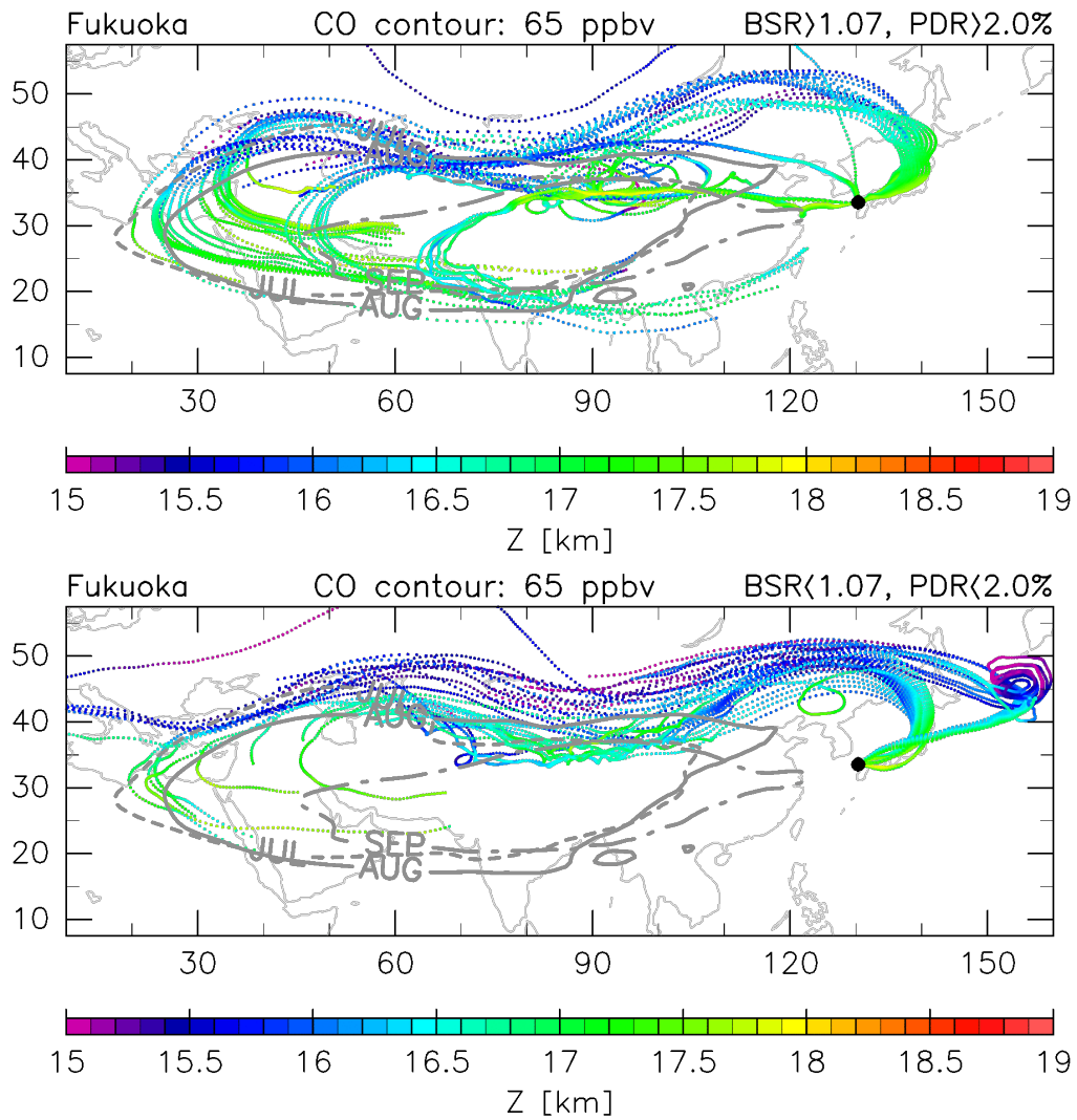
270 Figure 5 As for Fig. 4, but for trajectories from Fukuoka, with (top) 44 and (bottom) 37 trajectories.
