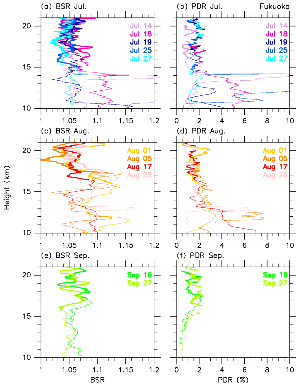
230 Figure 3 Eleven vertical profiles of (a, c, e) backscattering ratio (BSR) and (b, d, f) particle depolarization ratio (PDR, in %) in (a, b) July, (c, d) August, and (e, f) September 2018 obtained using the lidar system at Fukuoka. Dates and colours are assigned in the legend where, for example, “Jul 14” refers to the night of July 14–15. Stratospheric portion of the profiles has been thickened using the daily (first) lapse-rate tropopause location information provided by the JMA, based on operational 21 LT radiosonde data taken at the JMA Fukuoka site (at a ~4 km distance from the lidar site).
