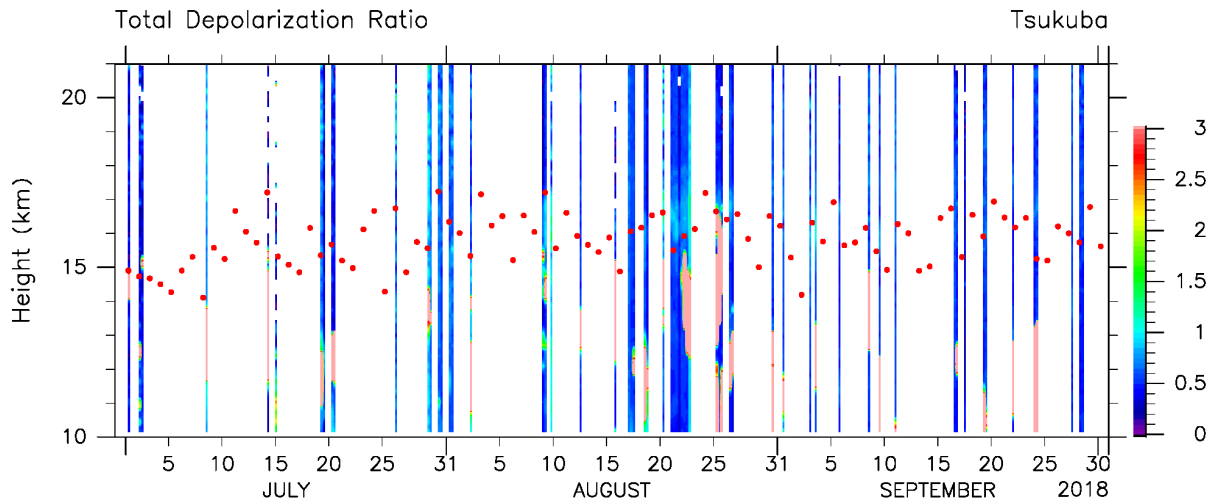
430 Figure A1 As for Fig. 1, but for the total depolarization ratio (TDR, %).
