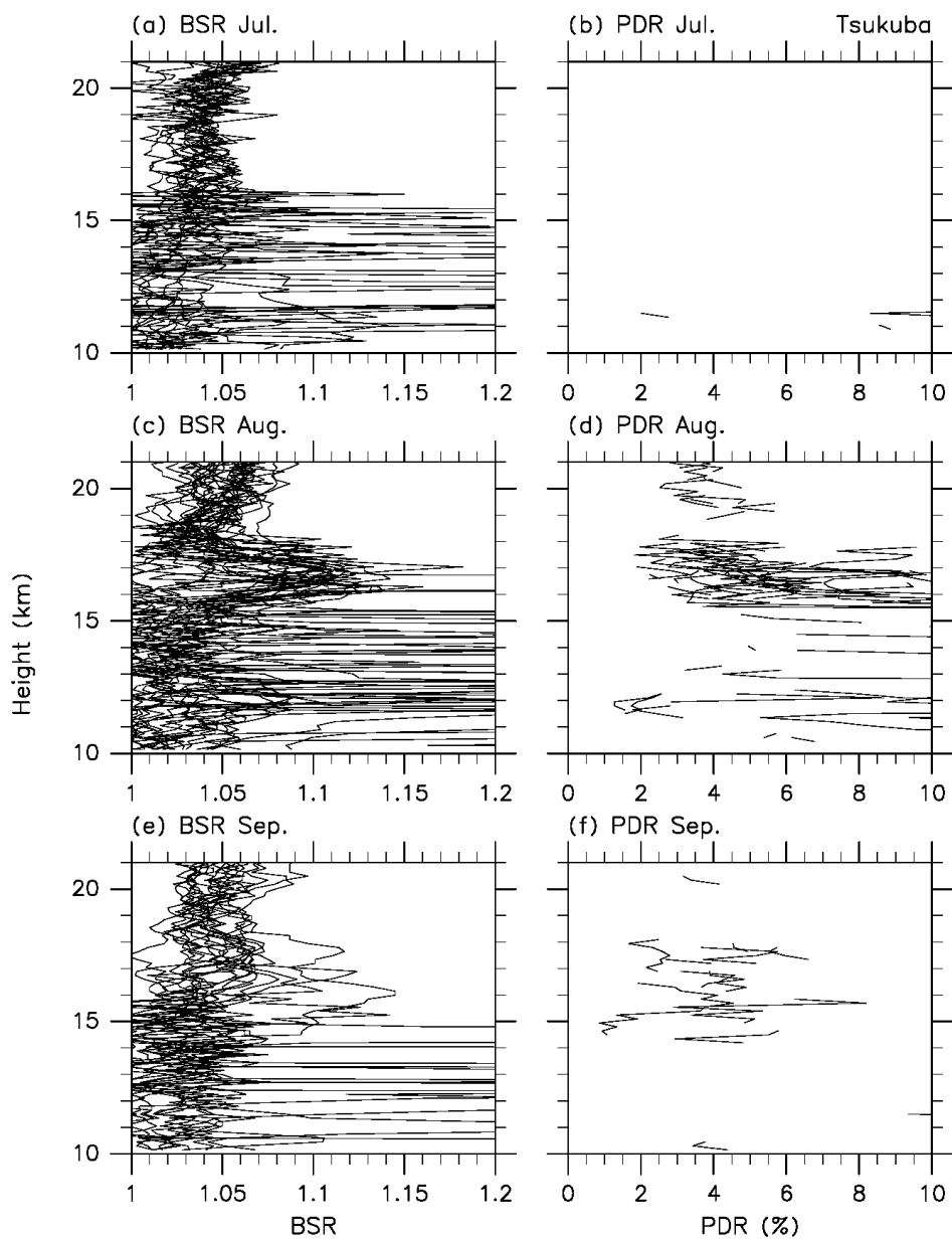
215 Figure 2 Vertical profiles of (a, c, e) backscattering ratio (BSR) and (b, d, f) particle depolarization ratio (PDR, in %) in (a, b) July, (c, d) August, and (e, f) September 2018 obtained using the lidar system at MRI, Tsukuba. It is noted that strong and noisy signals in BSR below \sim 15.5 km are due to cirrus clouds.
