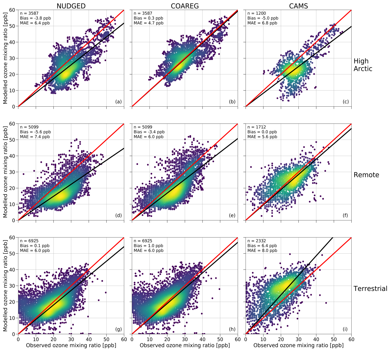
Figure 4. Comparison of the hourly observed and simulated ozone mixing ratios [ppb] for the DEFAULT-NUDGED (a,ed,ig), NUDGED and COAREG (b,fe,ikh), COAREG (c,g,k) runs and CAMS data (dc,hf,li) for the High Arctic (HA a-c) (a-d), Remote (RE d-f) (e-h) and Terrestrial (TE) (g-i) sites. The red line indicates the 1:1 line and the black line indicates the Ordinary Least Squares regression line through the origin. The number of data points (n), Bias [ppb] and Mean Absolute Error (MAE) [ppb] are shown in the top left corner. The colors represent the multivariate kernel density estimation with yellow colors having a higher density.
