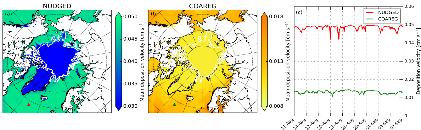
Figure 2. Spatial distribution of the mean simulated O_3 deposition velocity to snow/ice and oceans [ cm\ s^{-1} ] for the (a) NUDGED and (b) COAREG simulations and (c) temporal variation in O_3 deposition velocity [ cm\ s^{-1} ] for the NUDGED (red) and COAREG (green) simulations. The red and green markers in (a) and (b) indicate the location of the time series shown in (c). To give an indication of the sea ice extent, the white contours show the sea ice fraction of 0.5 at the start of the simulation.
