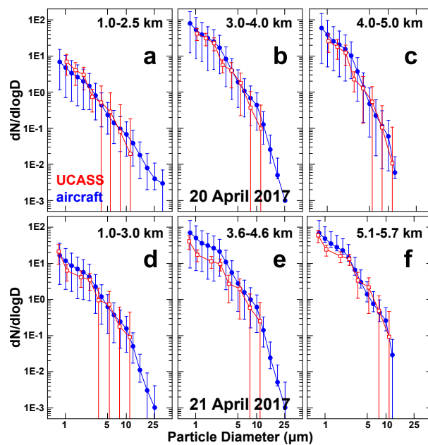
Figure 5. Particle number size distribution observed by UCASS (red) and with the CAPS instrument aboard the Falcon aircraft (blue) on 20 (a-c, launch 1) and 21 April 2017 (d-f, launch 3) for the height layers marked in Figure 4. Error bars refer to the standard deviation of the measurements.
