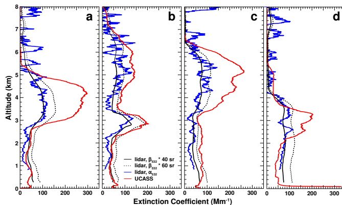
Figure 8. Aerosol extinction coefficient profiles from UCASS (red) and the Raman lidar PollyXT at Limassol. Lidar profiles refer to extinction coefficients obtained using the Raman method (blue) or by multiplying the aerosol backscatter coefficient derived without the use of Raman signals with lidar ratios of 40 sr (solid black line) and 60 sr (dotted black line).
