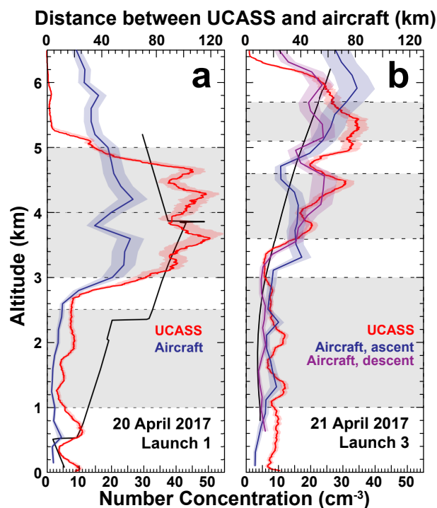
Figure 4. Total number of particles in the diameter range from 0.6 \mu\text{m} to 13.9 \mu\text{m} counted by UCASS (red) and with the CAPS instrument aboard the Falcon aircraft (blue and purple, size range from 0.79 to 14.0 \mu\text{m} , shading marks the standard deviation) measured (a) during the first UCASS launch on 20 April 2017 and (b) during the third UCASS launch on 21 April 2017. Red shaded areas refer to the effect of a counting uncertainty of 8% (y error) as stated in (Smith et al., 2019). The black lines mark the horizontal distance between the location of the observations from the UCASS and aircraft. Gray areas refer to the height layers considered in Figure 5.
