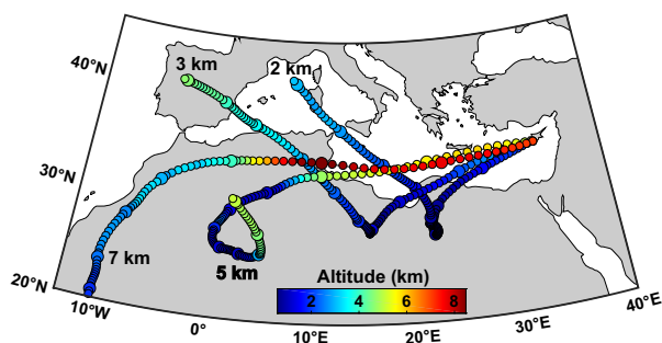
Figure 3. 120-h HYSPLIT backward trajectories starting over Limassol at 0100 UTC on 21 April 2017. Colour coding refers to the height of the trajectories. Intervals of 12 h are marked by increased circle size. The numbers in the plot refer to the arrival height over Limassol.
