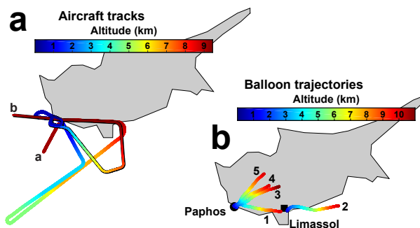
Figure 2. Flight tracks of (a) the DLR-Falcon aircraft and (b) the UCASS sondes launched from Paphos and Limassol. The Falcon tracks marked a (black border) and b (no border) refer to the research flights on 20 and 21 April 2017, respectively.
