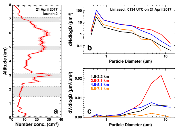
Figure 7. UCASS measurements during the second launch at 0134 UTC on 21 April 2017 from Limassol: (a) height profile of the total particle number concentration as in Figure 4 and (b) particle number and (c) volume size distributions averaged over four selected height levels as indicated in (a).
