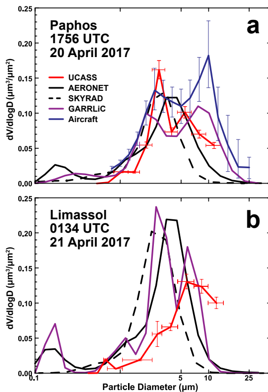
Figure 6. Total-column volume size distribution from the UCASS (red), AERONET (black solid), SKYRAD (black dashed), GARRLiC (purple), and aircraft (blue, only in a) obtained during (a) the first launch on 20 April 2017 and (b) the second launch on 21 April 2017. For clarity, only error bars of the UCASS and CAPS measurements are shown. Details on the locations and measurement times are provided in Table 1.
