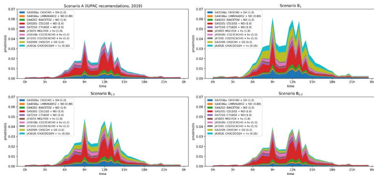
Figure 7: Modelled rates of \text{CH}_3\text{CO} formation (in ppt per seconds) through the diel cycle from photolysis of pyruvic acid (blue, orange and green) and other photochemical processes during IBAIRN. Top left: Scenario A (IUPAC recommendations from 2019). Top right: Scenario B 1 . Bottom left: Scenario B 0.5 . Bottom right: Scenario B 0.2 . In the legend, the first term is the equation tag used by CAABA/MECCA for the reaction. A full listing of the reactions can be downloaded (see “data availability”).
