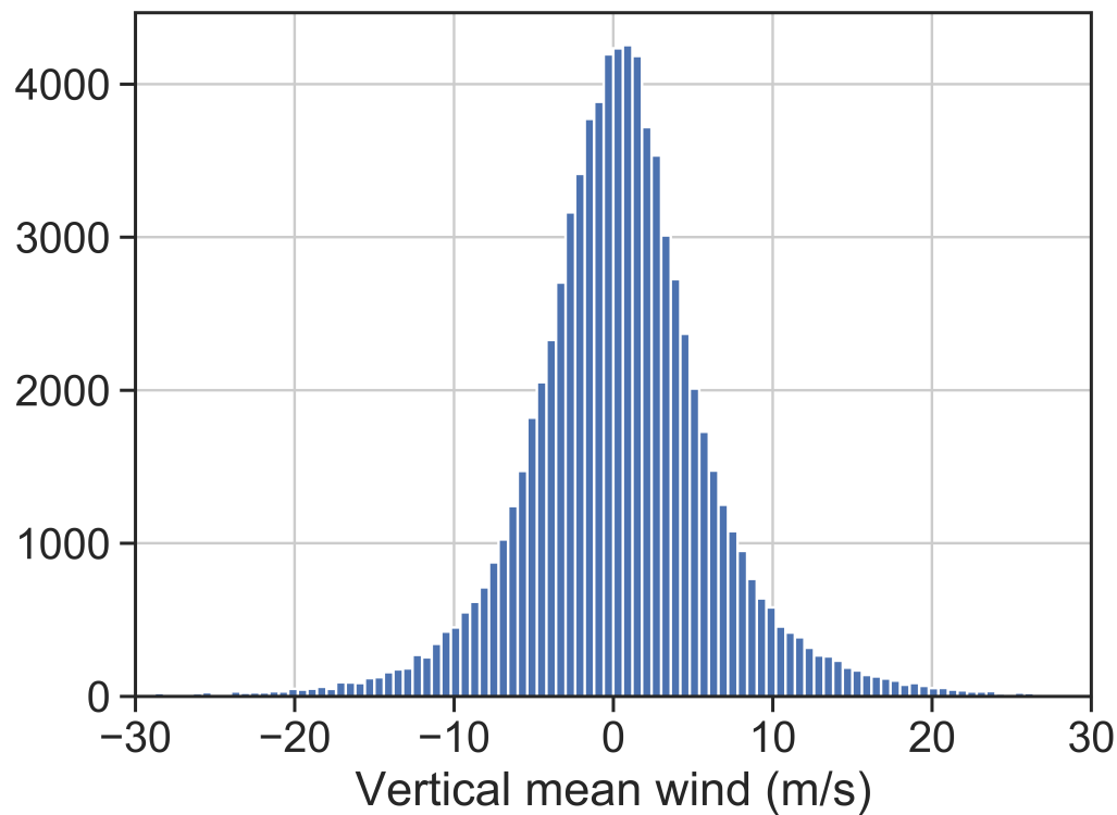
Fig. 2. Histogram of mean vertical velocity
