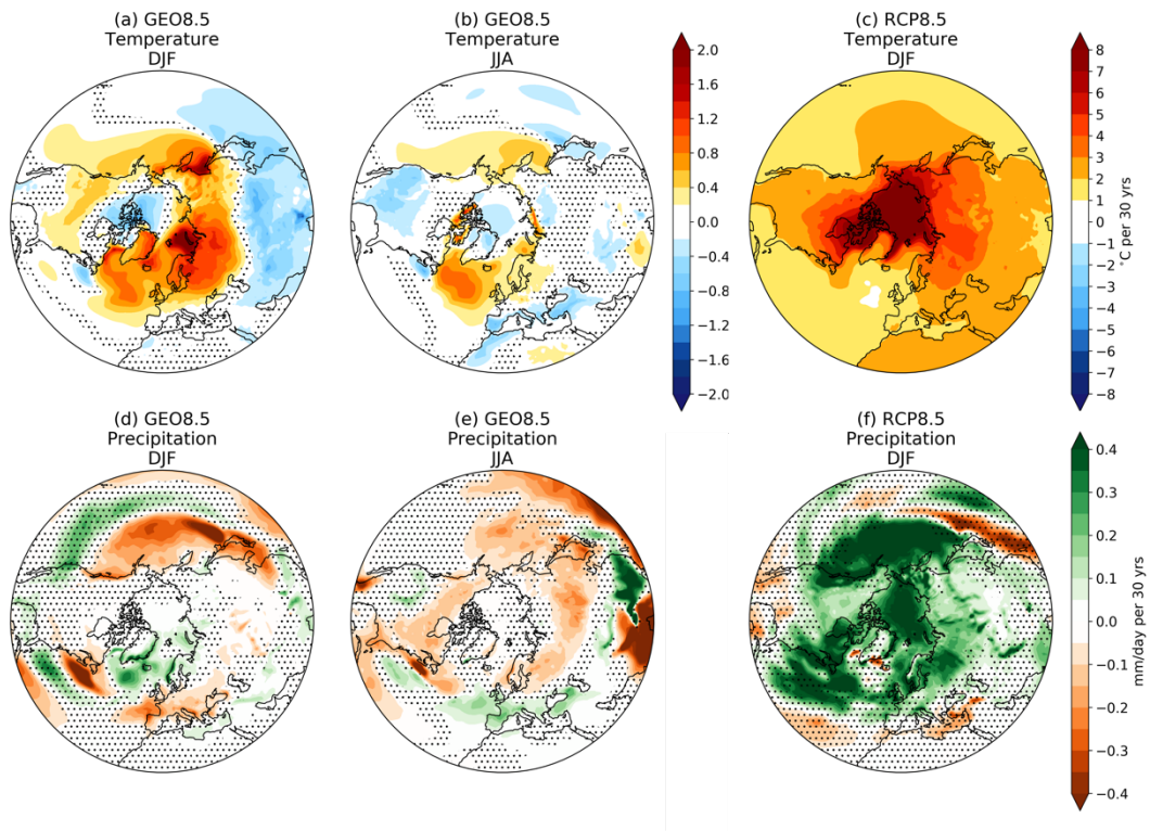
505 Figure 1. Trends in near-surface air temperature and precipitation. Ensemble mean linear trends in (a, b, c) temperature (°C per 30 yrs) and (d, e, f) precipitation (mm/day per 30 yrs) in different seasons and experiments: GEO8.5, DJF (first column), GEO8.5 JJA (second column) and RCP8.5, DJF (third column). Stippling indicates lack of statistical significance at the 95% confidence level under a one sample, two-sided Student's t -test using the standard deviation across ensemble members.
