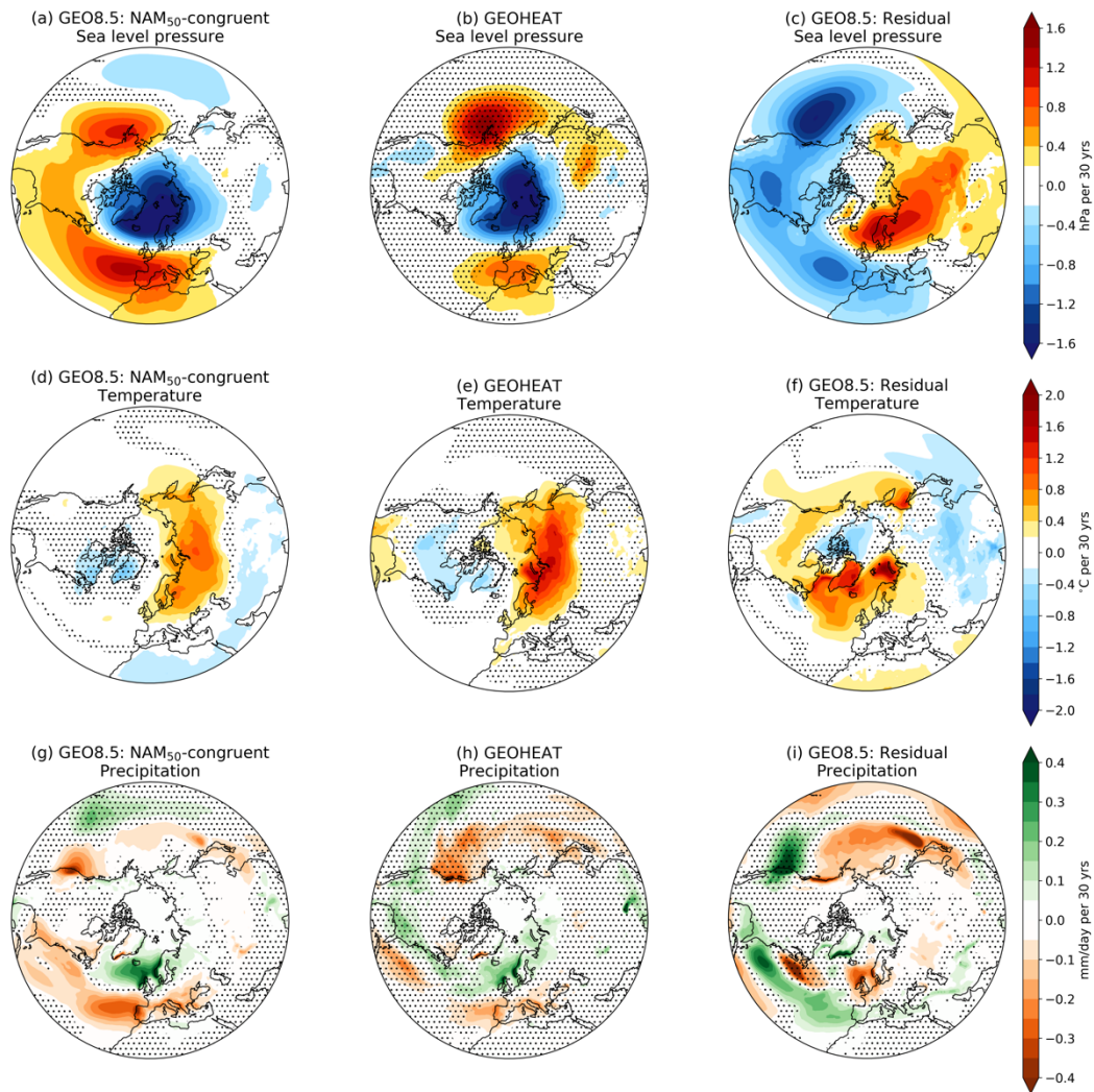
545 Figure 6. Results from regressions of DJF surface climate responses against the stratospheric NAM in GEO8.5, and the responses in GEOHEAT. Ensemble mean linear trends in (a, b, c) sea level pressure (hPa per 30 yrs), (d, e, f) near-surface air temperature (°C per 30 yrs) and (g, h, i) precipitation (mm/day per 30 yrs). Shown are trends in GEO8.5 that are congruent with NAM 50 (first column), equivalent trends in GEOHEAT (second column), and the difference between total GEO8.5 trends and NAM 50 -congruent trends (third column). In the second column, s Stippling indicates lack of statistical significance at the 95% confidence interval under a one sample, two-sided Student's t -test using the standard deviation across ensemble members.
