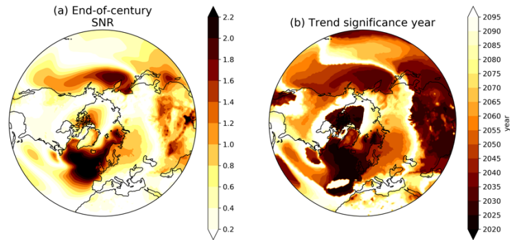
515 Figure 2. Significance of the DJF near-surface air temperature response under geoengineering. (a) The signal to noise ratio of the end-of-century ensemble mean response in GEO8.5 (2075-2095) relative to Base (2010-2030). (b) The endpoint year at which GEO8.5 ensemble mean trends beginning in 2020 become statistically significant from zero, and remain significant, at the 95% confidence level.
