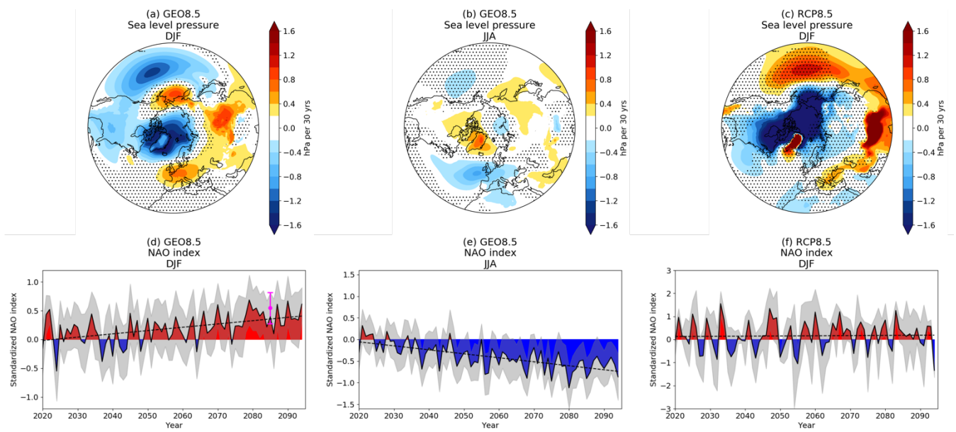
535 Figure 5. Trends in SLP and the surface (SLP-based) NAO timeseries. (a, b, c) Ensemble mean linear trends in sea level pressure (hPa per 30 yrs). (d, e, f) Ensemble mean timeseries of the NAO. Responses are shown for GEO8.5, DJF (first column), GEO8.5, JJA (second column) and RCP8.5, DJF (third column). The magenta point in (d) shows the ensemble mean response in GEOHEAT and its 95% confidence interval. Stippling in (a, b, c) indicates lack of statistical significance at the 95% confidence interval under a one sample, two-sided Student's t -test using the standard deviation across ensemble members. The grey shading in (d, e, f) indicates the 95% confidence interval ( \pm 2\sigma/\sqrt{N} where N is the number of ensemble members). The vertical scales for the NAO index are different in order to clearly illustrate the respective timeseries and confidence intervals.
