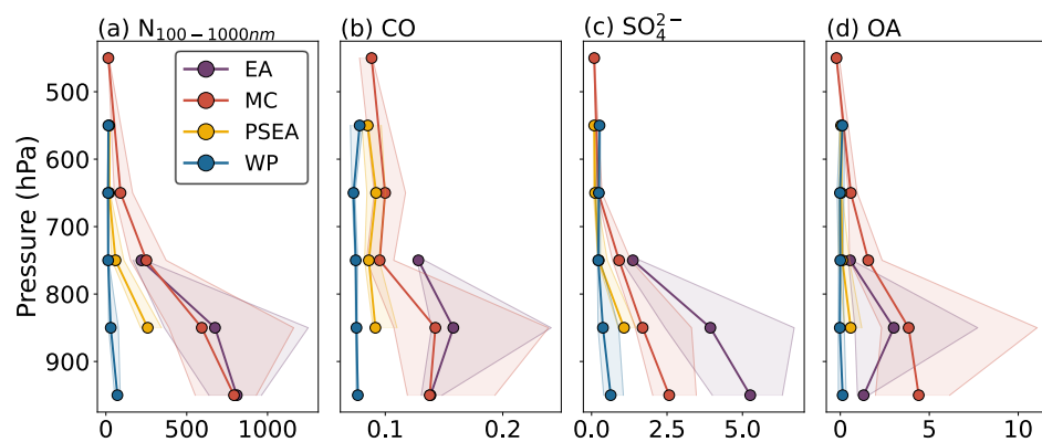
Figure 6: Vertical median profiles of composition for Peninsular Southeast Asia (PSEA), Maritime Continent (MC), East Asia (EA), and West Pacific (WP). (a) N_{100-1000nm} ( cm^{-3} ), (b) CO (ppm), (c) SO_4^{2-} ( \mu g m^{-3} ), (d) OA ( \mu g m^{-3} ). Left and right sides of shaded areas refer to 25th and 75th percentiles, respectively.
