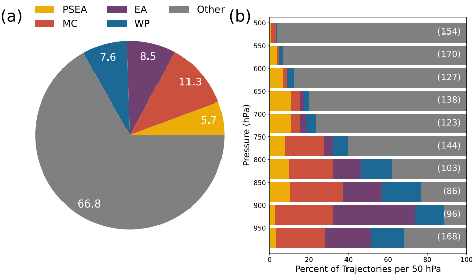
1368 Figure 4: Relative contributions (in percentages) of air masses arriving from study regions (a) averaged over all altitudes 1369 and (b) pressure levels (hPa). Total number of trajectories per pressure bin is provided on the right end of (b). Source 1370 regions are Peninsular Southeast Asia (PSEA), Maritime Continent (MC), East Asia (EA), and West Pacific (WP). 1371
