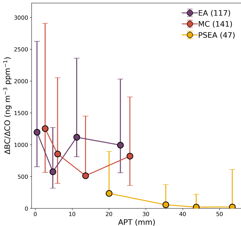
Figure 9: (a) \Delta BC/\Delta CO ratio ( \Delta CO > 0.02 ppm) as a function of accumulated precipitation along individual trajectories (APT) resolved by source region. APT was calculated with PERSIANN-CDR, and (b) histograms of \Delta BC/\Delta CO resolved by wet ( APT > 10 mm) and dry ( APT < 10 mm) air masses. Medians and 25 th /75 th percentiles (error bars) are shown for (a) each source region: Peninsular Southeast Asia (PSEA), Maritime Continent (MC), and East Asia (EA). West Pacific (WP) was not plotted because of few data points where \Delta CO > 0.02 ppm. Black line in (a) represents the trend for all source-classified data (EA, MC, PSEA, WP) grouped into APT bins. Number of observations plotted per source region are provided in parentheses in (a).
