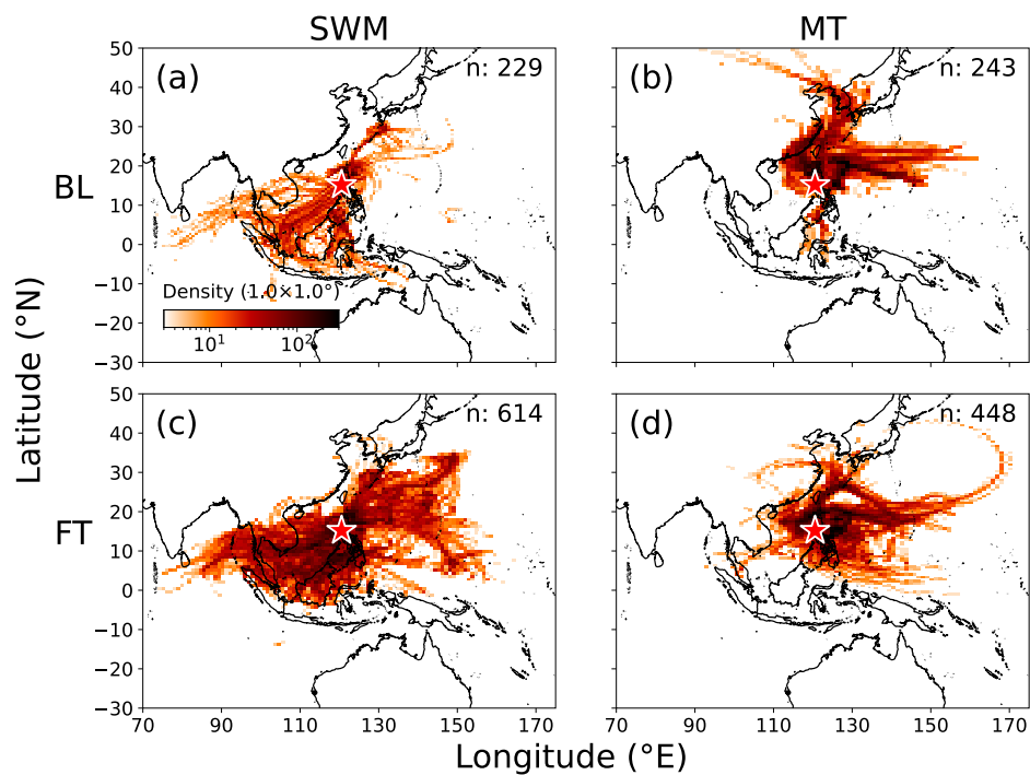
Figure 2: Trajectory densities resolved by monsoon phase and sampling vertical level. Monsoon phases are southwest monsoon (SWM; before 20 Sep 2019) and the monsoon transition (MT; after 20 Sep 2019). Vertical sampling levels are divided into boundary layer (BL; < 2 km) and free troposphere (FT; > 2 km). Red star denotes Clark International Airport, Philippines. Number of trajectories (n) is shown in the upper right of each panel.
