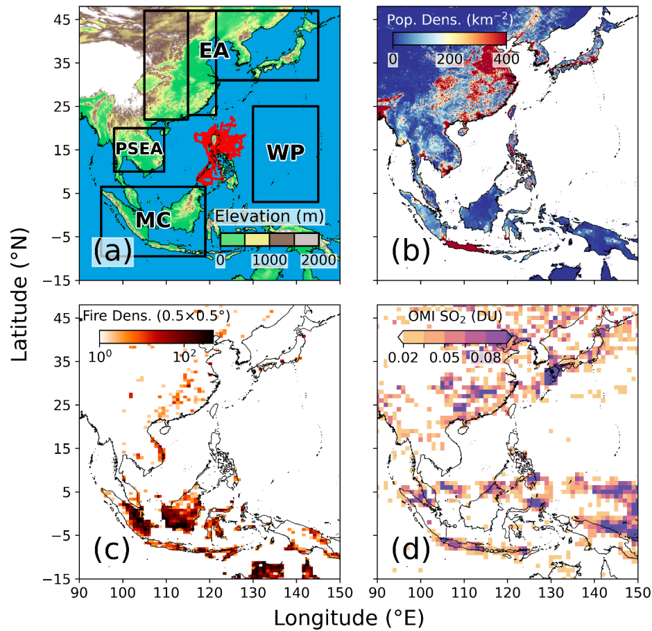
1350 Figure 1: Maps of (a) ground elevation from the Global Multi-resolution Terrain Elevation Data 2010 (GMTED2010), flight 1351 tracks in red, and approximate source regions in labeled boxes: Peninsular Southeast Asia (PSEA), Maritime Continent 1352 (MC), East Asia (EA), and West Pacific (WP), (b) 2020 population density from the Center for International Earth Science 1353 Information Network (CIESIN) Gridded Population of the World (GPW) v4, (c) MODIS active fire hotspot density (only 1354 fires tagged with > 80% confidence) averaged at 0.5° × 0.5° resolution from 1 Aug to 15 Oct 2019, and (d) OMI-retrieved 1355 PBL SO 2 averaged over the same period.
