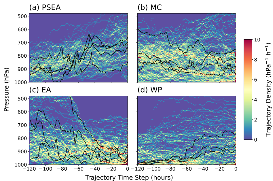
Figure 5: Vertical motion during transport from (a) Peninsular Southeast Asia (PSEA), (b) Maritime Continent (MC), (c) East Asia (EA), and (d) West Pacific (WP). Color corresponds to density as a function of trajectory altitude (pressure) and time step. Example trajectories are plotted in black to show actual vertical motion.
