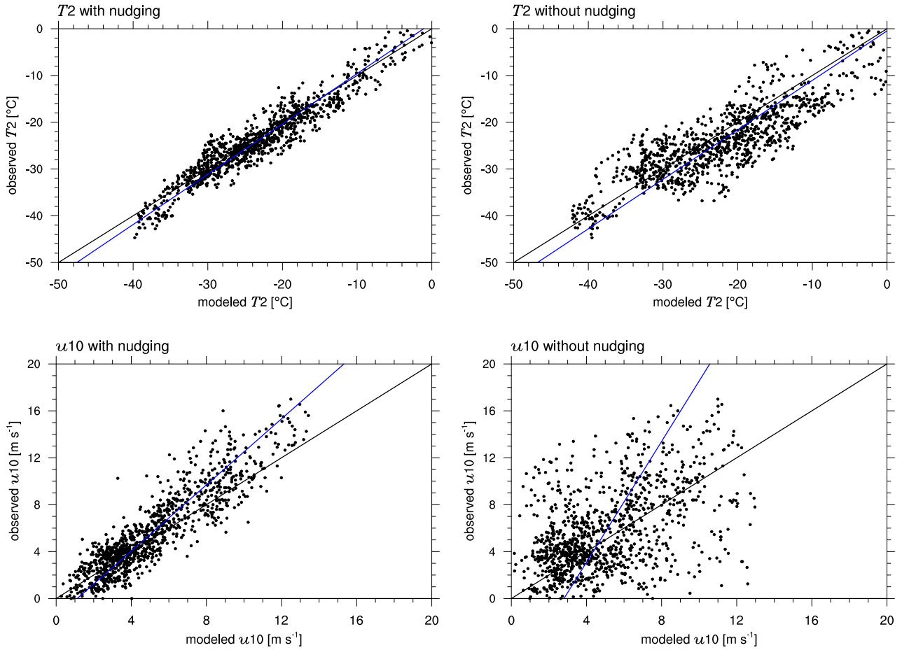
Figure 3. Correlation of observed and modeled temperature and wind speed at Utqiagvik for the complete time range from February 1, 2009 through May 1, 2009. The black and blue lines show perfect agreement and the regression line of the simulation and the observation, respectively.
