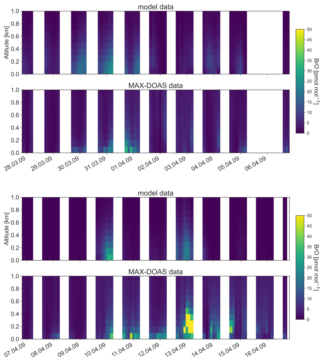
Figure 10. Vertical profiles of BrO from March 28, 2009 to April 16, 2009 at Utqiagvik. The date shown is for 00:00, GMT-9 (local time at Utqiagvik). Top: Modeled BrO convoluted with the MAX-DOAS averaging kernel, Bottom: BrO observed with MAX-DOAS
