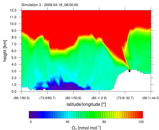
Figure 6. Ozone mixing ratio obtained from simulation 3 ( \beta = 1.5 ) against height along a horizontal line through Summit, cf. Fig. 1. A tropopause fold reaches Summit (♦). The time zone is GMT+0.
