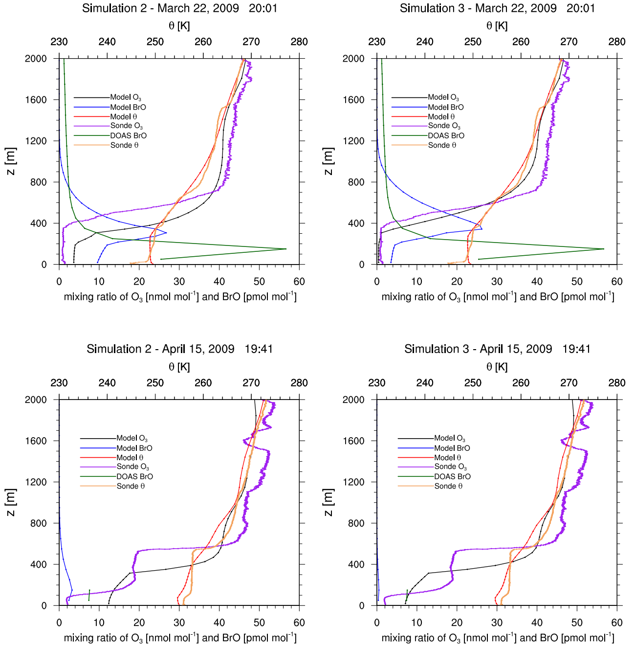
Figure 9. Vertical profiles of measured and modeled (simulation 2 (left) and simulation 3 (right)) ozone, of potential temperature \theta , and of BrO at Utqiagvik on March 22 (top) and April 15 (bottom), 2009. The time zone is GMT+0. Measurements are from upward flights using ozone sondes (Oltmans et al., 2012) and DOAS measurements (Frieß et al., 2011). On April 15, only the observed BrO mixing ratio in the lowest 100 m is accurate due to very poor visibility.
