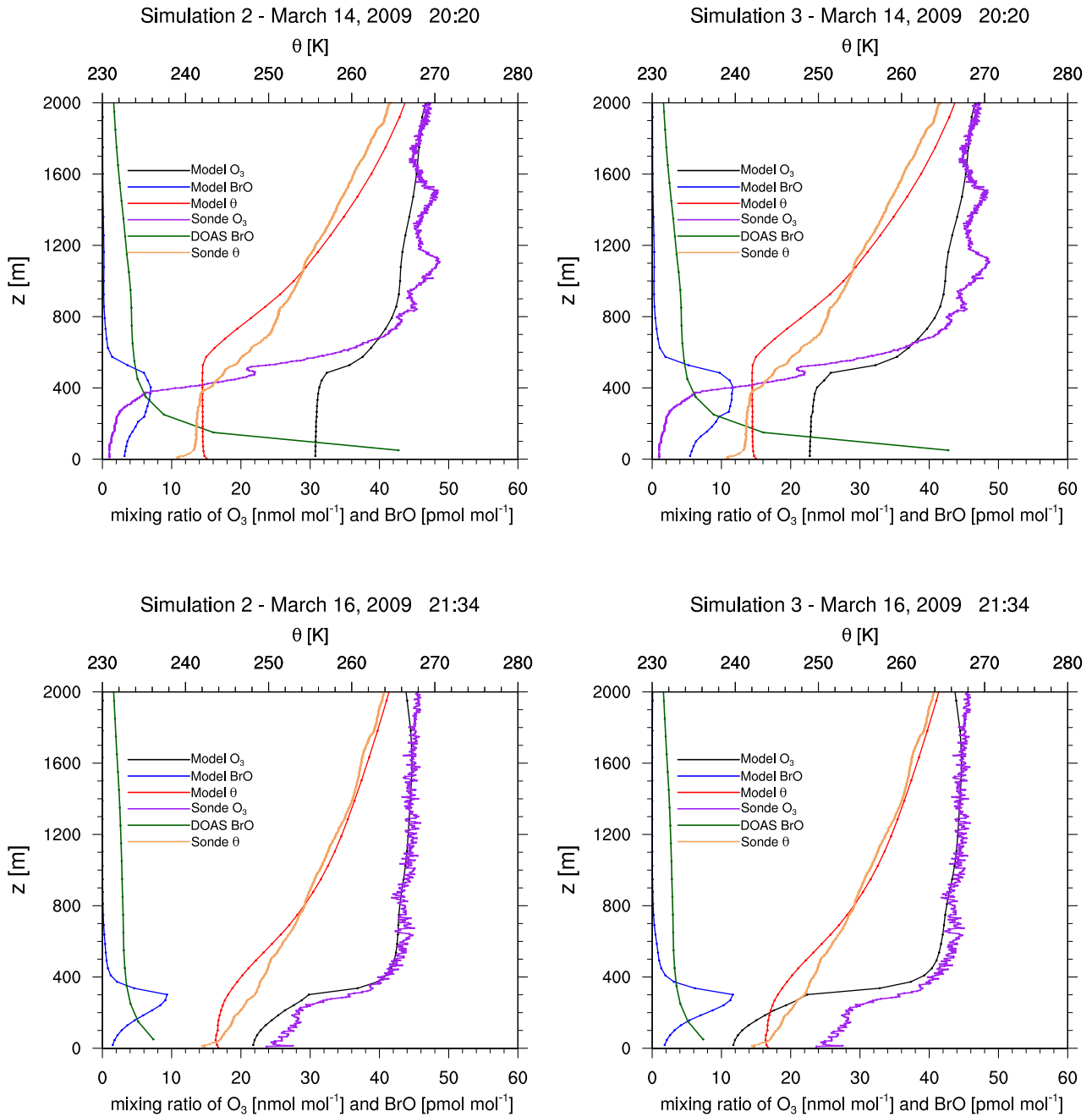
Figure 8. Vertical profiles of measured and modeled ozone, of potential temperature \theta , and of BrO at Utqiagvik on March 14 (top) and on March 16 (bottom), 2009. The time zone is GMT+0. Measurements are from upward flights using ozone sondes (Oltmans et al., 2012) and DOAS measurements (Frieß et al., 2011).
