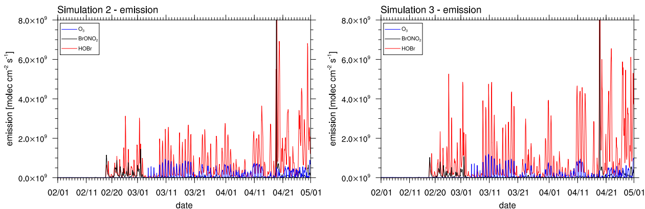
Figure 16. Emission rate of \text{Br}_2 due to HOBr and \text{BrONO}_2 and due to bromide oxidation by ozone from the snow surface at coordinates 178 W, 78 N for simulations 2 with \beta = 1 (left) and simulation 3 with \beta = 1.5 (right). The date shown is for 06:00, GMT+0.
