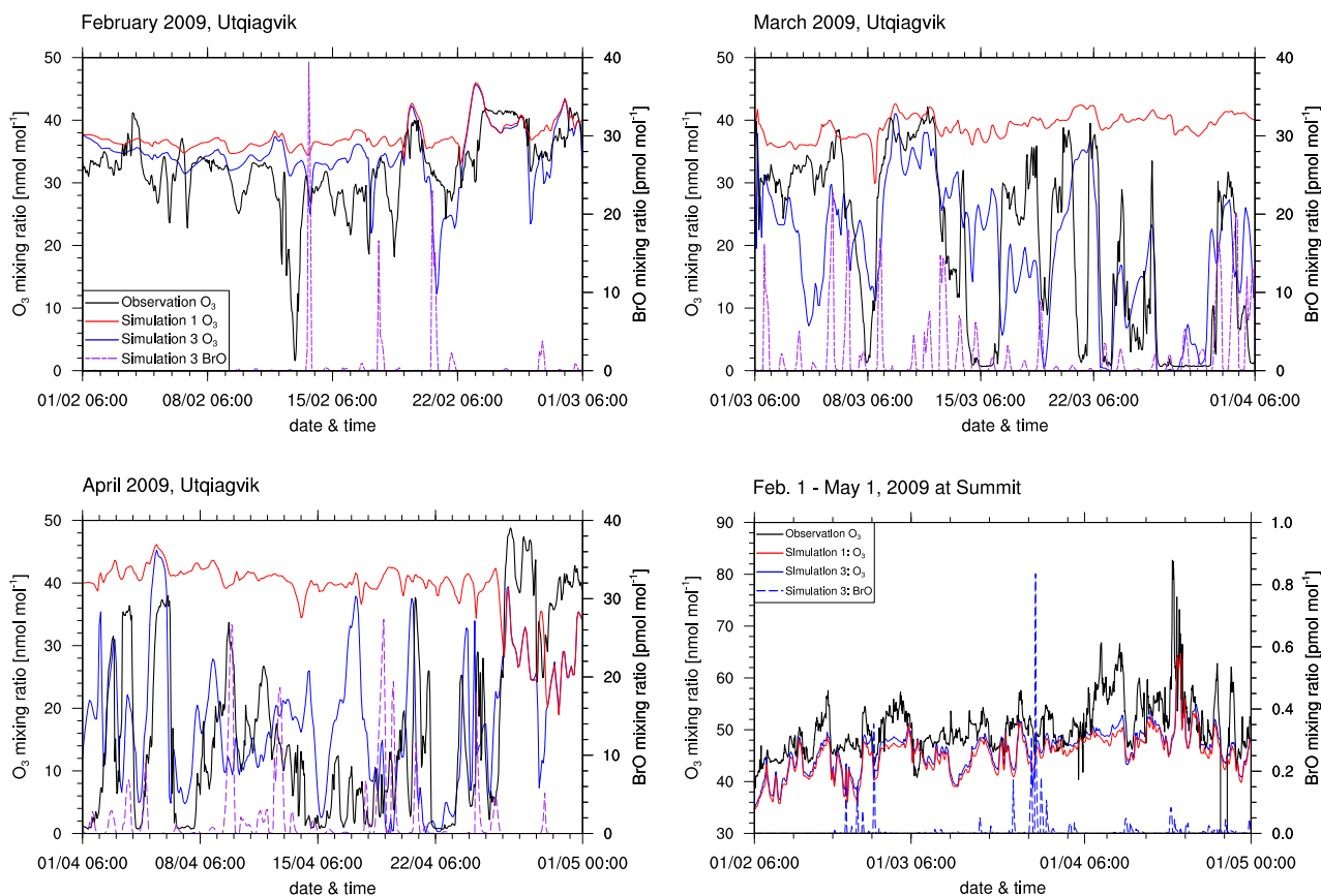
Figure 4. Ozone at Utqiagvik and at Summit from observations and simulations 1 (no halogens) and 3 (increased emissions, \beta = 1.5 ). Modeled BrO mixing ratios are also shown. The figures share the legend.
