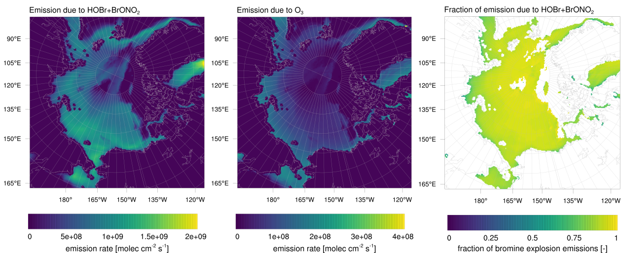
Figure 15. Emission rate of \text{Br}_2 due to \text{HOBr} + \text{BrONO}_2 (left) and due to bromide oxidation by ozone (center) from the snow surface for simulation 3, averaged over the complete simulation period. Ratio of \text{Br}_2 emissions due to \text{HOBr} and \text{BrONO}_2 to total \text{Br}_2 emissions on FY ice (right).
