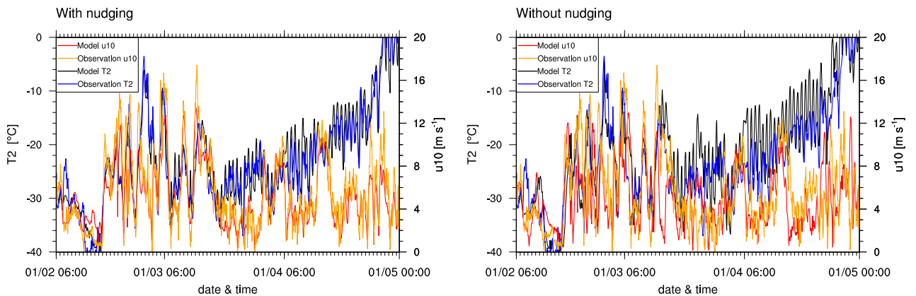
Figure 2. 2 m temperature and 10 m wind speed at Utqiagvik in February through May 2009. Measurements are taken from the Barrow Atmospheric Baseline Observatory (Mefford et al., 1994).
