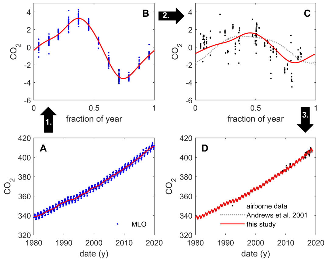
725 Figure 2. Illustration of the major steps in deriving a tropical upper tropospheric reference time series. Panel (a) shows the monthly mean surface CO 2 concentrations at Mauna Loa (MLO) (Keeling et al., 2001) with a stiff spline trend shown in red. Panel (b) shows a fit of the mean seasonal cycle at MLO compared to detrended observations from 1980–2019. Panel (c) shows the 1-month-lagged seasonal cycle (red line) rescaled in amplitude to match detrended airborne observations in the equatorial upper troposphere (20°S < lat < 20°N, alt >8 km, black). The seasonal cycle derived by Andrews et al. (2001) is presented as a dotted grey line for reference. 730 Panel (d) shows the resulting upper tropospheric mean reference time series (TRTS, red) used for CO 2 in the age of air algorithm with the airborne observations from the tropical upper troposphere (black dots) and the time series (grey dotted line) of Andrews et al. (2001).
